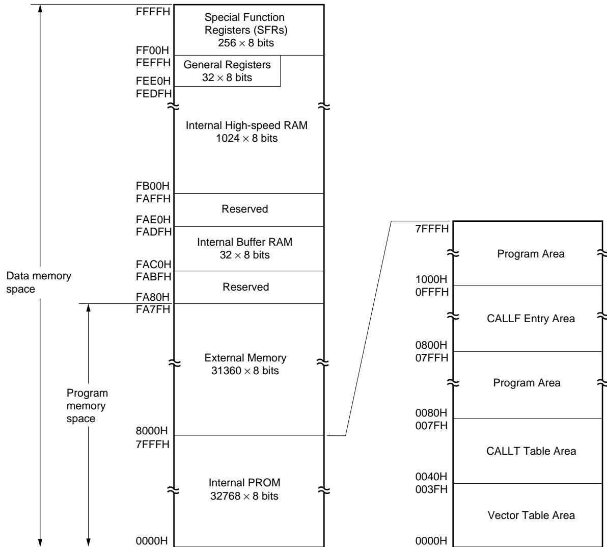
Figure 5-4. Memory Map ( \mu PD78P054)
