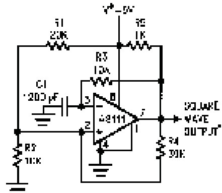
FIGURE 4. Free Running Multivibrator
