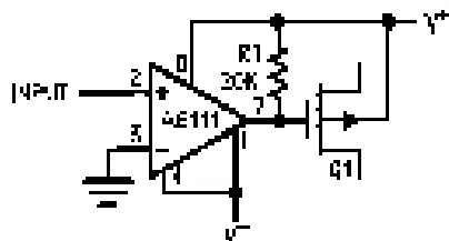
Zero Crossing Detector Driving MOS Switch
