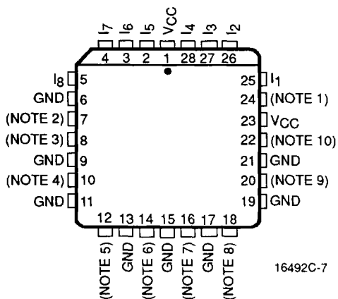
28-Pin PLCC
