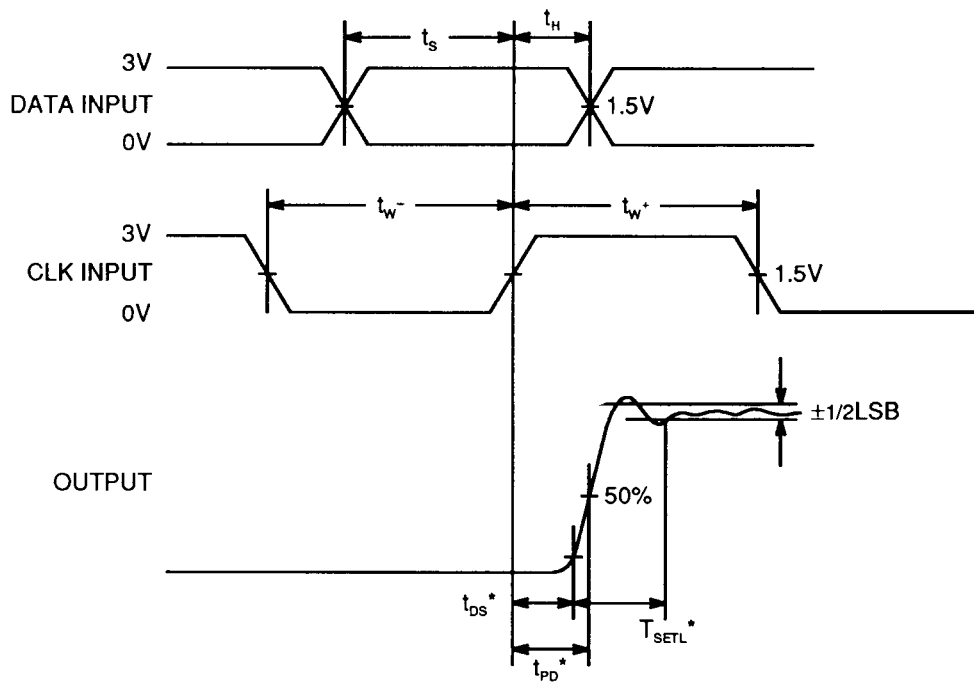
Fig. 2 – TIMING DIAGRAM
