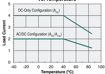
Maximum Load Current vs. Temperature
