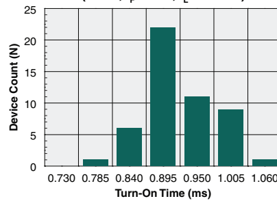
Typical Turn-On Time Distribution (N=50, I_F=5\text{mA} , I_L=120\text{mA} )
