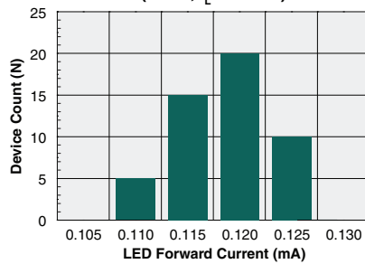
Typical I_F for Switch Operation (N=50, I_L=500\text{mA} )
