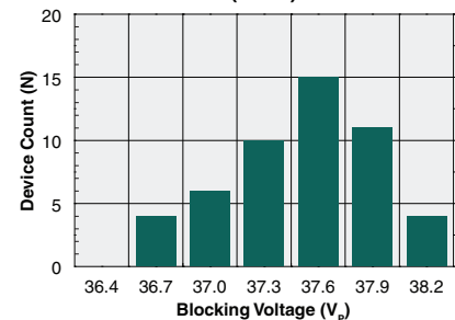
Blocking Voltage Distribution (N=50)
