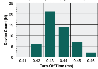
Typical Turn-Off Time Distribution (N=50, I_F=5\text{mA} , I_L=120\text{mA} )
