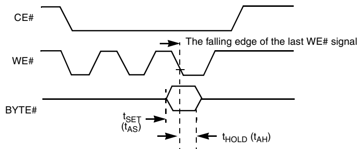
Figure 13. BYTE# Timings for Write Operations
