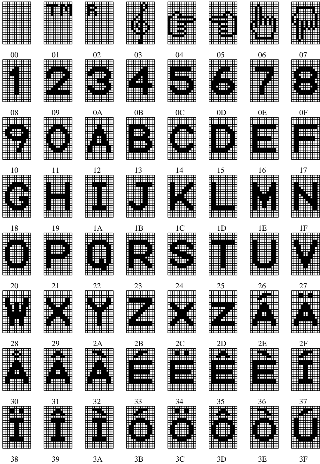
Figure 17. ROM 00 - 3F
