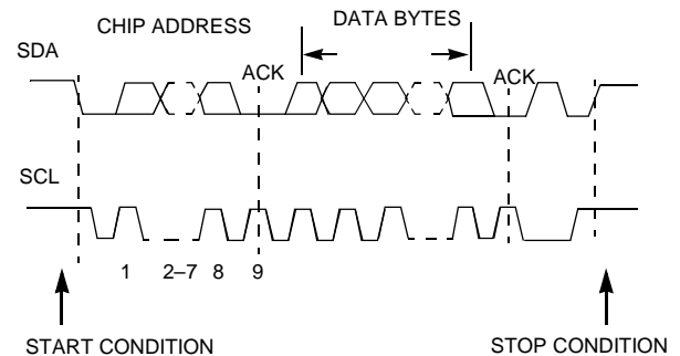
Figure 2. M_BUS Format
