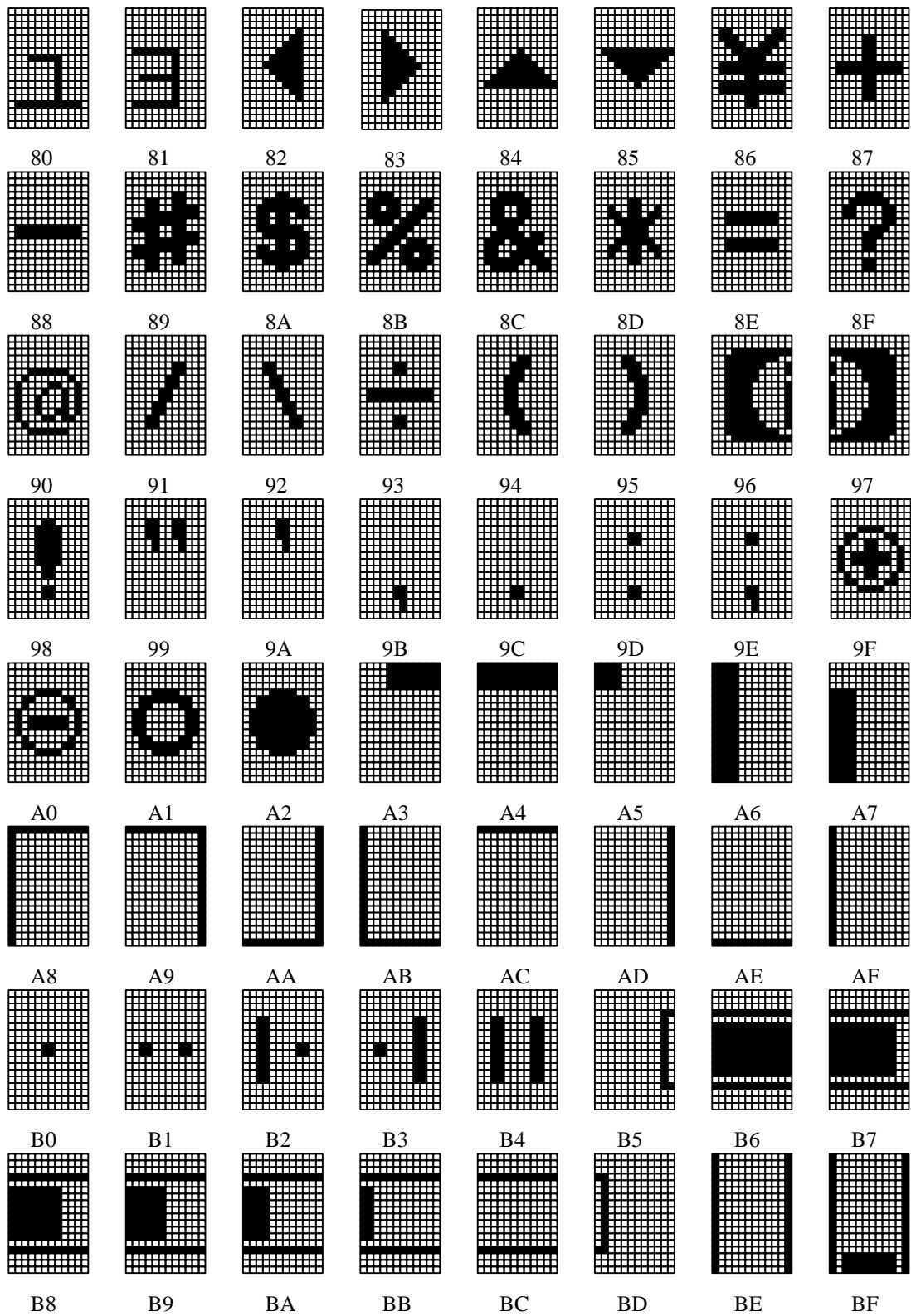
Figure 19. ROM 80 - BF
