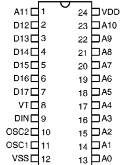
HT646L – 24 SOP/SDIP
