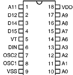
HT683L – 18 DIP
