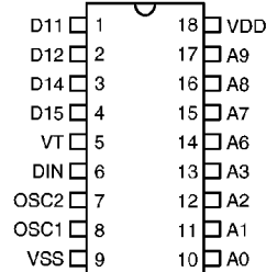
HT684L – 18 DIP
