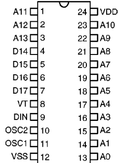
HT644L – 24 SOP/SDIP
