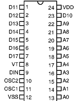
HT648L – 24 SOP/SDIP
