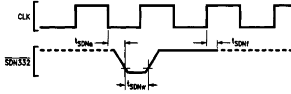
FIGURE 4-13. SDRAM332 Timing (NS32332 CPU)
