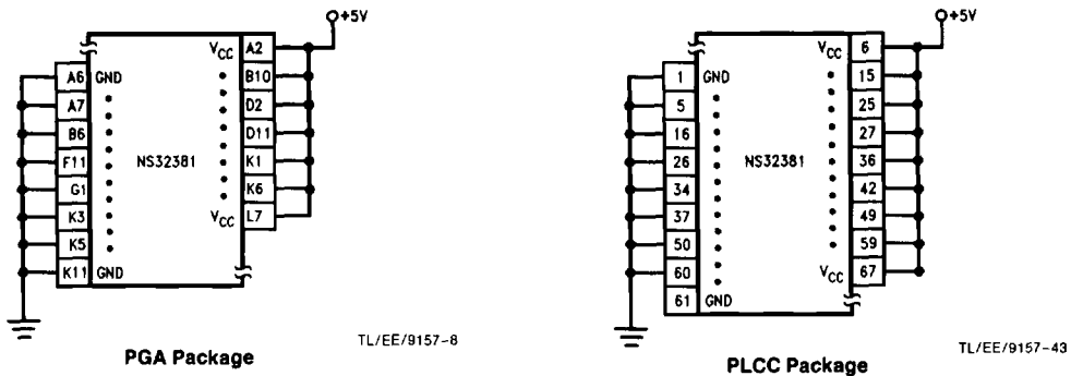
FIGURE 3-1. Recommended Supply Connections
