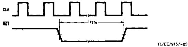
FIGURE 4-7. Non-Power-On Reset
