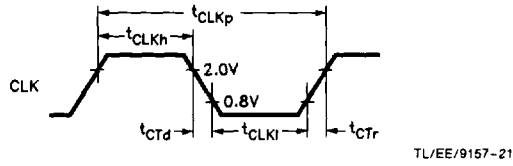
FIGURE 4-5. Clock Timing
