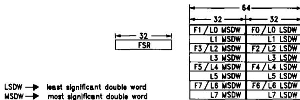
FIGURE 2-1. Register Set
