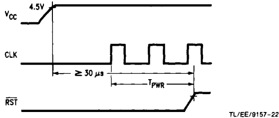
FIGURE 4-6. Power-On Reset
