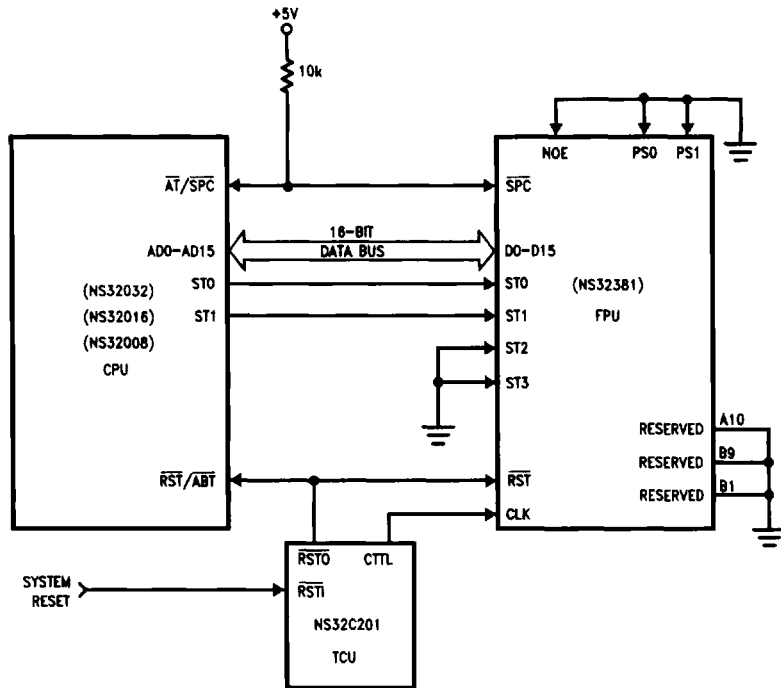
FIGURE 3-4c. System Connection Diagram with the NS32008, NS32016 or NS32032 CPU
