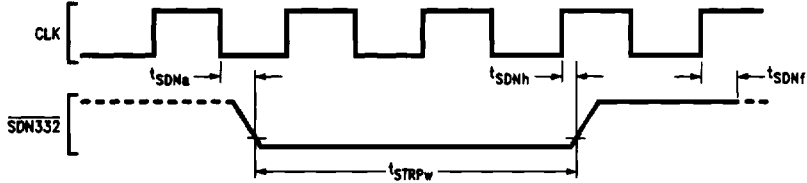
FIGURE 4-14. SDRAM332 (TRAP) Timing (NS32332 CPU)
