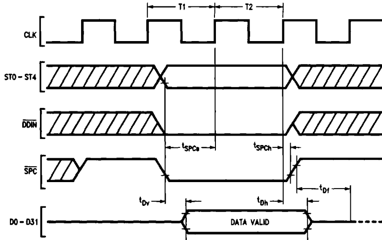
FIGURE 4-15. Read Cycle from FPU (NS32532 CPU)
