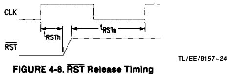
FIGURE 4-8. \overline{RST} Release Timing
