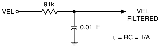
FIGURE 17. VEL OUTPUT FILTER
