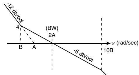
FIGURE 19. OPEN LOOP BODE PLOT
