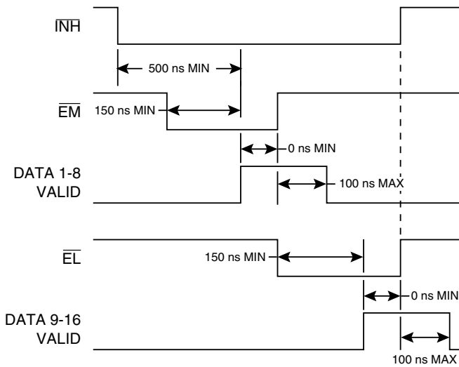
FIGURE 14. 8-BIT DATA TRANSFER TIMING
