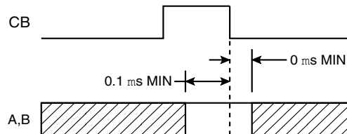
FIGURE 2. RESOLUTION CONTROL TIMING DIAGRAM
