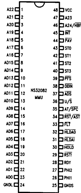
Top View
