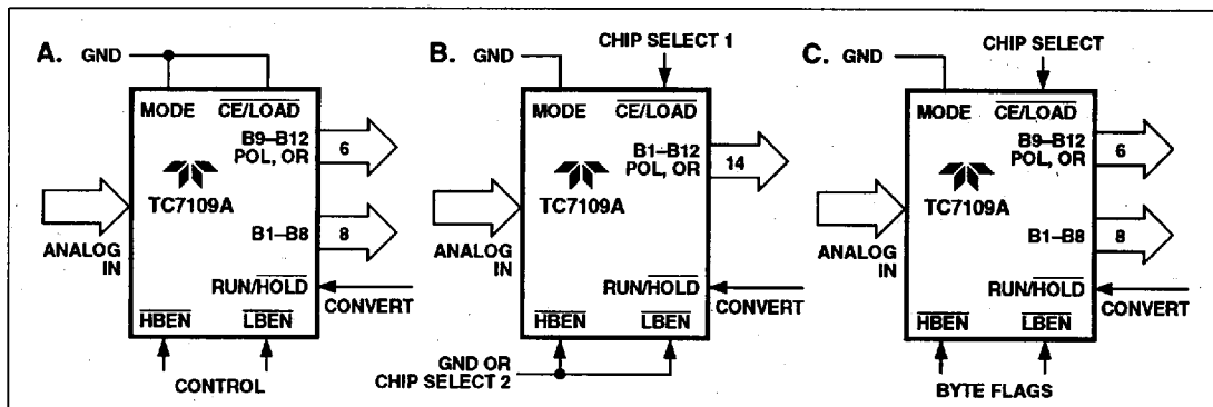
Figure 12 Direct Mode Chip and Byte Enable Combinations
