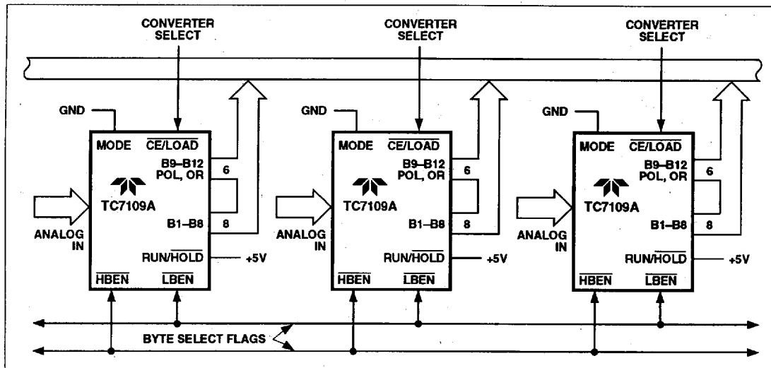
Figure 13 Three-Stating Several TC7109A's to a Small Bus
