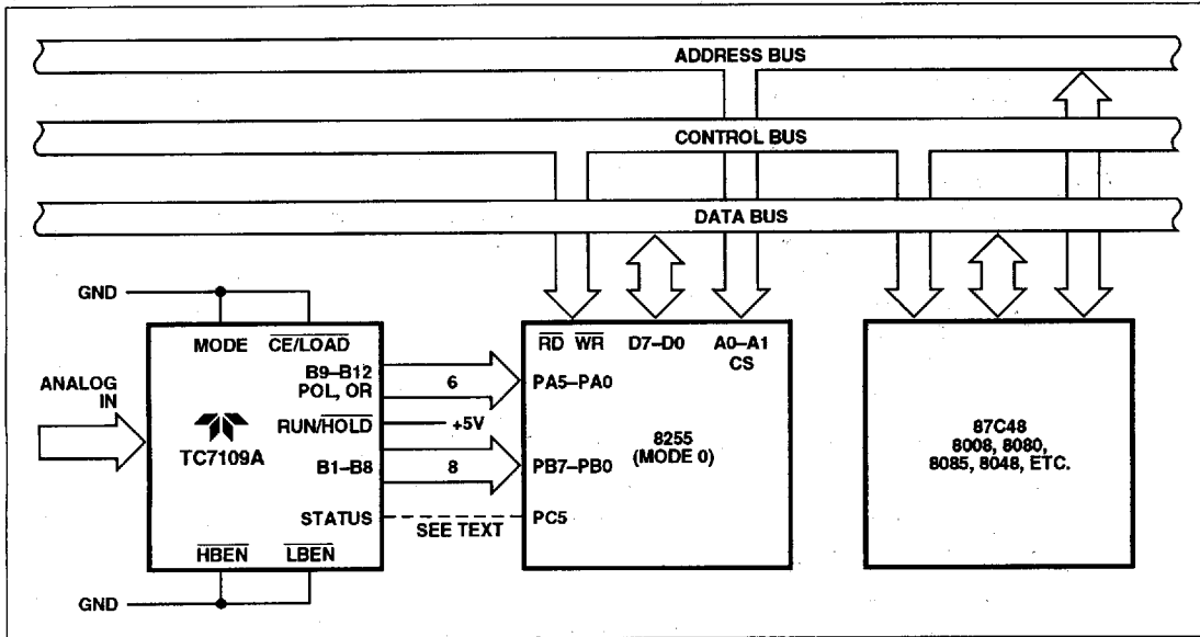
Figure 14 Full-Time Parallel Interface to MCS-48, -80, -85 Microcomputers
