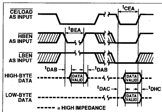
Figure 6 TC7109A Direct Mode Output Timing
