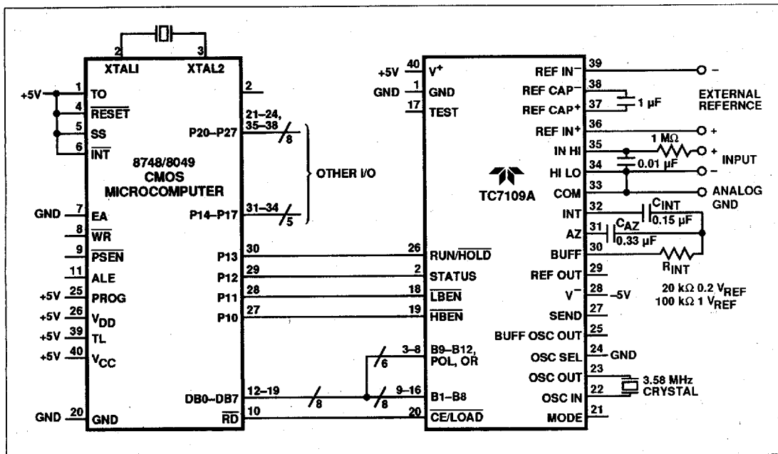
Figure 2 TC7109A Parallel Interface With 8048/8049 Microcomputer
