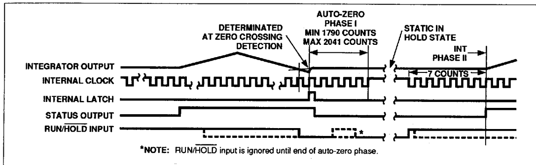
Figure 5 TC7109A RUN/HOLD Operation
