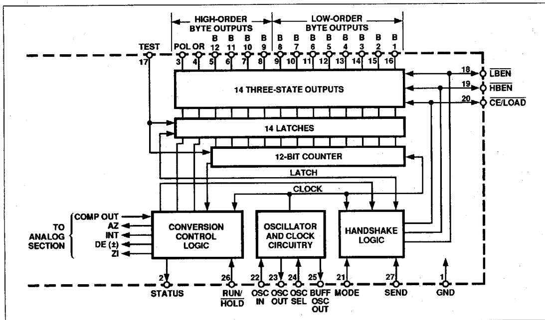
Figure 4 Digital Section
