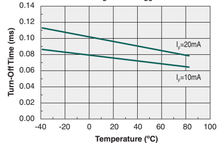
Typical Turn-Off Time vs. Temperature ( I_L=100\text{mA}_{DC} )
