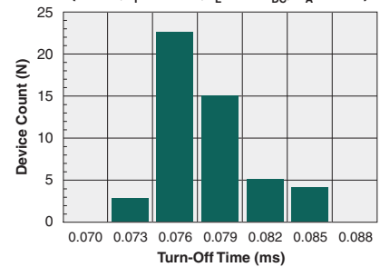
Typical Turn-Off Time (N=50, I_F=10\text{mA} , I_L=5\text{mA}_{DC} , T_A=25^\circ\text{C} )
