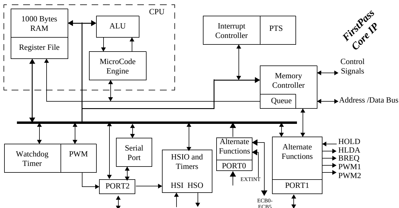
Figure 1. UT80CRH196KDS Microcontroller
