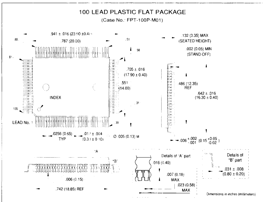
FPT-100P-M01
