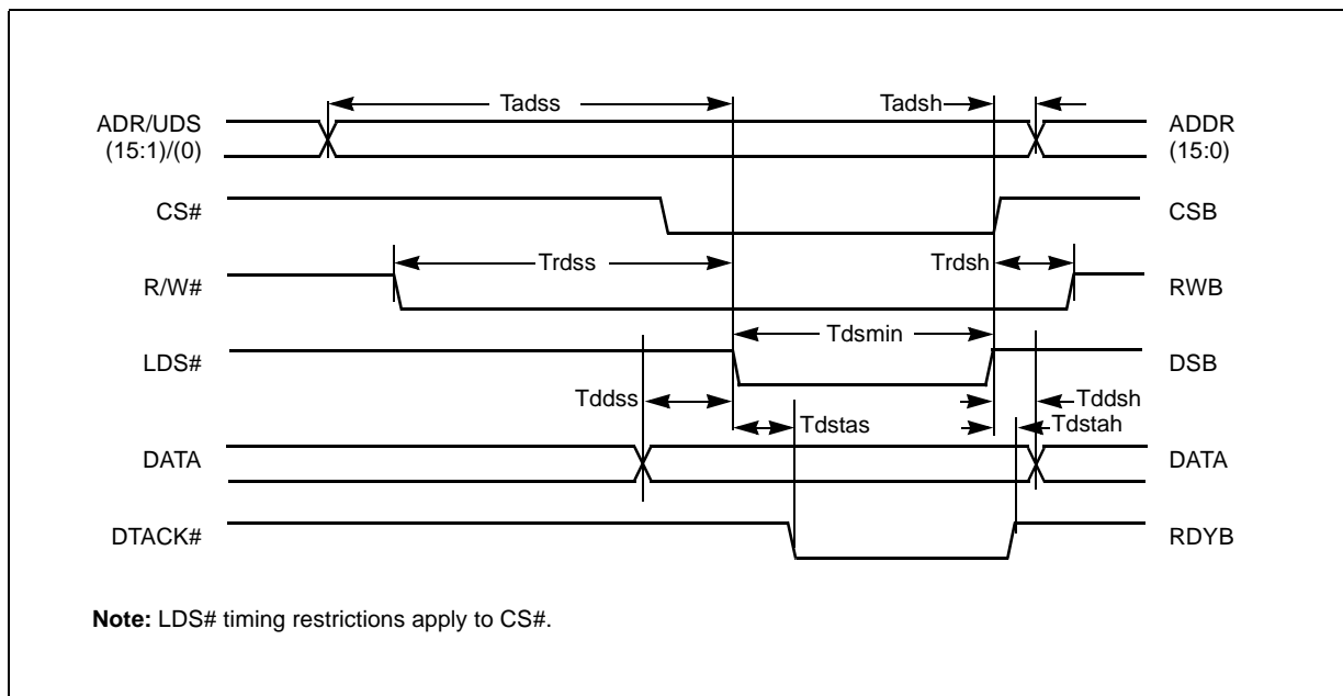
Figure 53 Motorola* M68302 Processor - Write Timing
