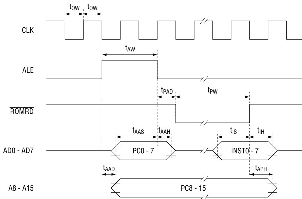
Figure 7. ROM Read Timing
