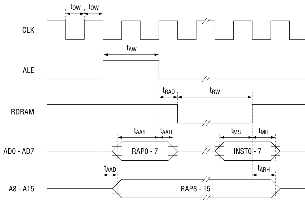
Figure 8. RAM Read Timing
