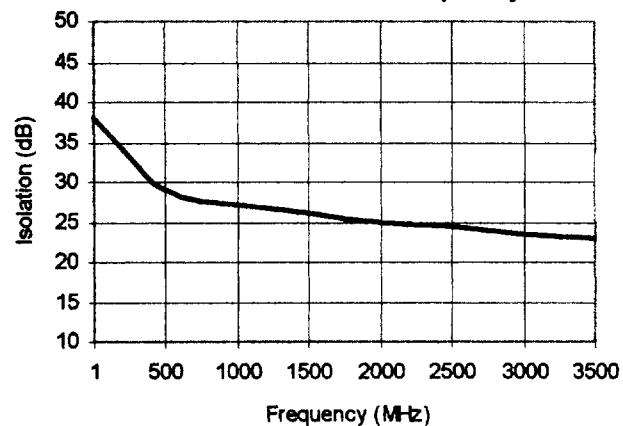
LO/IF Isolation vs Frequency
