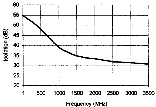
LO/RF Isolation vs Frequency
