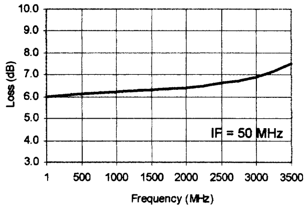
Loss vs Frequency
