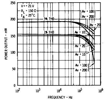
POWER OUTPUT AS A FUNCTION OF FREQUENCY OF FREQUENCY 5% AND 1% TOTAL HARMONIC DISTORTION
