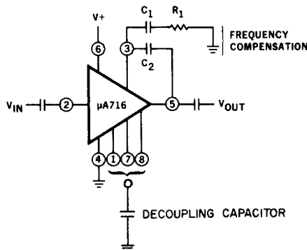
CONNECTION DIAGRAM AND COMPONENT TABLE FOR AVAILABLE GAIN OPTIONS
