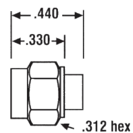
3201-2A-1 SMA Straight Male Semi-Rigid/Ultra-Flex-Solder RG405 .085SR (Gold)
