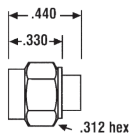
3201-2A-9 SMA Straight Male Semi-Rigid/Ultra-Flex-Solder RG405 .085SR (Passivated)
