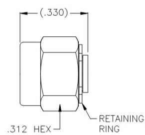
3133-9 SMA Straight Male Semi-Rigid/Ultra-Flex-Solder .047 SR (Passivated)
