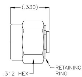
3183P-3-9 SMA Straight Male Semi-Rigid/Ultra-Flex-Solder RG405 .085SR (Passivated)
