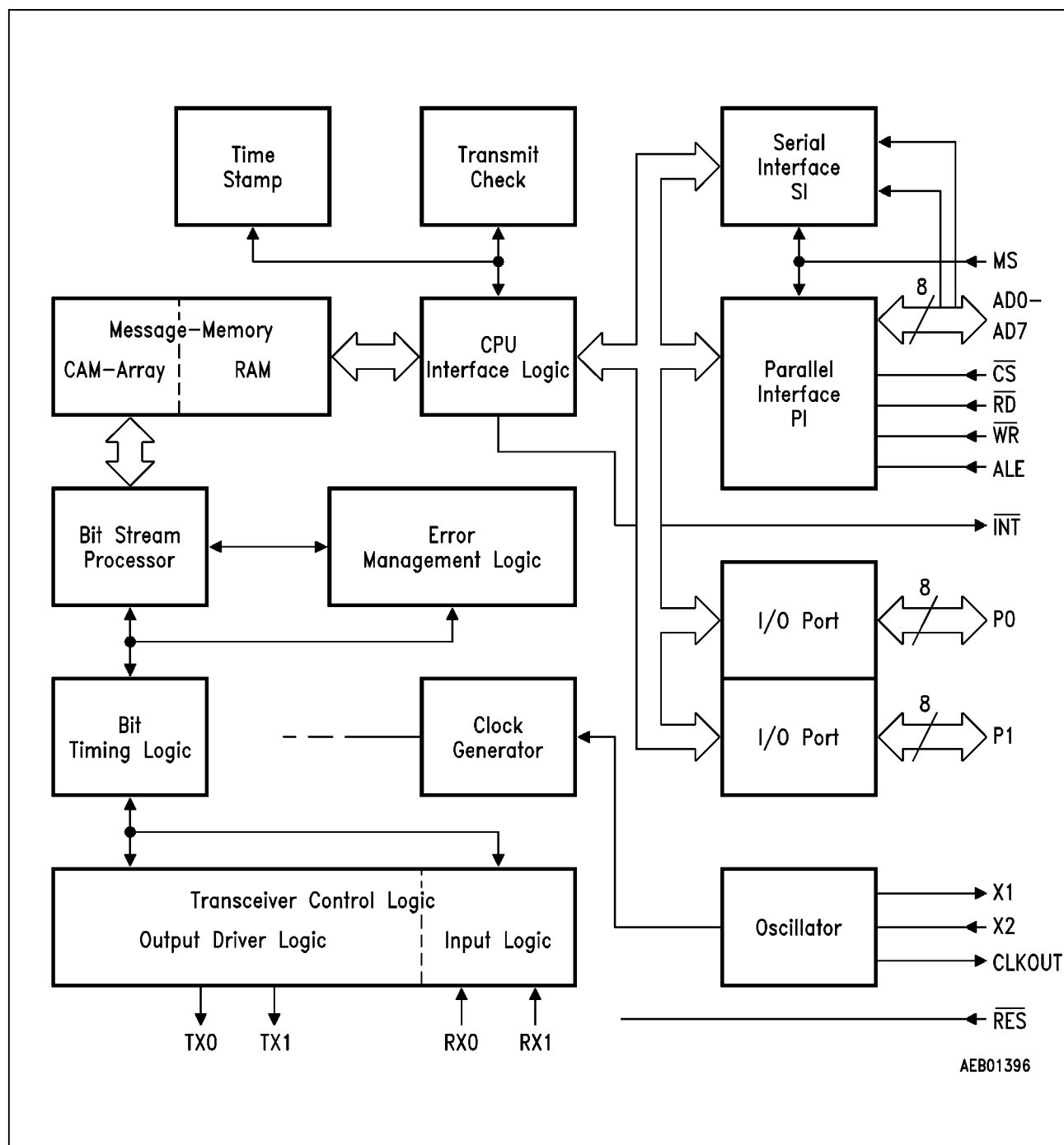
Figure 3 Block Diagram
