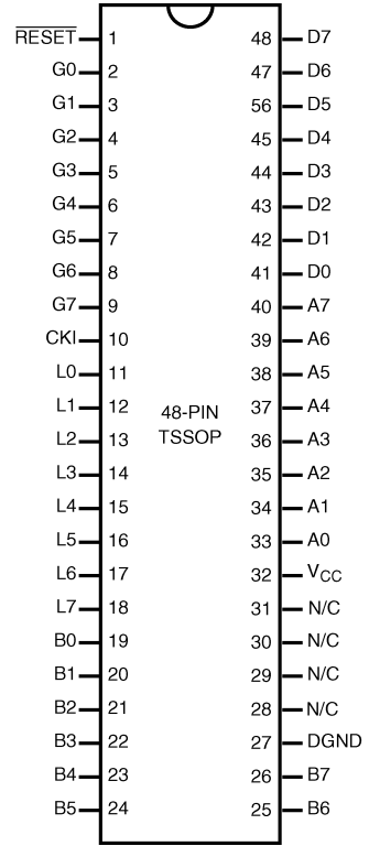
20032759 Top View TSSOP Package See NS Package Number MTD48
