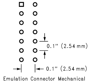
FIGURE 6. Emulation Connection
