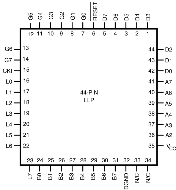
20032755 Top View LLP Package See NS Package Number LQA44A
