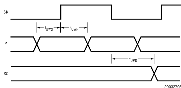
FIGURE 1. MICROWIRE/PLUS Timing
