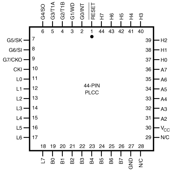
20032764 Top View Plastic Chip Package See NS Package Number V44A
