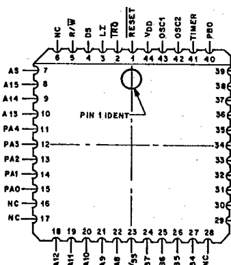
CDP6805E3 44 PLCC TOP VIEW
