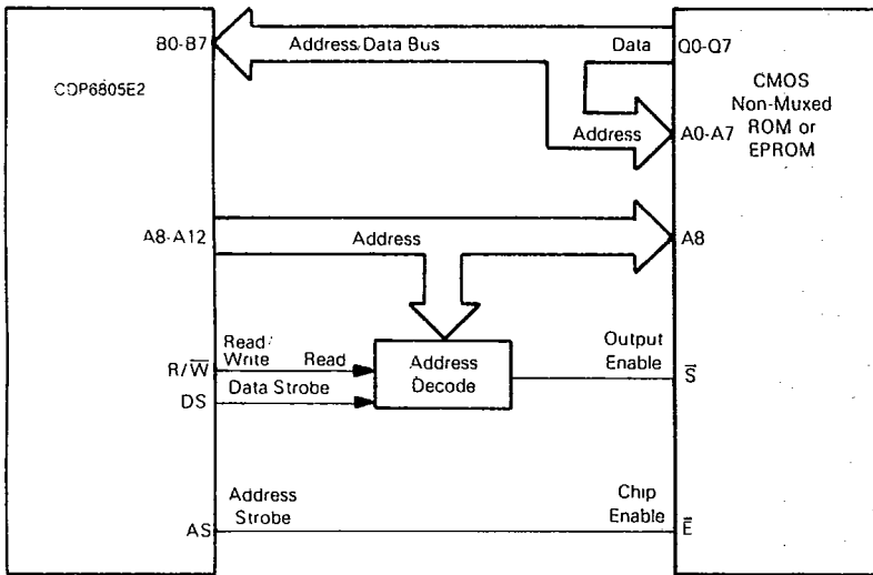
Fig. 22 - Connection to latch non-multiplexed CMOS ROM or EPROM.
