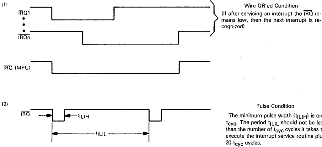
(b) Interrupt Mode Diagram
