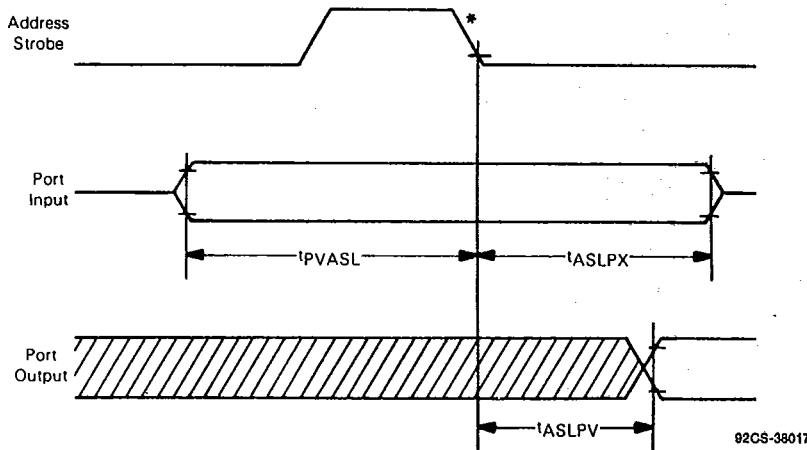
Fig. 3 - I/O port timing waveforms.
