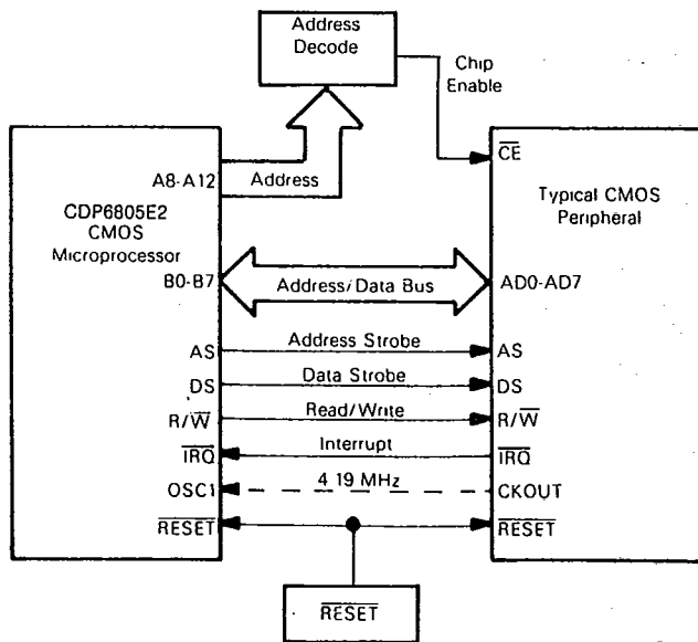
Fig. 20 - Connection to CMOS peripherals.
