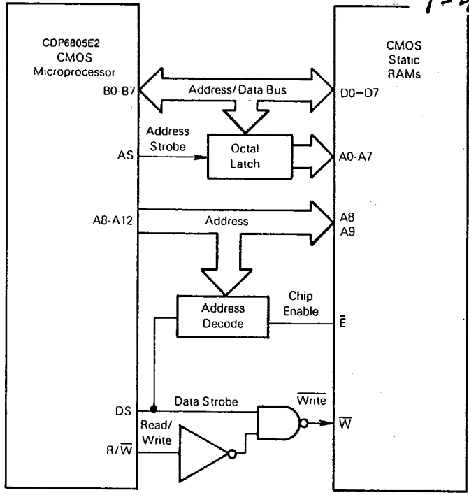
Fig. 23 - Connection to static CMOS RAMs.
