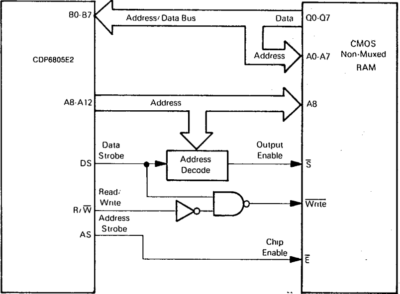
Fig. 24 - Connection to latched non-multiplexed CMOS RAM.
