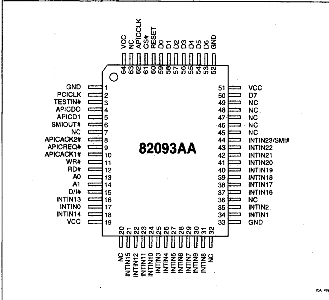
Figure 4. IOAPIC Pinout
