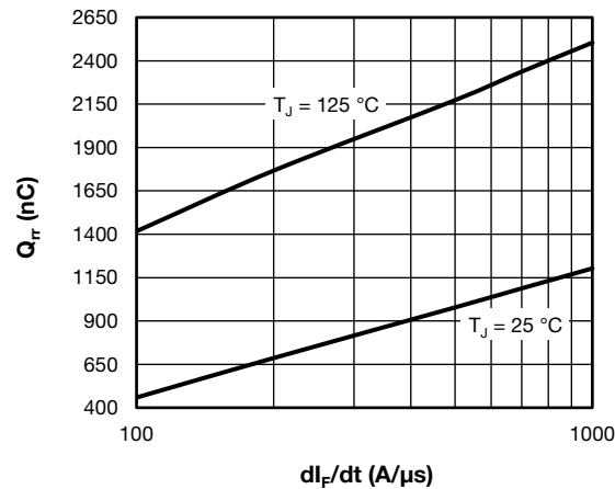
Fig. 17 - Typical Diode Reverse Recovery Charge vs. di_F/dt V_{rr} = 200\text{ V} , I_F = 50\text{ A}
