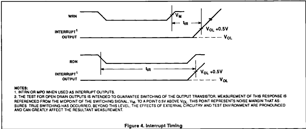
Figure 4. Interrupt Timing
