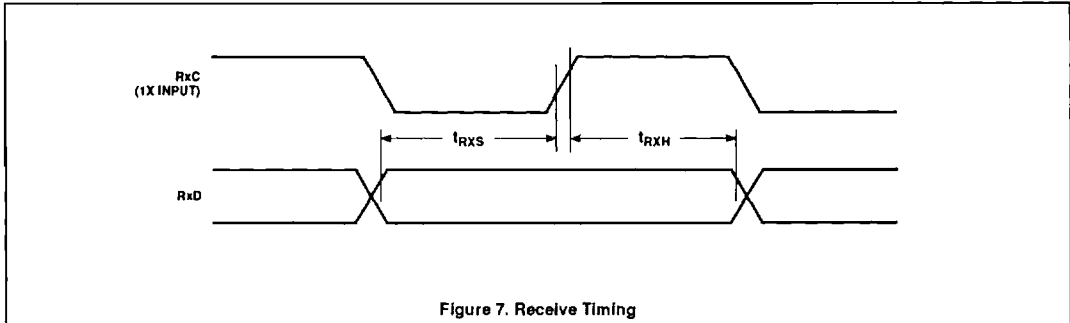
Figure 7. Receive Timing
