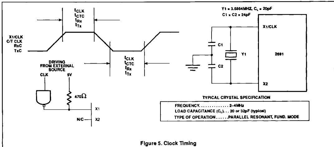
Figure 5. Clock Timing
