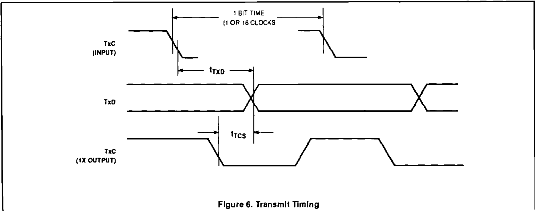
Figure 6. Transmit Timing
