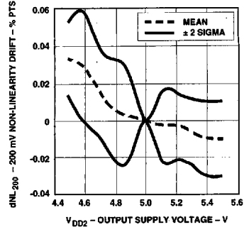
Figure 12. 200 mV Nonlinearity Drift vs. V_{DD2} ( V_{DD1} = 5 V).
