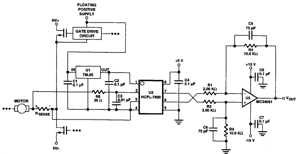
Figure 26. Recommended Application Circuit.
