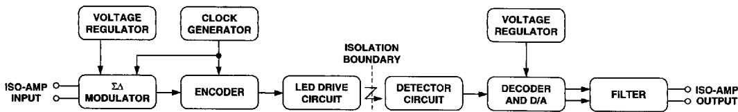
Figure 28. HCPL-7800 Block Diagram.
