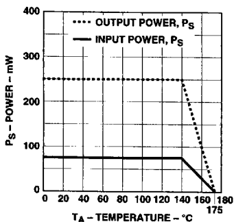
Figure 27. Dependence of Safety-Limiting Parameters on Ambient Temperature.
