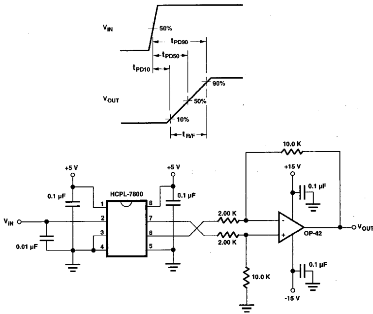
Figure 22. Propagation Delay and Rise/Fall Time Test Circuit.
