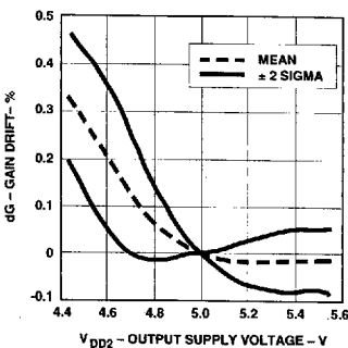
Figure 8. Gain Drift vs. V_{DD2} ( V_{DD1} = 5 V).
