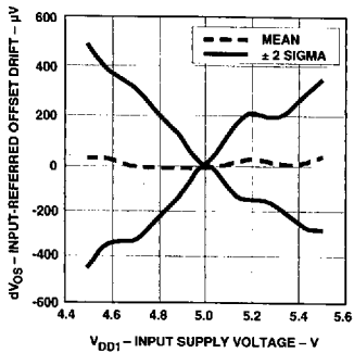
Figure 3. Input-Referred Offset Drift vs. V_{DD1} ( V_{DD2} = 5 V).
