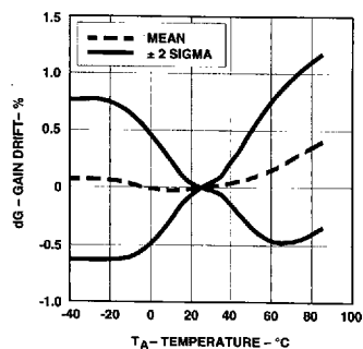
Figure 6. Gain Drift vs. Temperature.
