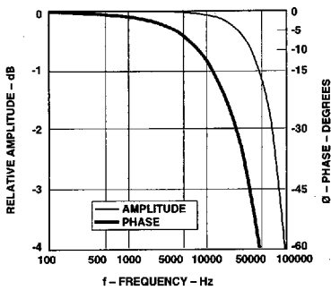
Figure 23. Typical Amplitude and Phase Response vs. Frequency.
