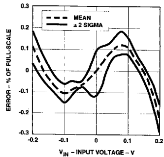
Figure 9. 200 mV Nonlinearity Error Plot.
