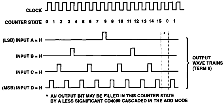
FIGURE 4. TIMING DIAGRAM
