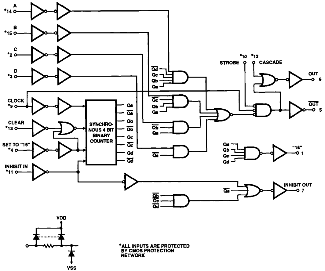
FIGURE 1. LOGIC DIAGRAM
