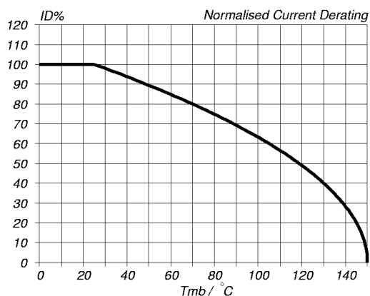
Fig.2. Normalised continuous drain current. ID\% = 100 \cdot I_D / I_{D\ 25^\circ\text{C}} = f(T_{sp}) ; conditions: V_{GS} \geq 5\text{ V}
