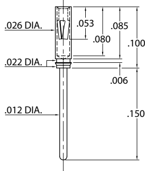
8210-0-15-15-04-27-04-0 Press-fit in .024/.027 stepped hole
