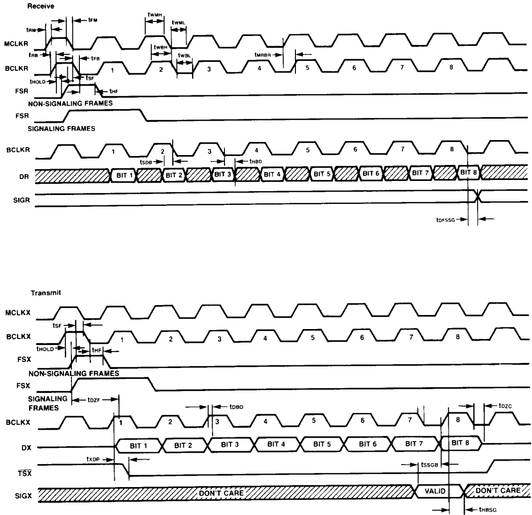
Figure 2. Short Frame Sync Timing
