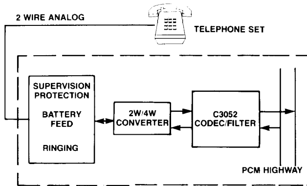
Figure 4. Typical Line Termination for Channel Bank
