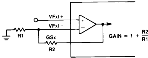
Figure 1. Transmit Filter Gain Adjustment
