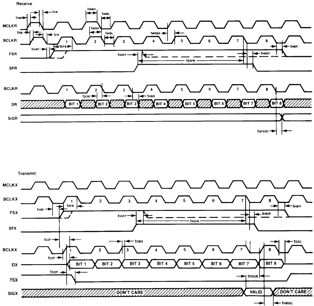
Figure 3. Long Frame Sync Timing
