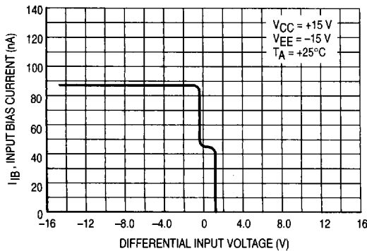
Figure 4. Input Bias Current versus Differential Input Voltage
