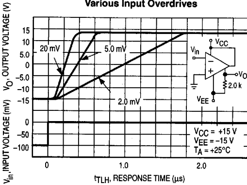
Figure 8. Response Time for Various Input Overdrives
