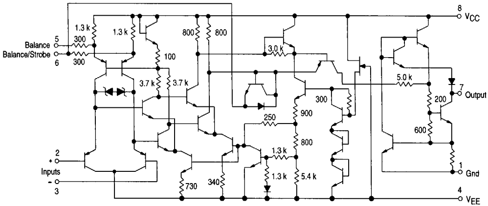
Figure 1. Circuit Schematic
