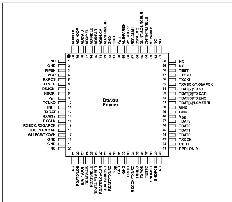
Figure 1-2. Bt8330 Pinout Diagram - 80-Pin MQFP
