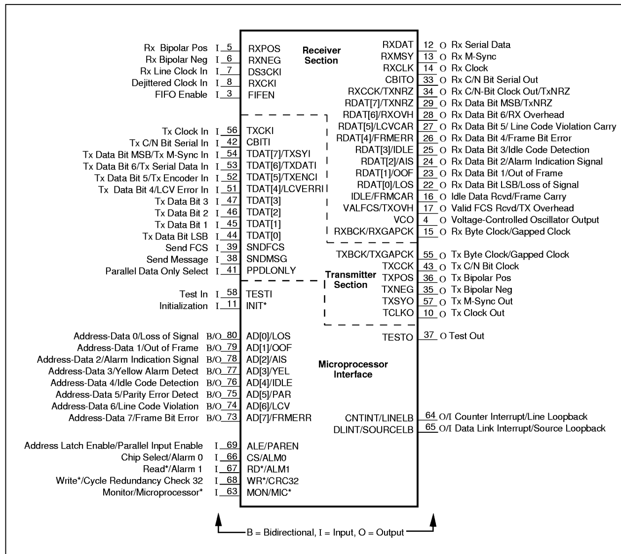
Figure 1-4. Bt8330 Framer Functional Logic Diagram - 80-Pin MQFP
