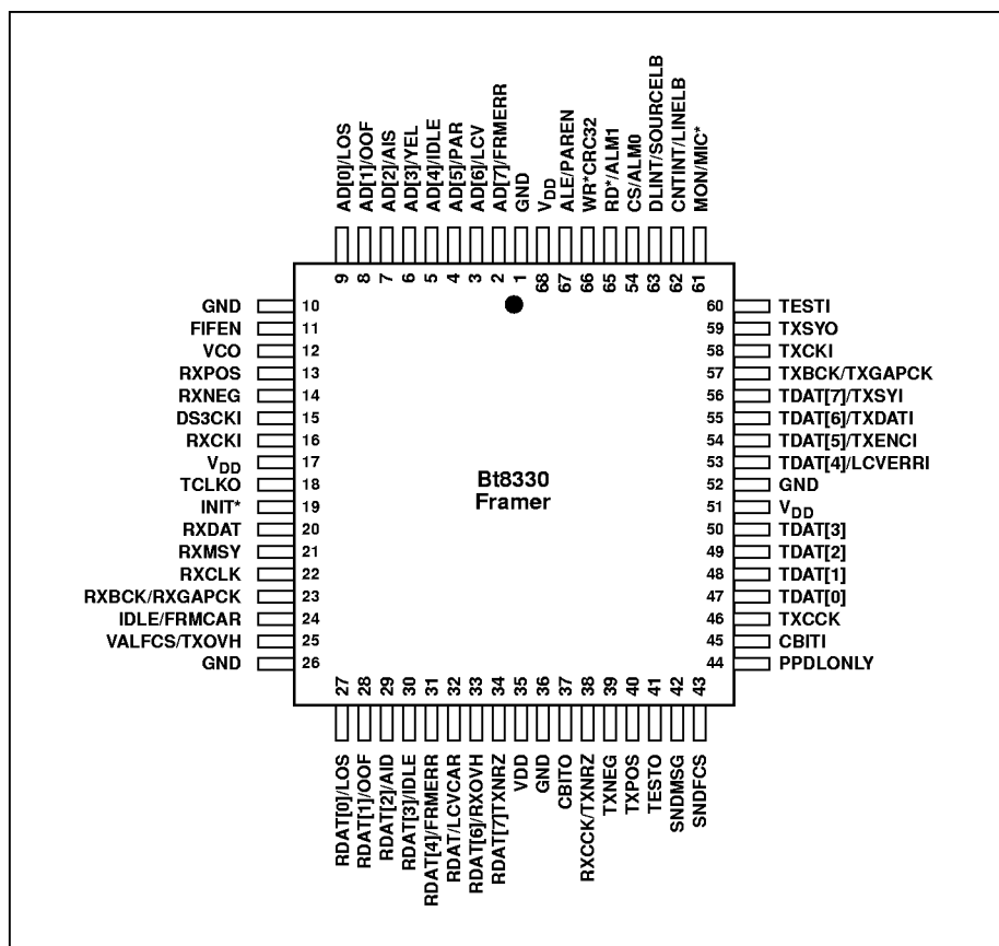
Figure 1-1. Bt8330 Pinout Diagram - 68-Pin PLCC
