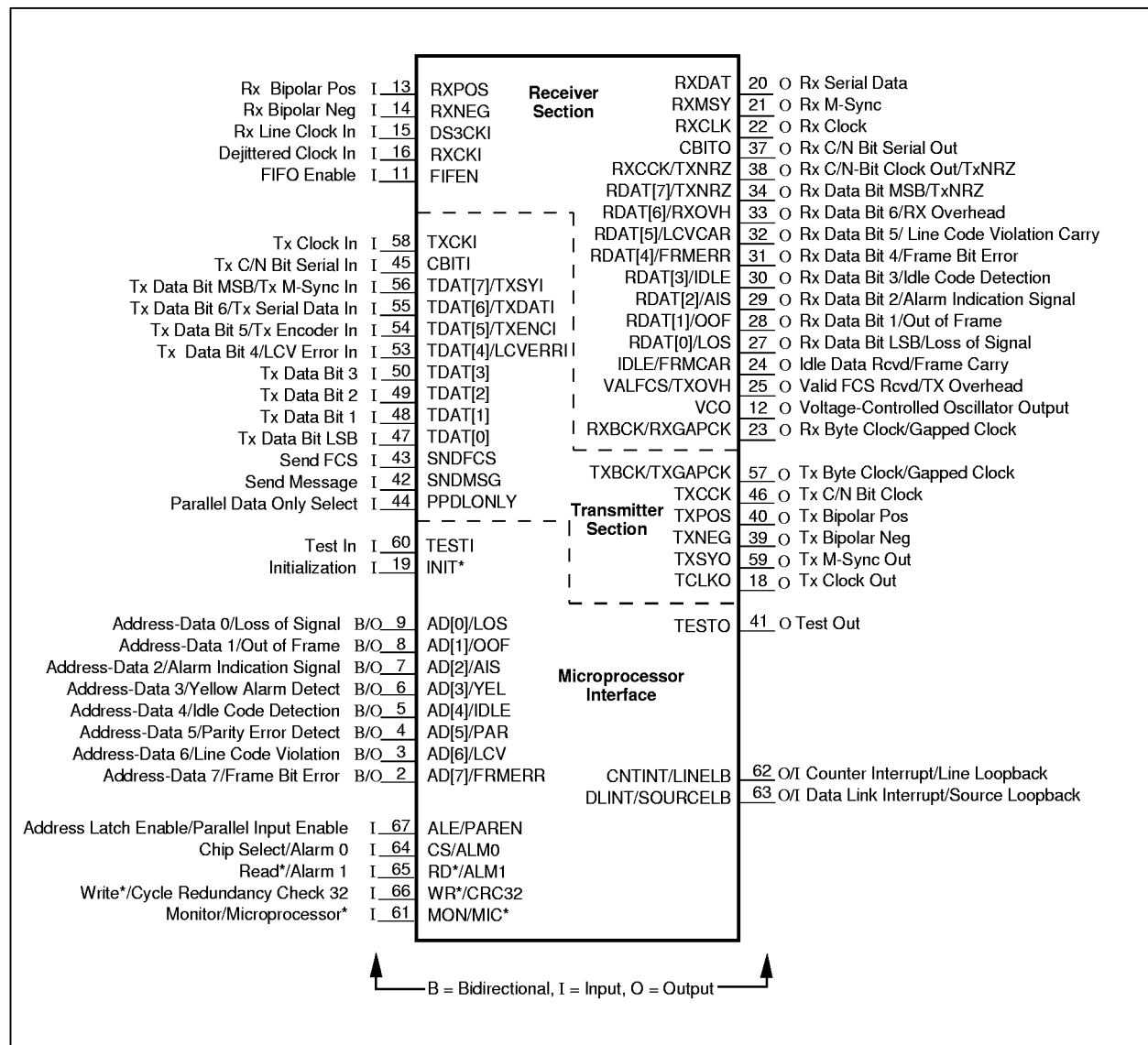
Figure 1-3. Bt8330 Framer Functional Logic Diagram - 68-Pin PLCC
