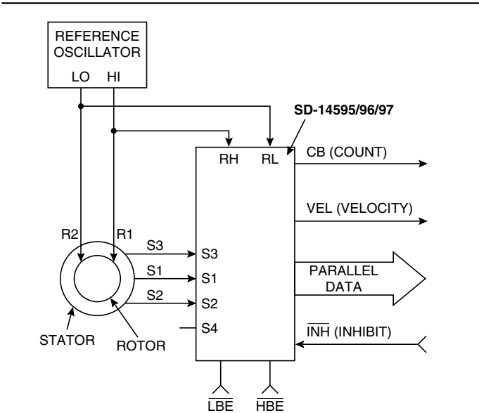
FIGURE 4. SYNCHRO INPUT CONNECTION DIAGRAM
