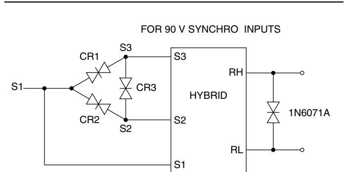
CR1, CR2, and CR3 are 1N6136A, bipolar transient voltage suppressors or equivalent.
