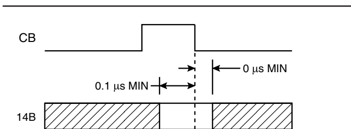
FIGURE 2. RESOLUTION CONTROL TIMING DIAGRAM
