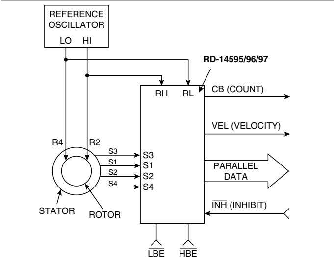
FIGURE 5. RESOLVER INPUT CONNECTION DIAGRAM
