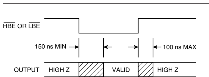
FIGURE 7. TRI-STATE OUTPUT TIMING
