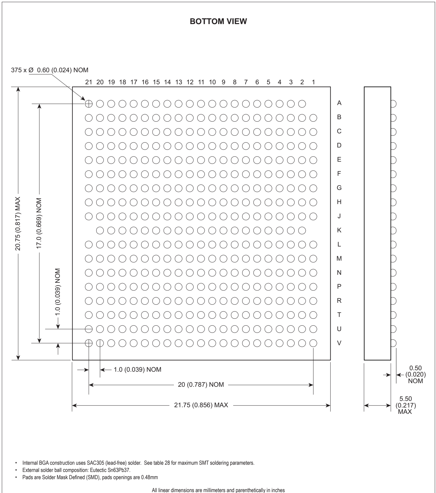
FIGURE 16 – PACKAGE DIMENSION: 375 PLASTIC BALL GRID ARRAY (PBGA) FOR W3J128M72K-XPBX
