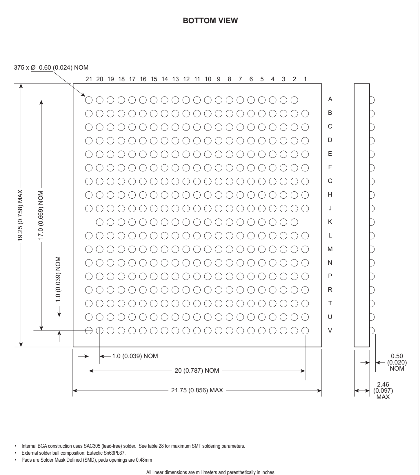
FIGURE 16A – PACKAGE DIMENSION: 375 PLASTIC BALL GRID ARRAY (PBGA) FOR W3J128M72K-XLBX
