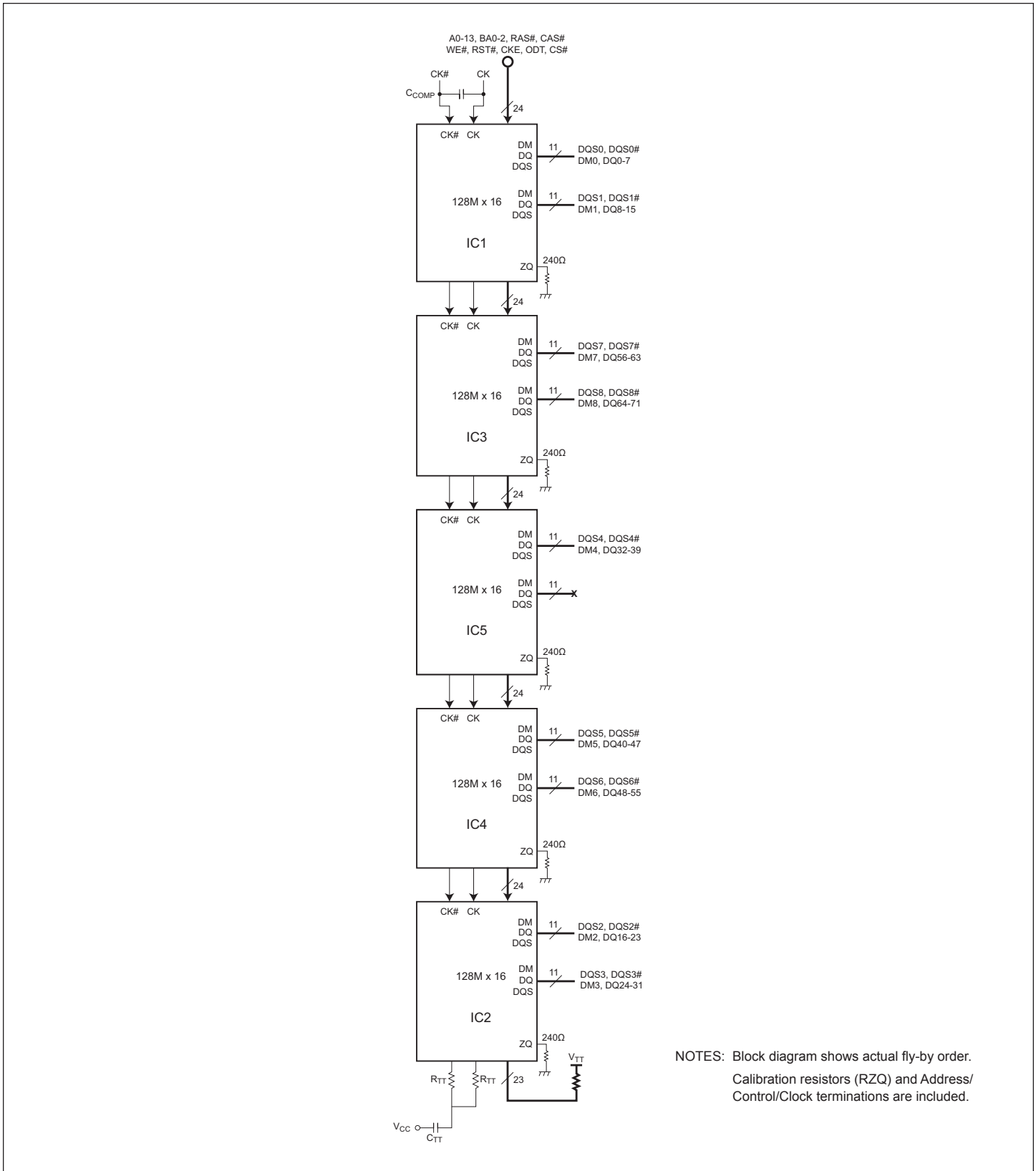
FIGURE 2A – FUNCTIONAL BLOCK DIAGRAM FOR W3J128M72K-XLBX
