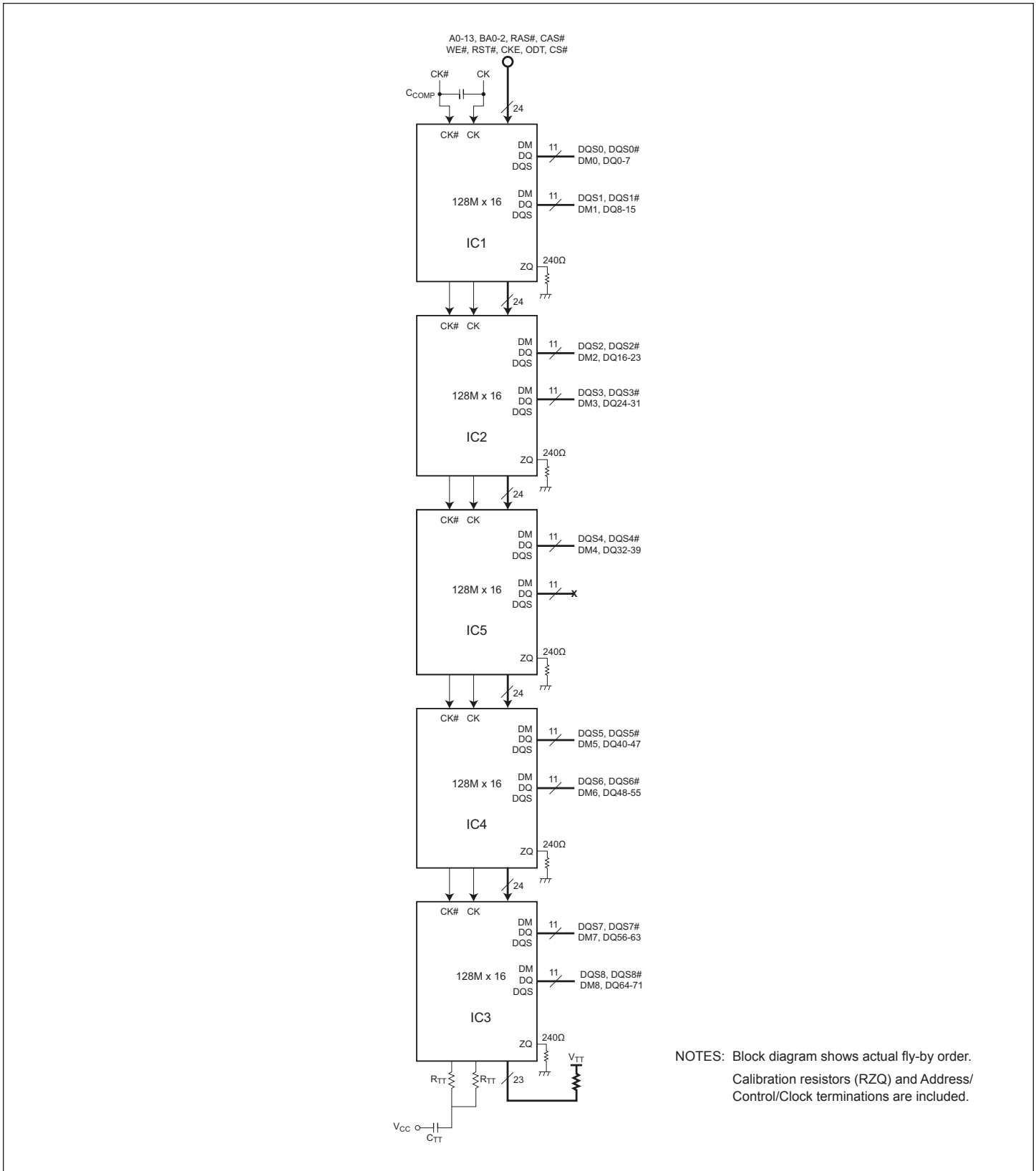
FIGURE 2 – FUNCTIONAL BLOCK DIAGRAM FOR W3J128M72K-XPBX
