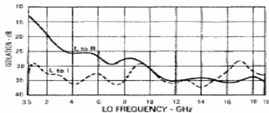
Isolation vs. Frequency
