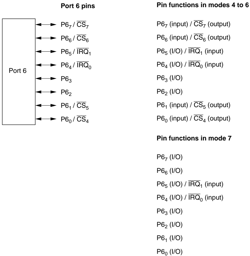
Figure 5.6 Port 6 Pin Functions
