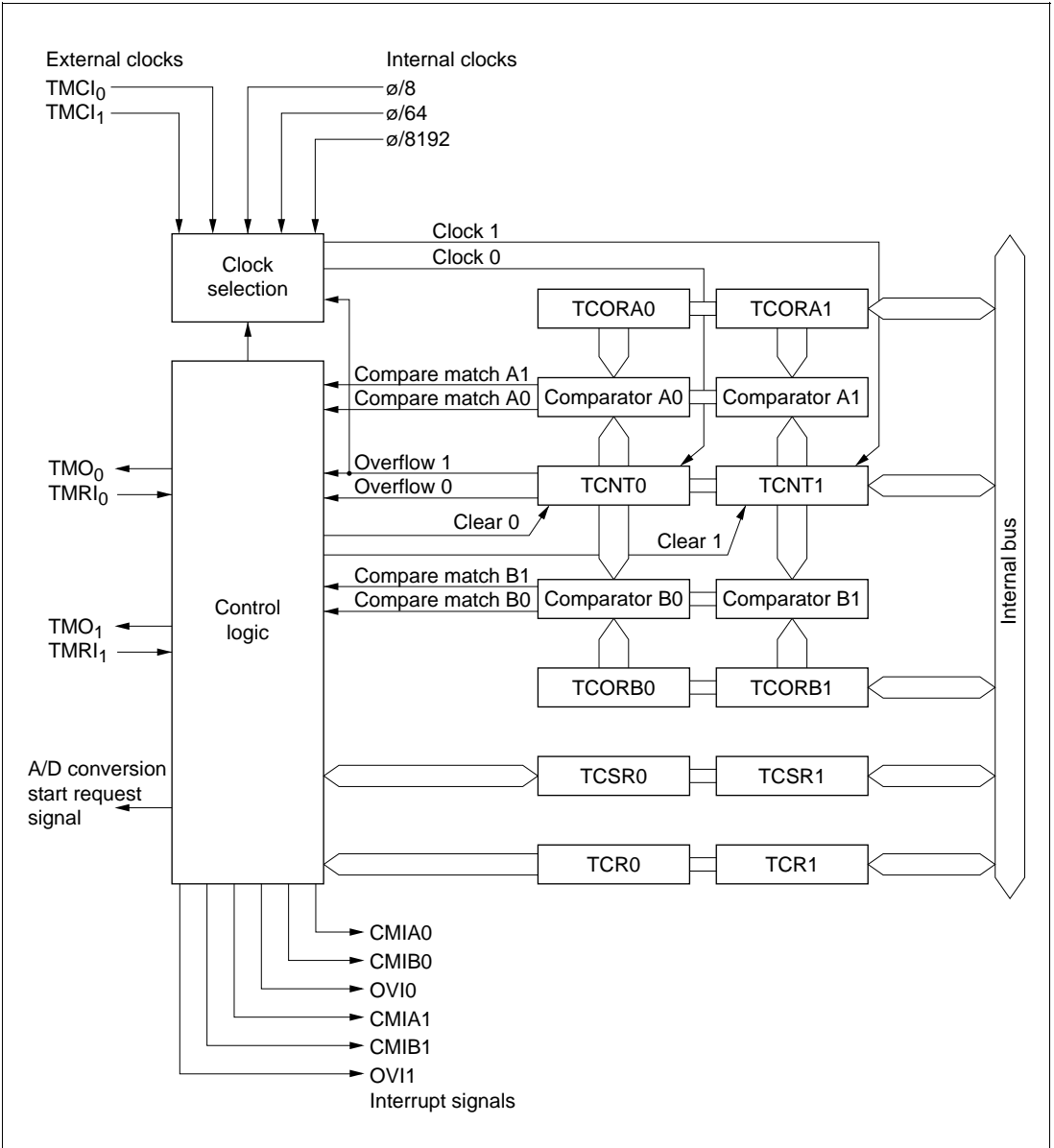
Figure 6.6 Block Diagram of 8-Bit Timer
