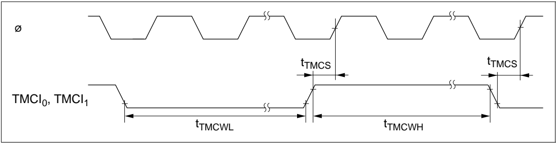
Figure 7.25 8-Bit Timer Clock Input Timing
