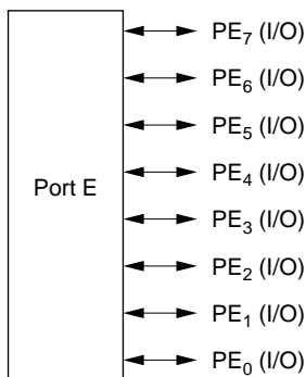
Figure 5.24 Port E Pin Functions (Mode 7)
