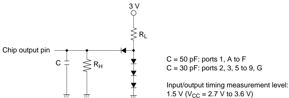
Figure 7.1 Output Load Circuit
