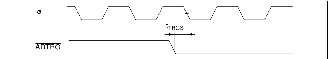
Figure 7.30 A/D Converter External Trigger Input Timing
