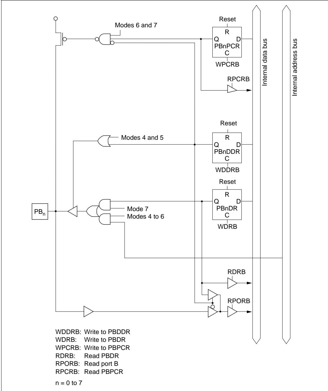
Figure 5.37 Port B Block Diagram (Pins PB n )
