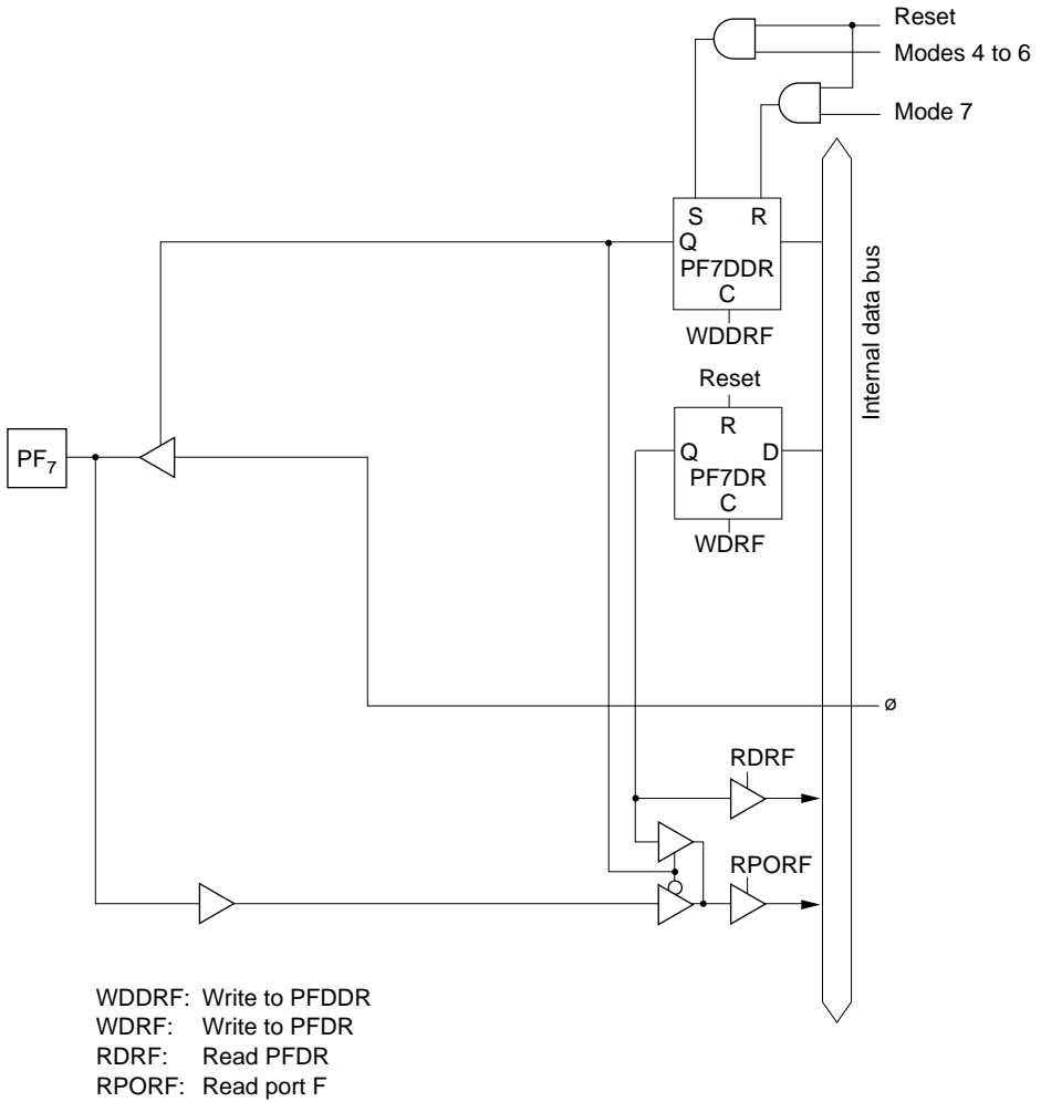
Figure 5.41 (h) Port F Block Diagram (Pin PF 7 )
