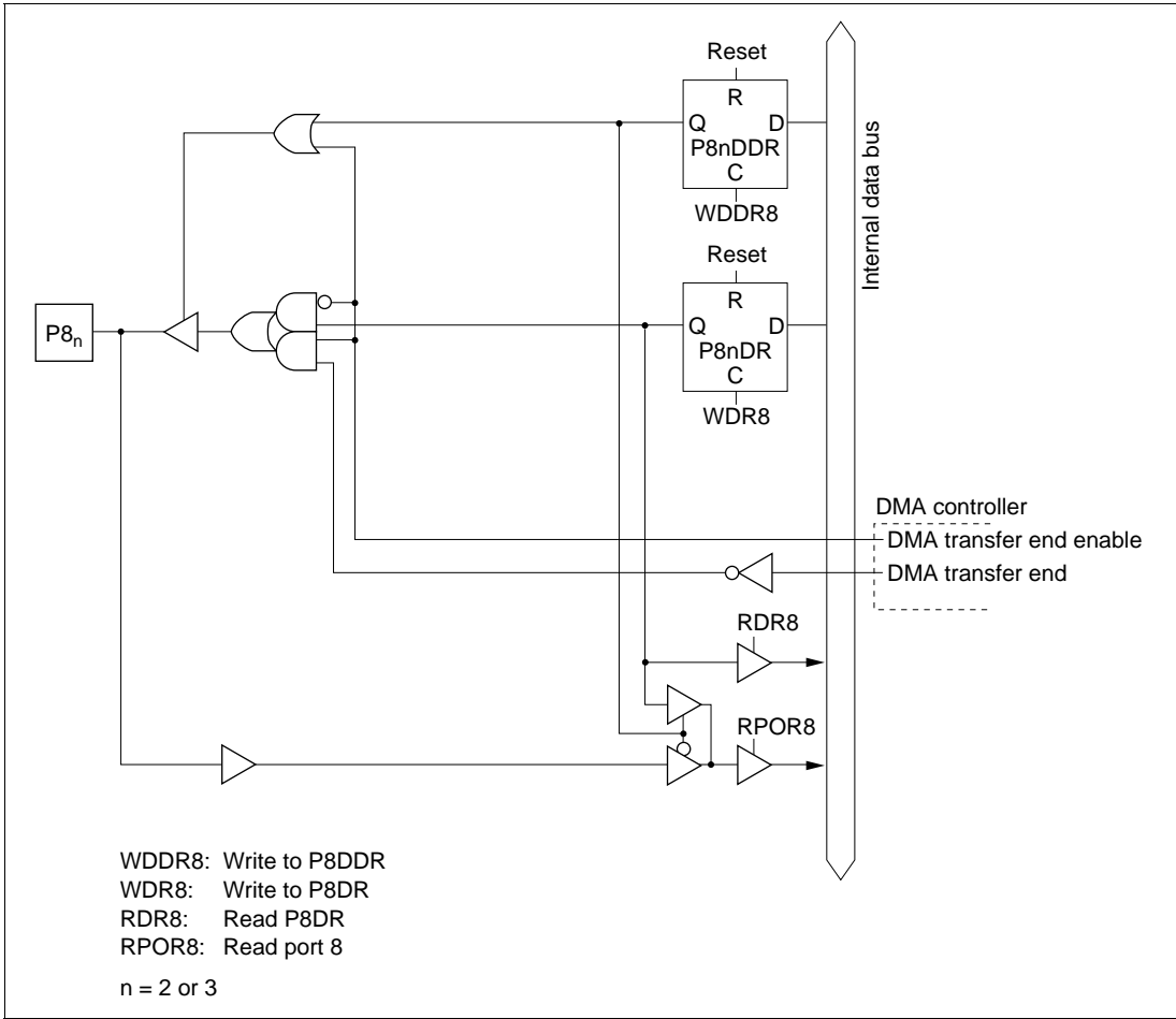
Figure 5.34 (b) Port 8 Block Diagram (Pins P8_2 and P8_3 )
