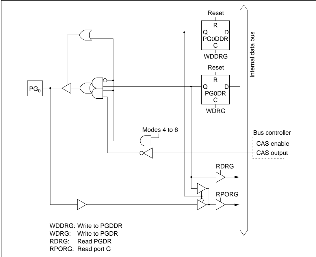
Figure 5.42 (a) Port G Block Diagram (Pin PG 0 )
