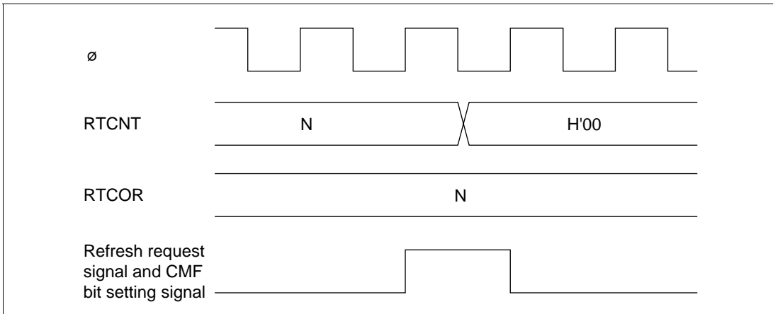
Figure 4.14 Compare Match Timing
