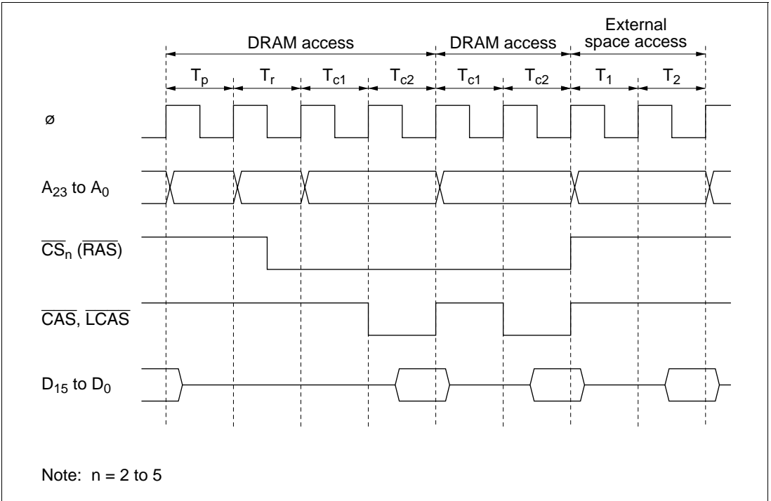
Figure 4.12 Example of Operation Timing in RAS Up Mode
