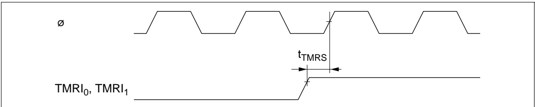
Figure 7.26 8-Bit Timer Reset Input Timing
