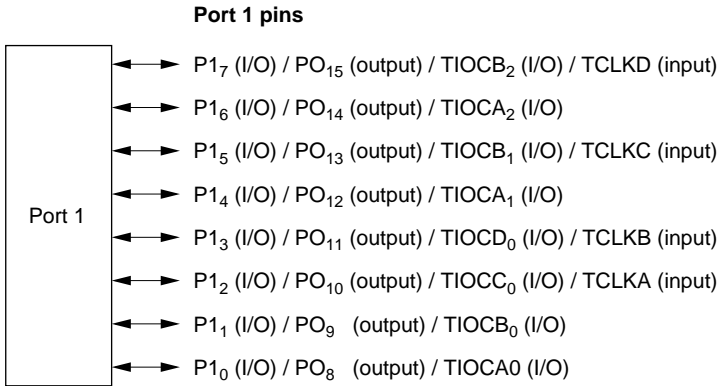
Figure 5.1 Port 1 Pin Functions
