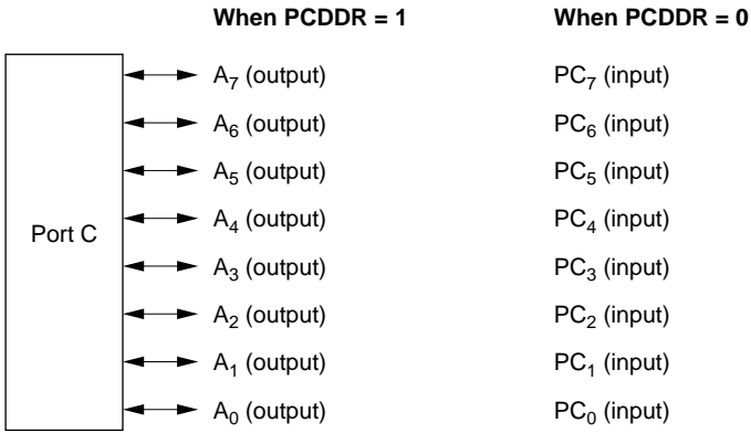
Figure 5.17 Port C Pin Functions (Mode 6)
