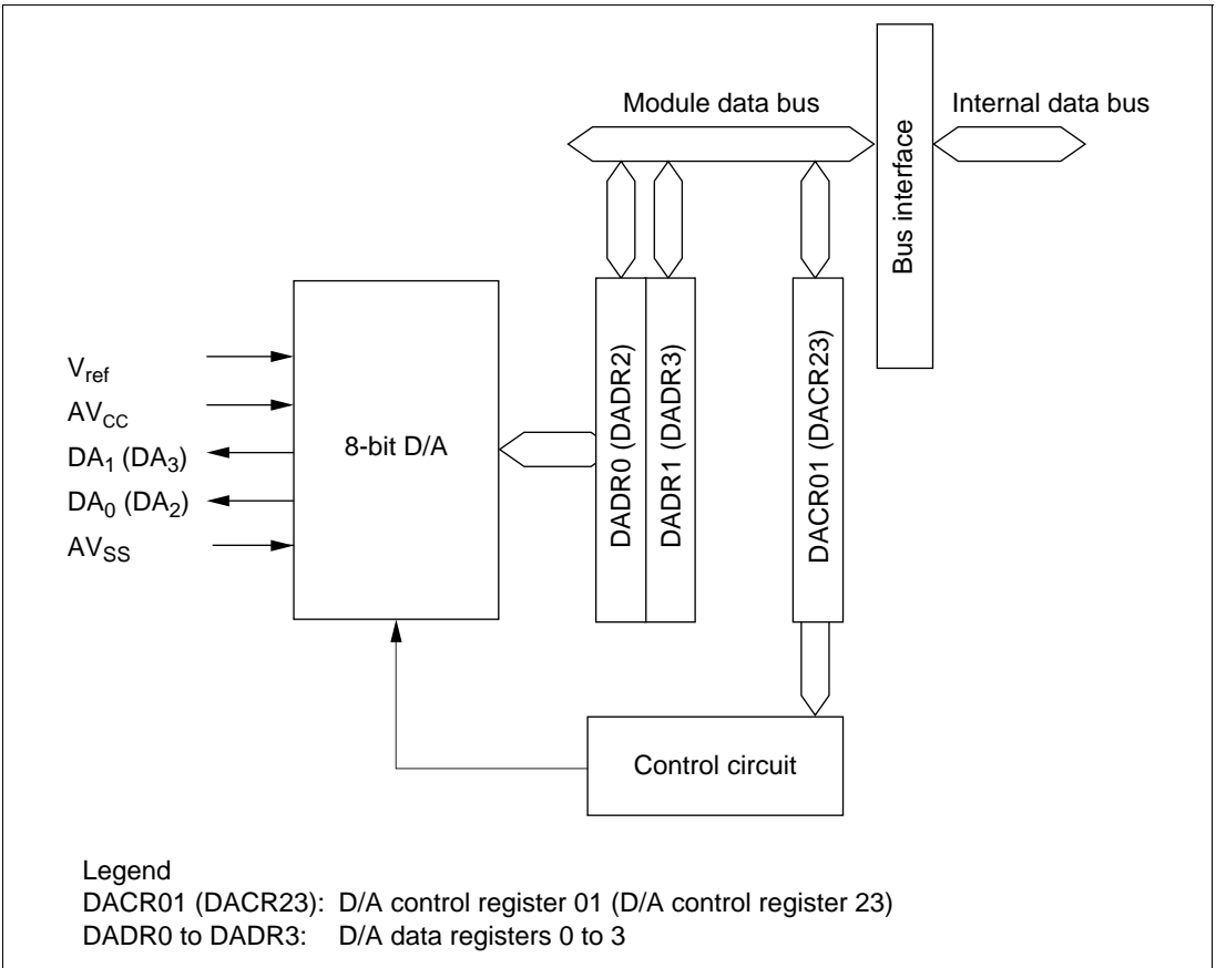
Figure 6.11 Block Diagram of D/A Converter
