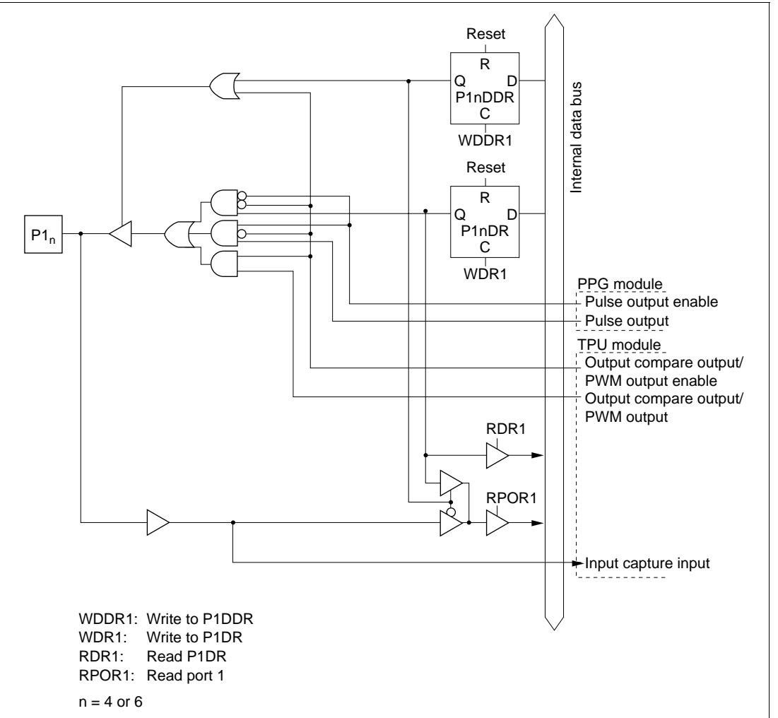
Figure 5.27 (c) Port 1 Block Diagram (Pins P1 4 and P1 6 )
