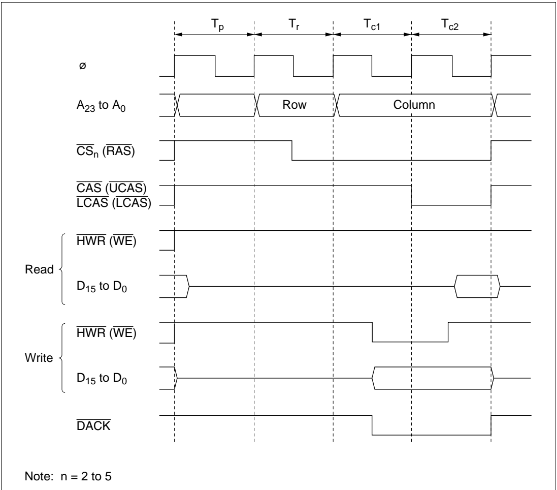
Figure 4.18 \overline{\text{DACK}} Output Timing when DDS = 1 (Example of DRAM Access)
