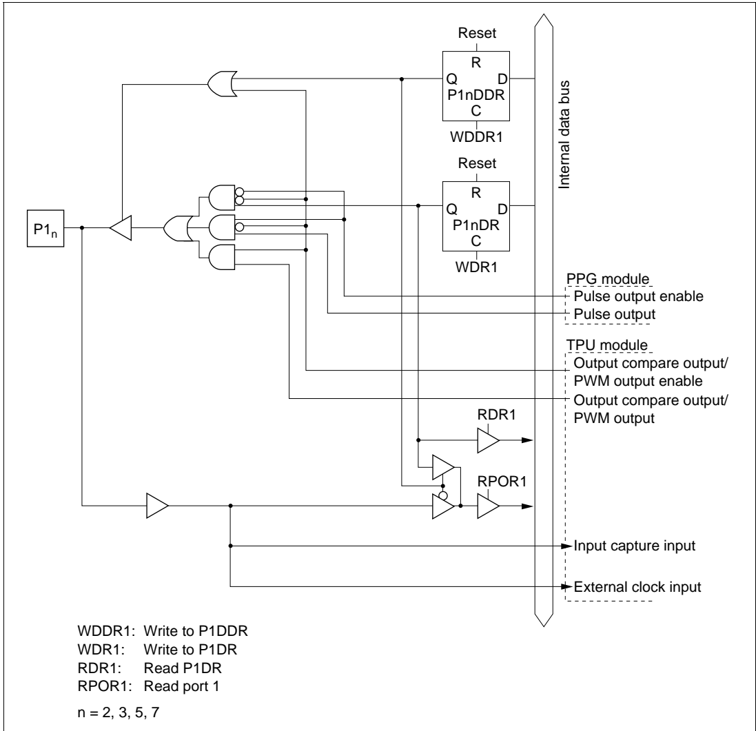
Figure 5.27 (b) Port 1 Block Diagram (Pins P1 2 , P1 3 , P1 5 , and P1 7 )
