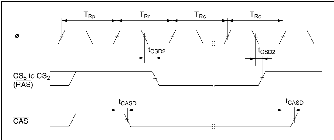
Figure 7.11 Self-Refresh Timing
