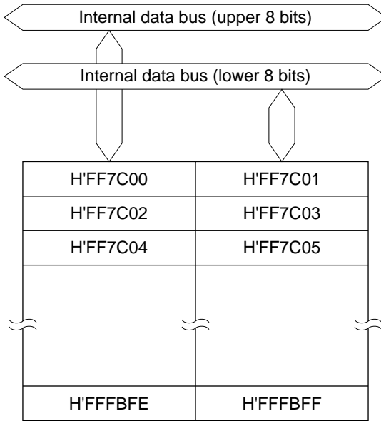
Figure 6.12 Block Diagram of RAM (32 kbytes)
