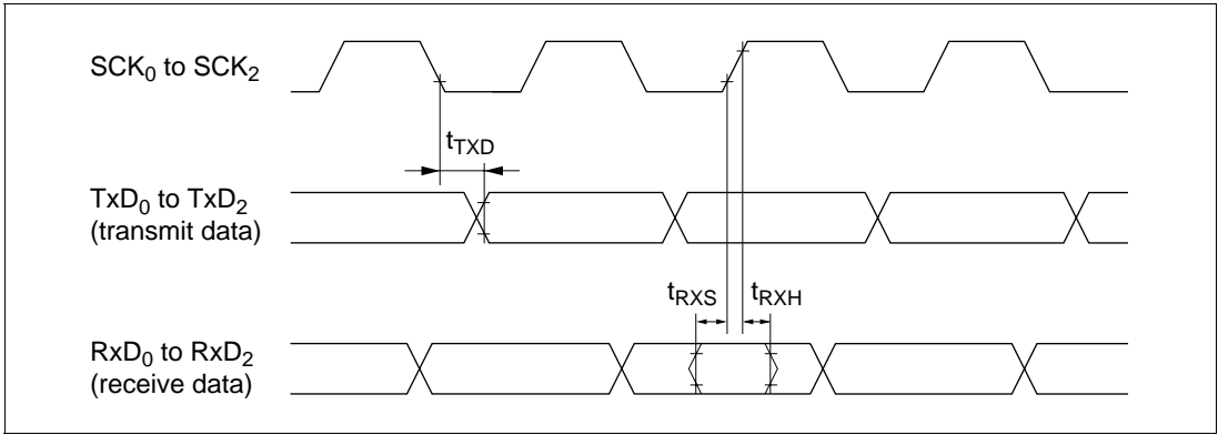
Figure 7.29 SCI Input/Output Timing (Synchronous Mode)
