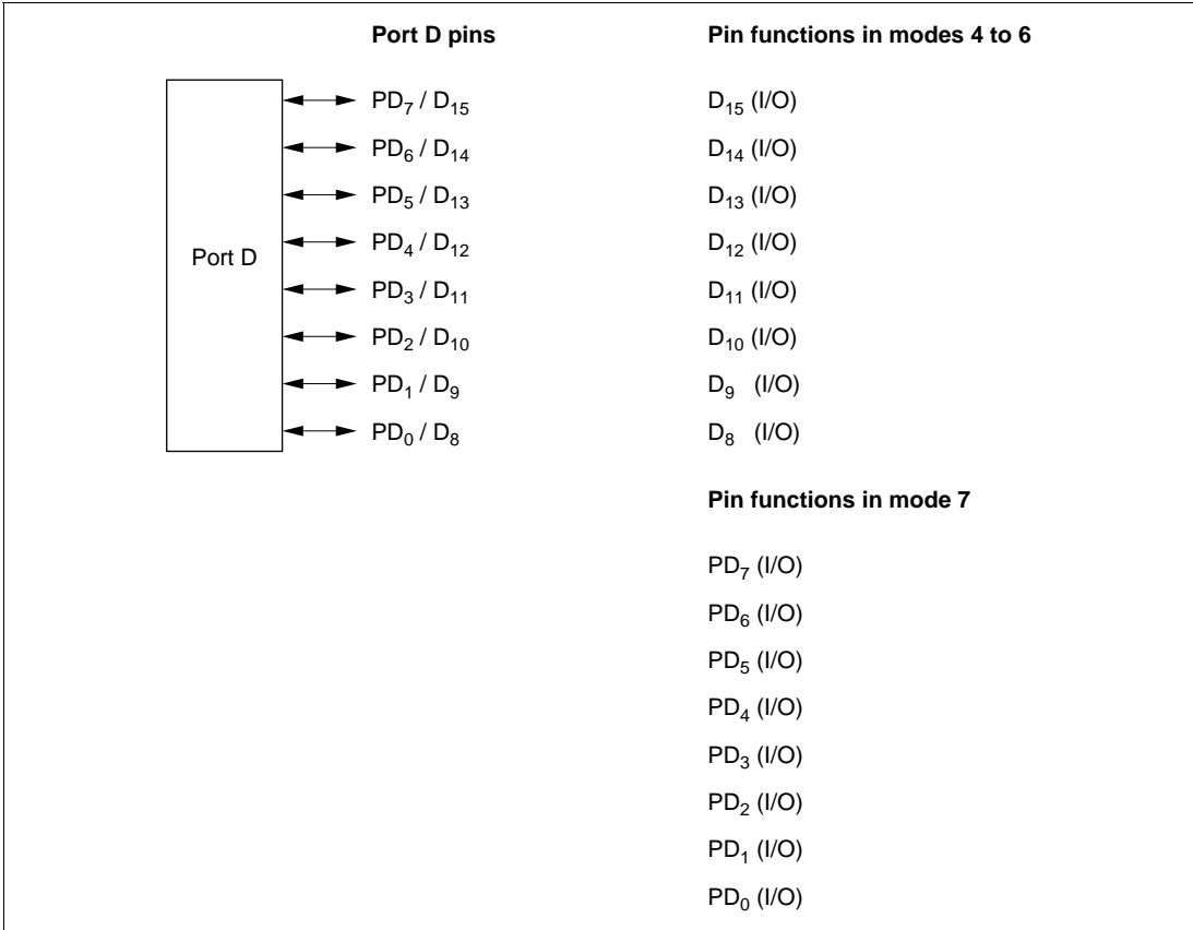
Figure 5.19 Port D Pin Functions
