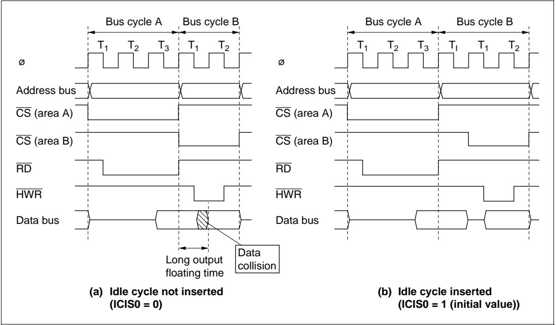
Figure 4.22 Example of Idle Cycle Operation (2)
