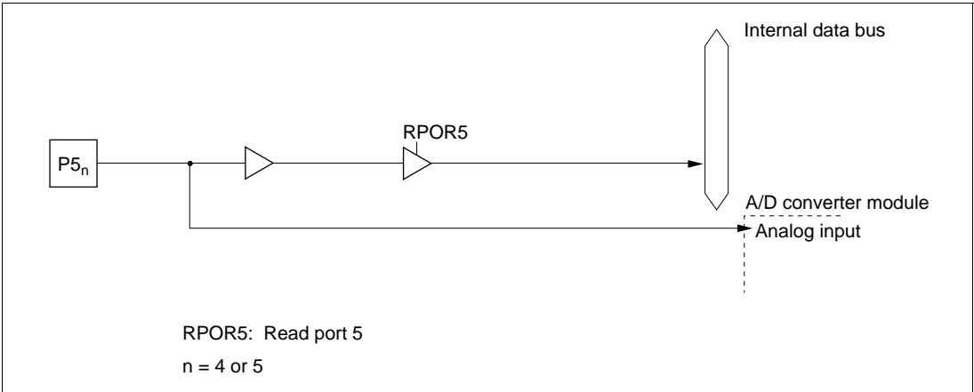
Figure 5.31 (e) Port 5 Block Diagram (Pins P5_4 and P5_5 )
