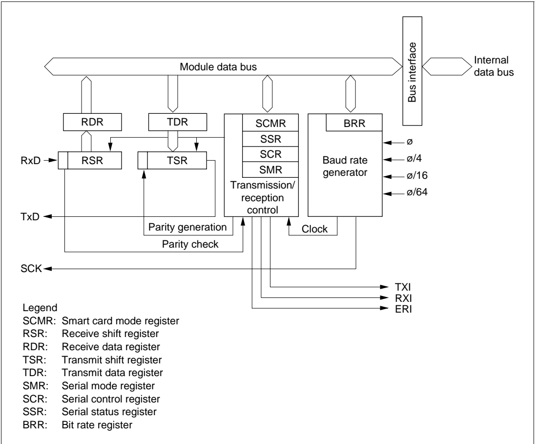
Figure 6.9 Block Diagram of Smart Card Interface
