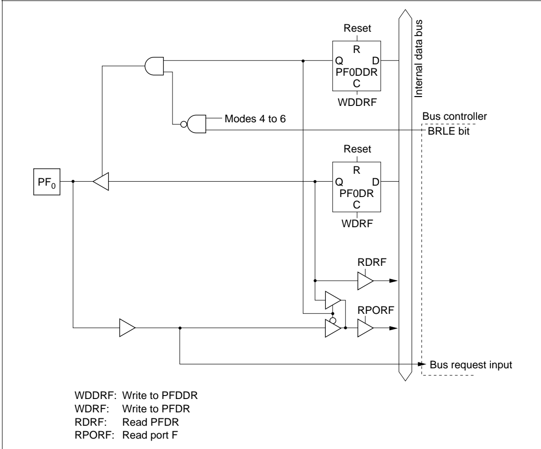
Figure 5.41 (a) Port F Block Diagram (Pin PF 0 )
