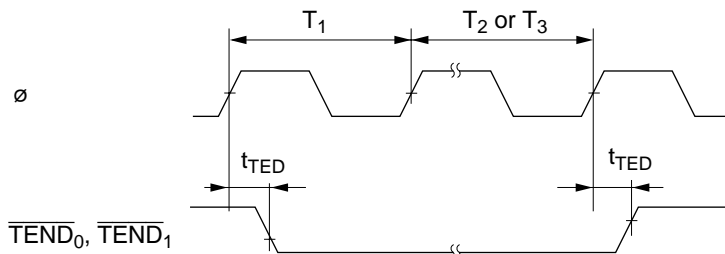
Figure 7.18 DMAC \overline{TEND} Output Timing
