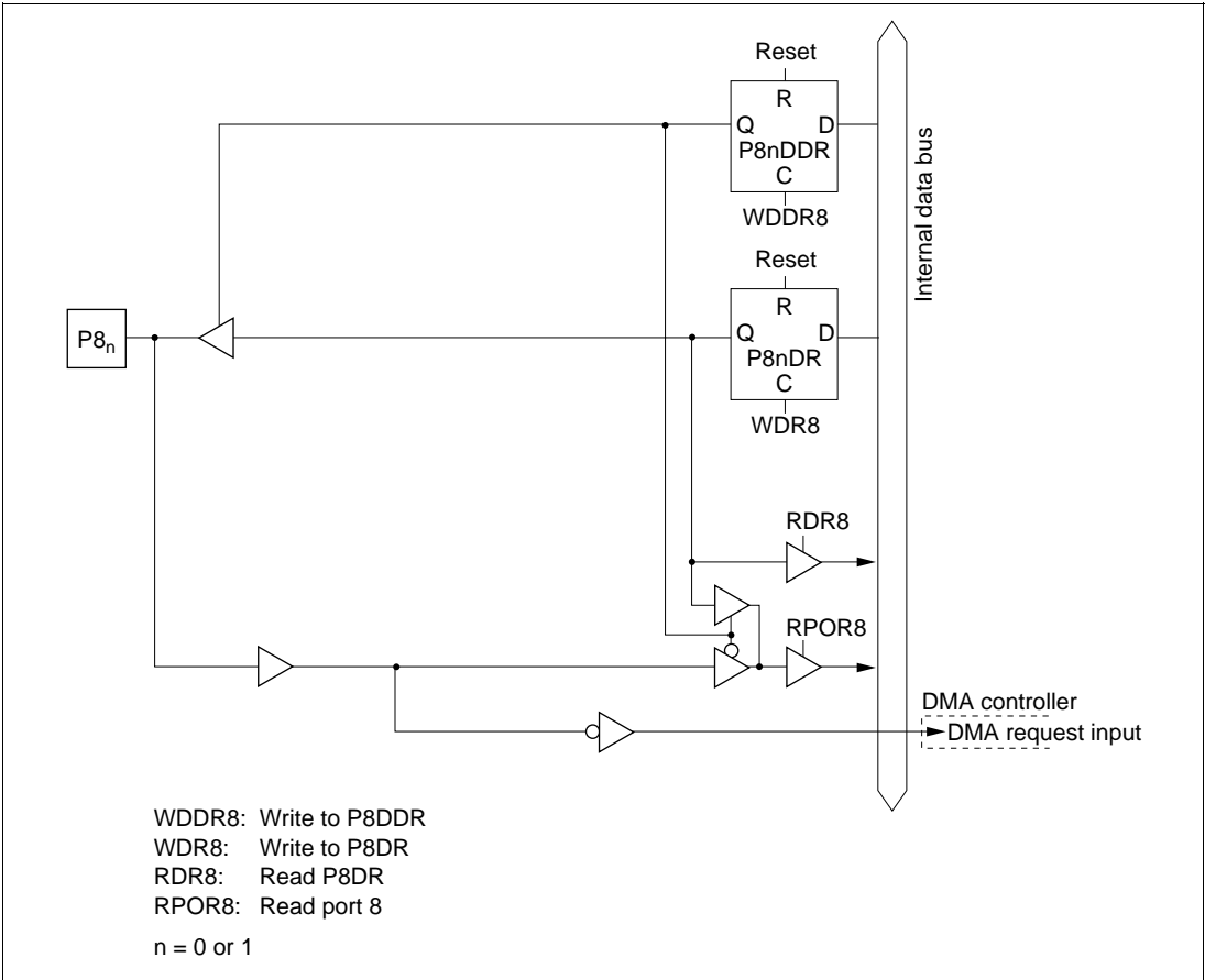
Figure 5.34 (a) Port 8 Block Diagram (Pins P8 0 and P8 1 )
