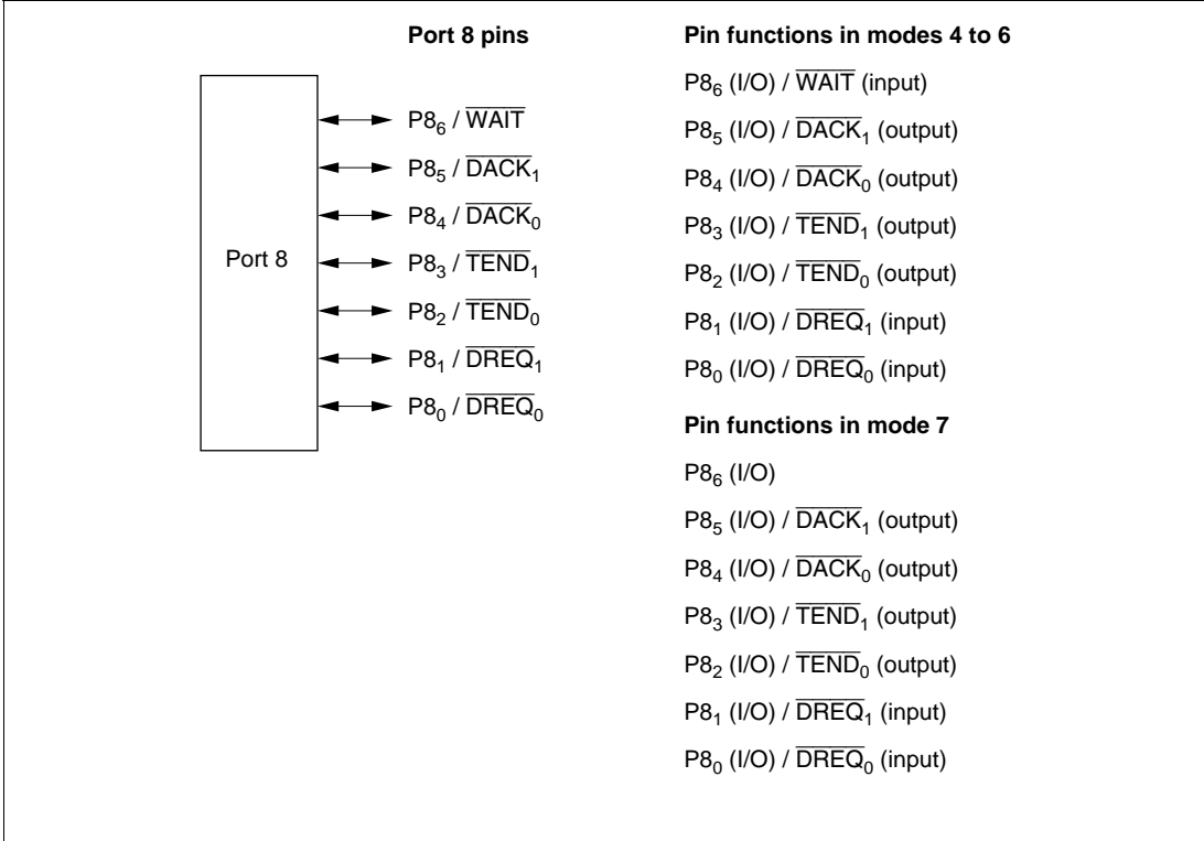
Figure 5.8 Port 8 Pin Functions
