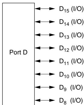
Figure 5.20 Port D Pin Functions (Modes 4 to 6)
