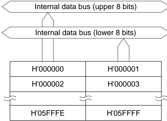
Figure 6.14 Block Diagram of Flash Memory (384 kbytes)
