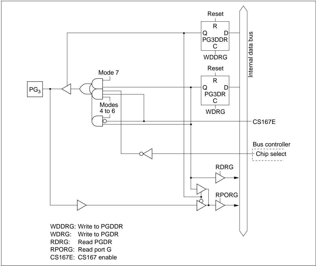
Figure 5.42 (c) Port G Block Diagram (Pin PG 3 )
