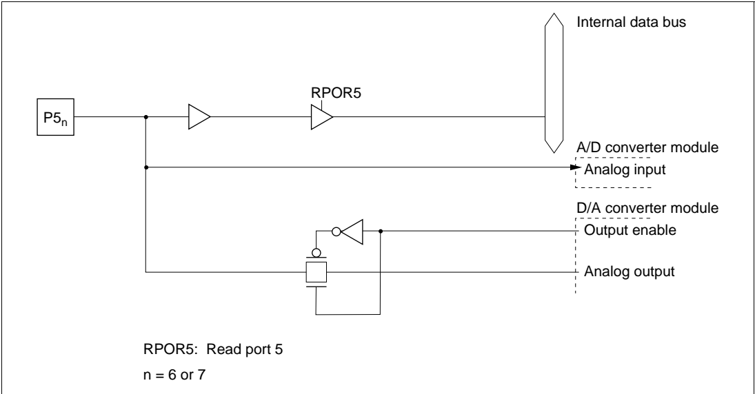
Figure 5.31 (f) Port 5 Block Diagram (Pins P5_6 and P5_7 )
