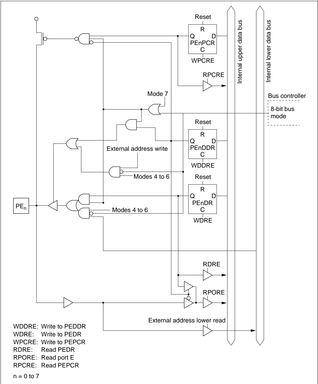
Figure 5.40 Port E Block Diagram (Pins PE n )
