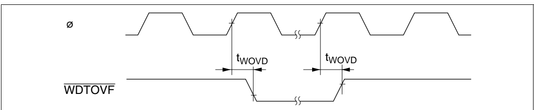
Figure 7.27 WDT Output Timing
