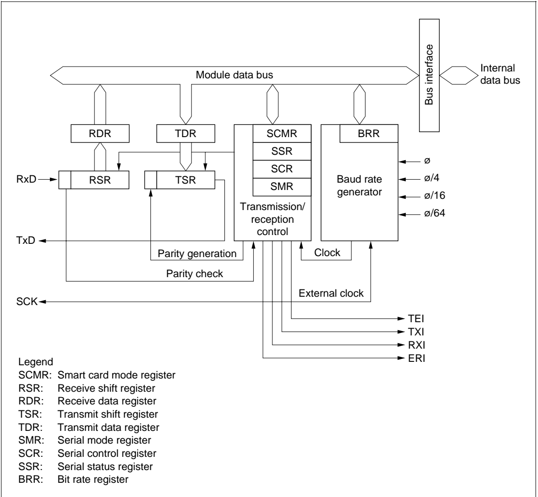
Figure 6.8 Block Diagram of SCI
