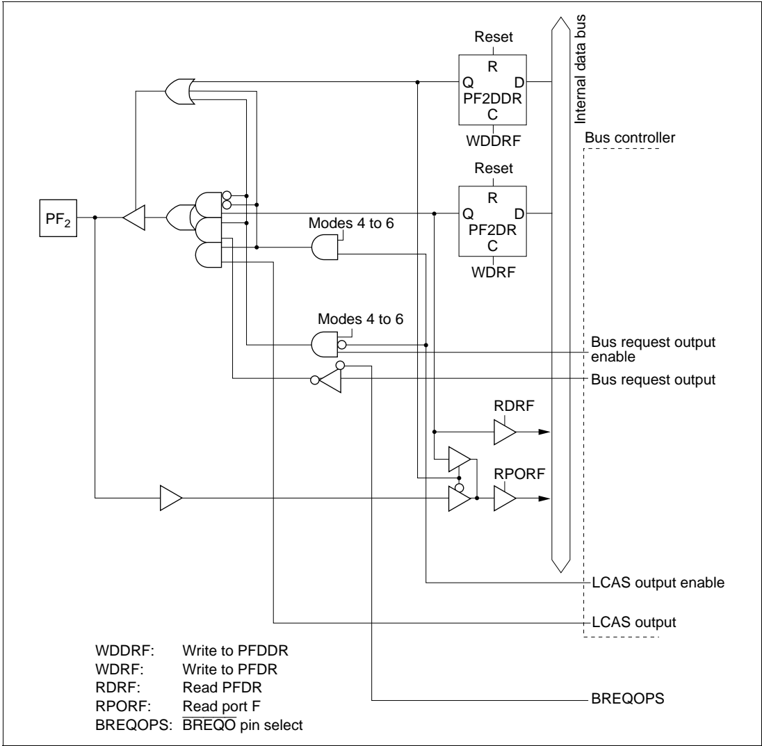
Figure 5.41 (c) Port F Block Diagram (Pin PF 2 )
