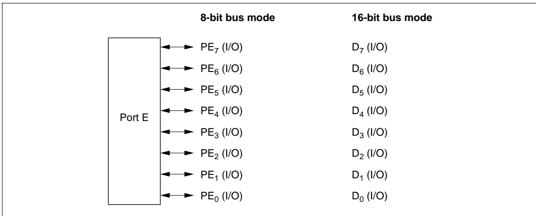
Figure 5.23 Port E Pin Functions (Modes 4 to 6)
