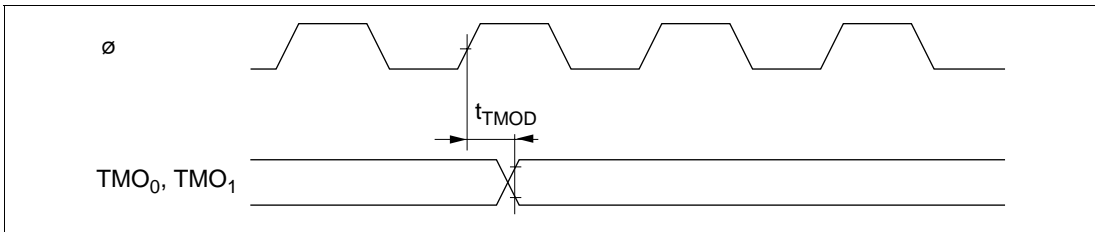
Figure 7.24 8-Bit Timer Output Timing
