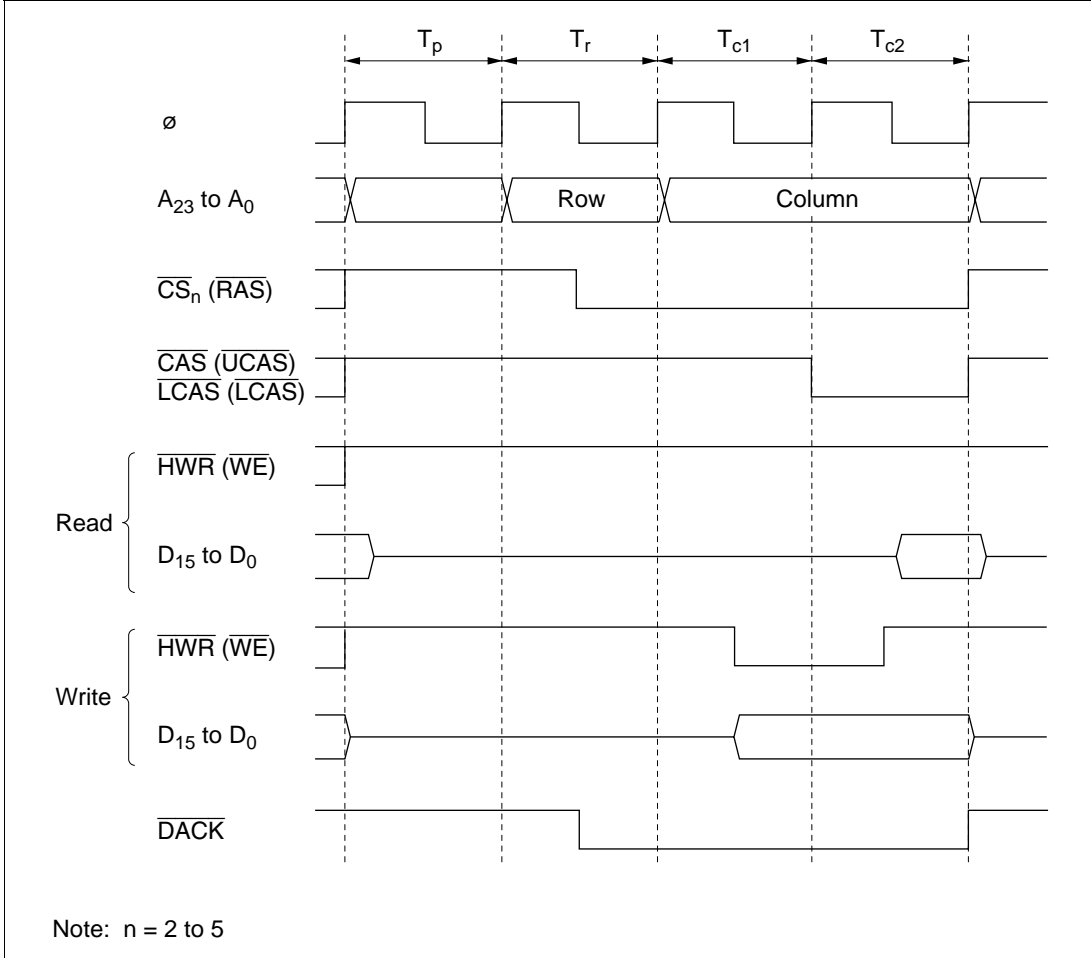
Figure 4.19 \overline{\text{DACK}} Output Timing when \text{DDS} = 0 (Example of DRAM Access)
