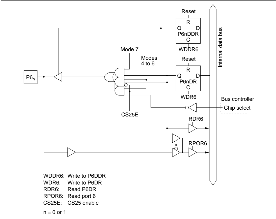
Figure 5.32 (a) Port 6 Block Diagram (Pins P6_0 and P6_1 )
