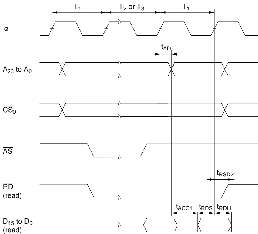
Figure 7.13 Burst ROM Access Timing (1-State Access)
