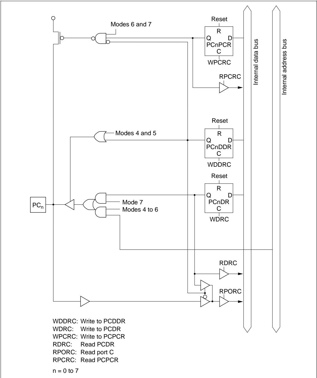
Figure 5.38 Port C Block Diagram (Pins PC n )
