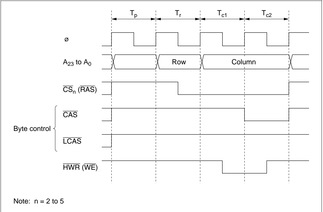
Figure 4.8 2-CAS Control Timing (Upper Byte Write Access)
