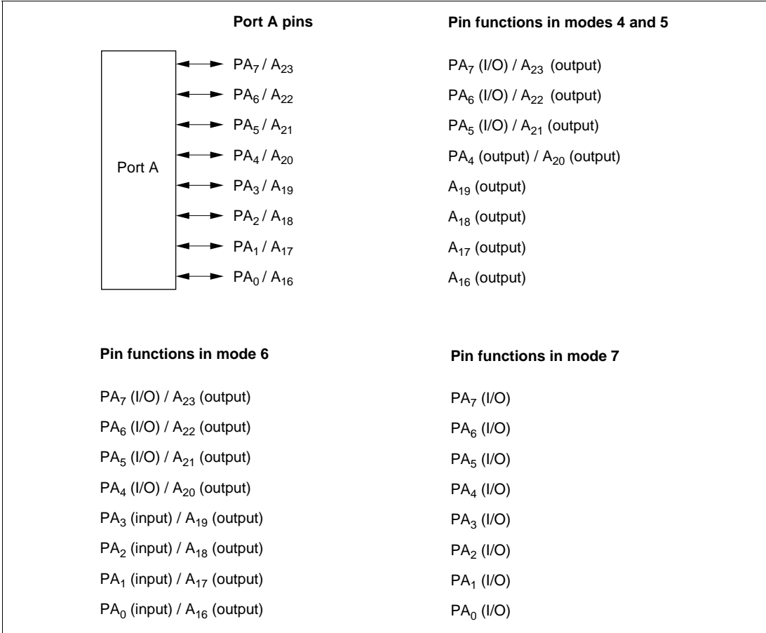
Figure 5.10 Port A Pin Functions
