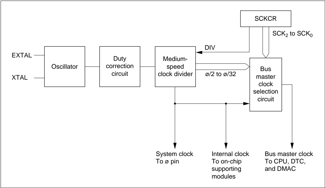
Figure 6.18 Block Diagram of Clock Pulse Generator
