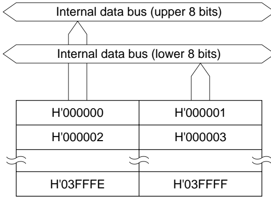
Figure 6.16 Block Diagram of Flash Memory (256 kbytes)
