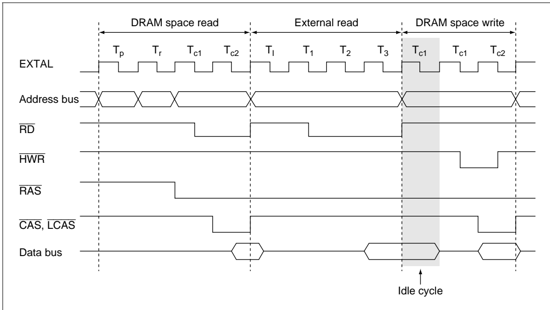
Figure 4.25 (b) Example of Idle Cycle Insertion in RAS Down Mode (ICIS0 = 1)
