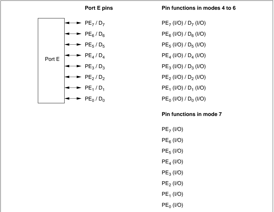
Figure 5.22 Port E Pin Functions
