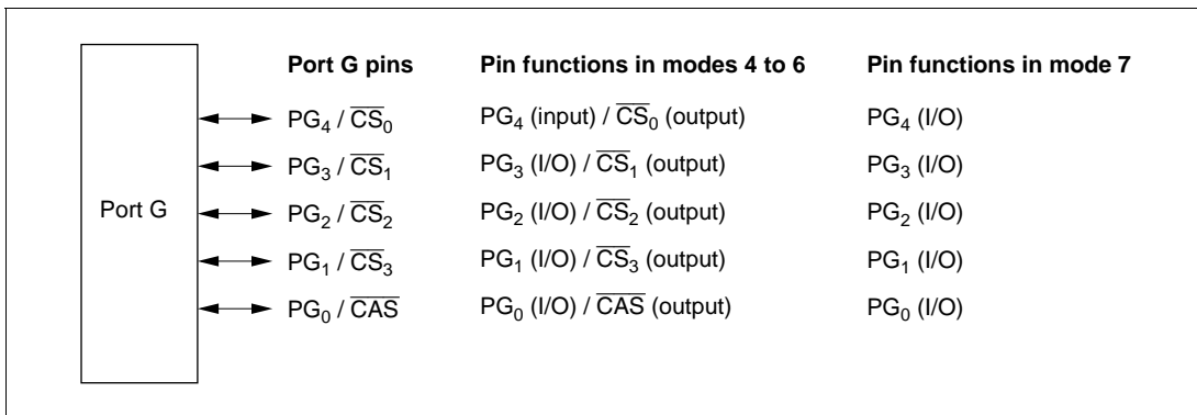
Figure 5.26 Port G Pin Functions
