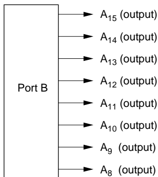
Figure 5.12 Port B Pin Functions (Modes 4 and 5)
