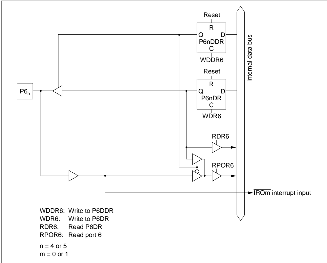
Figure 5.32 (c) Port 6 Block Diagram (Pins P6 4 and P6 5 )
