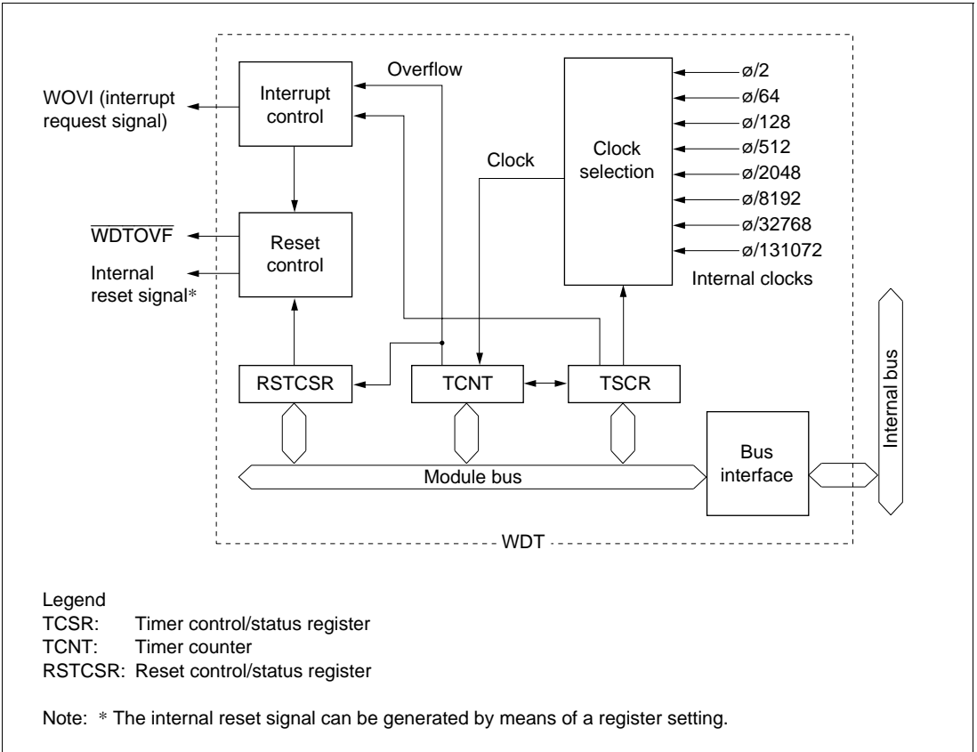
Figure 6.7 Block Diagram of WDT
