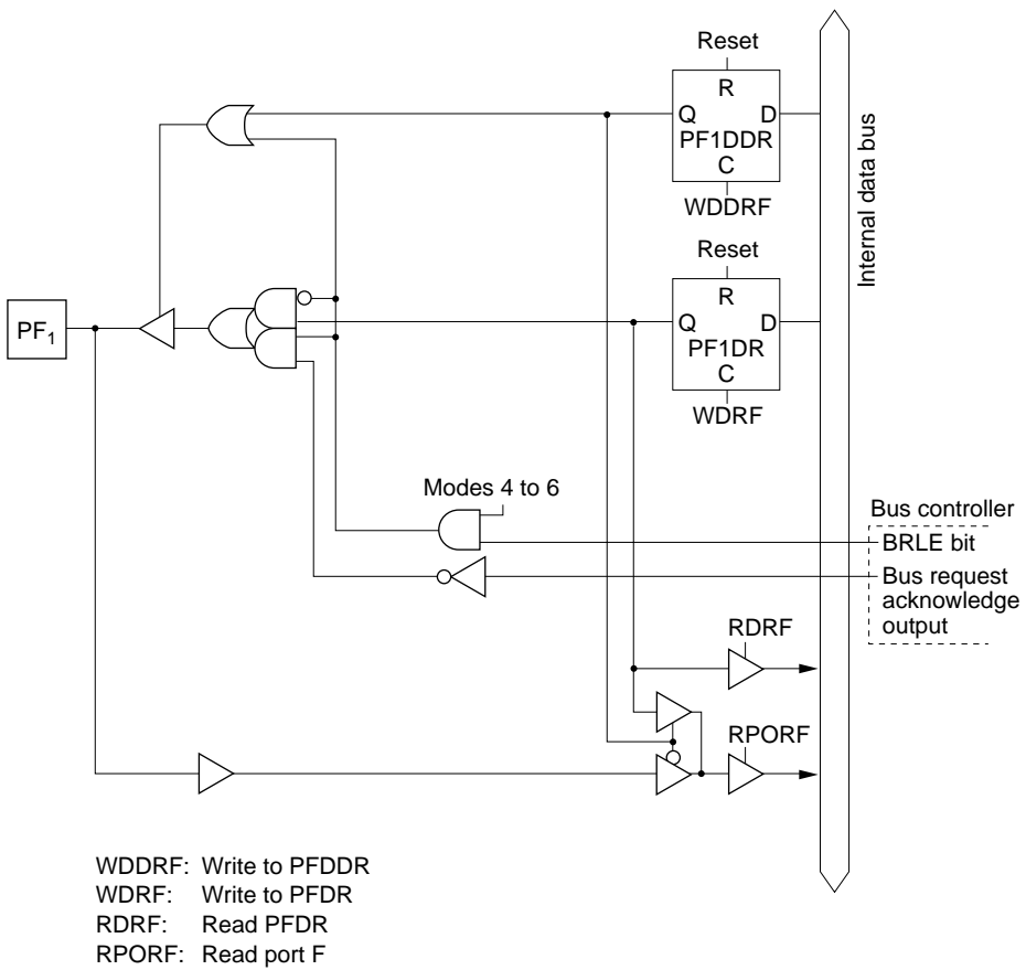
Figure 5.41 (b) Port F Block Diagram (Pin PF 1 )
