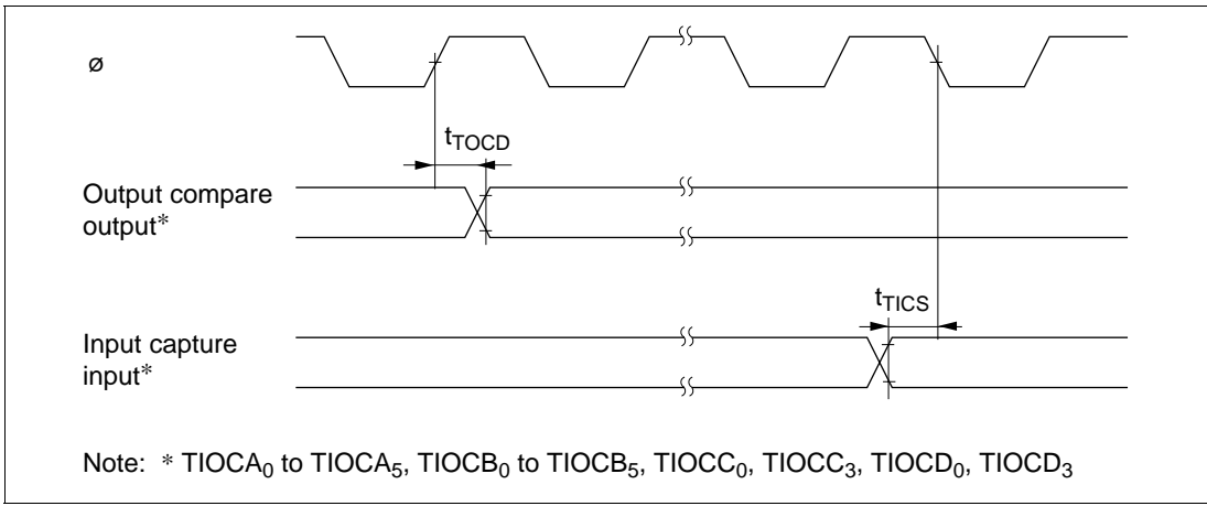
Figure 7.22 TPU Input/Output Timing
