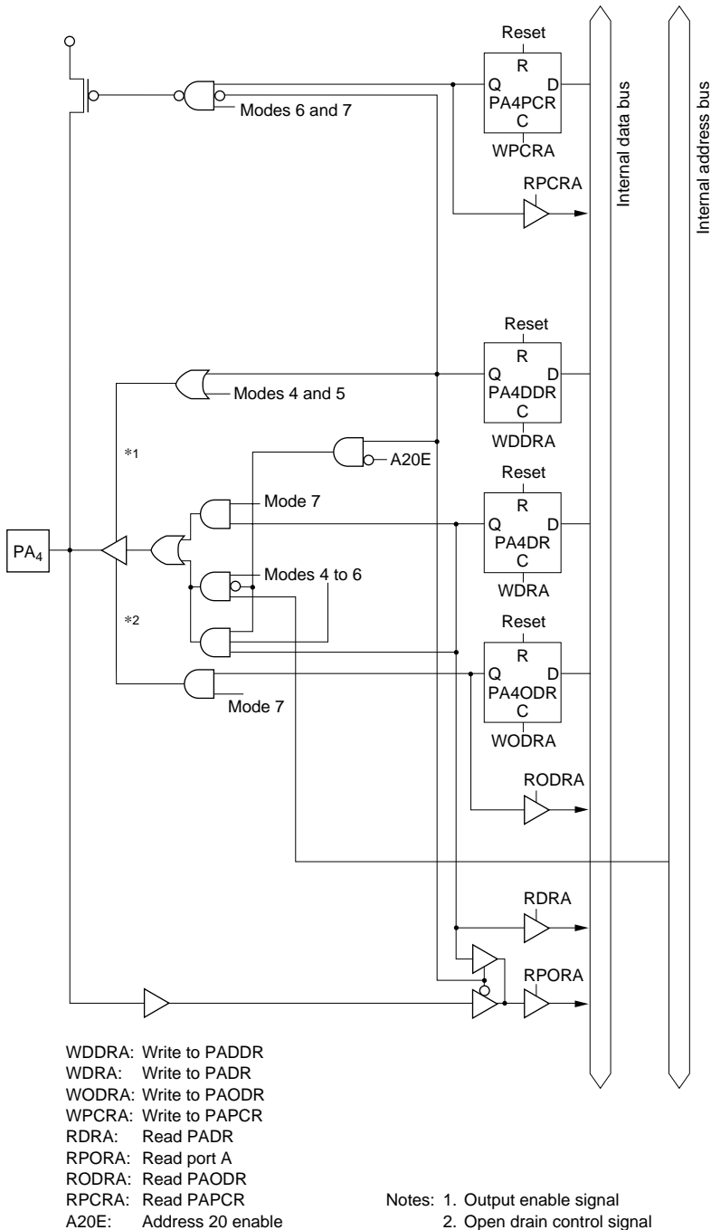
Figure 5.36 (b) Port A Block Diagram (Pin PA 4 )
