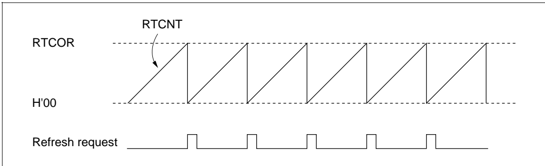
Figure 4.13 RTCNT Operation
