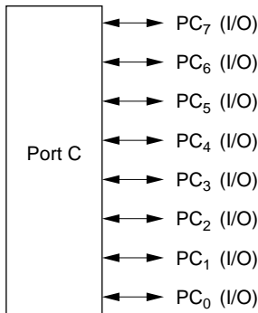
Figure 5.18 Port C Pin Functions (Mode 7)
