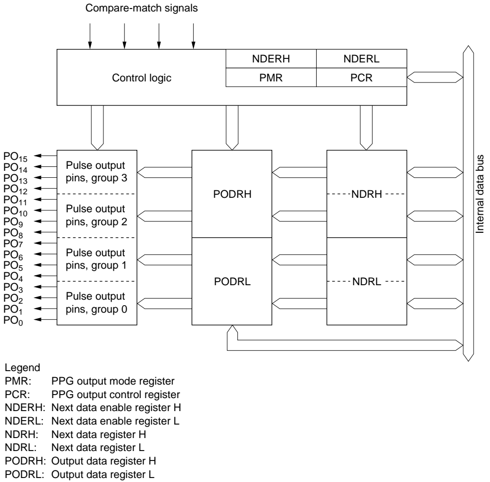
Figure 6.5 Block Diagram of PPG
