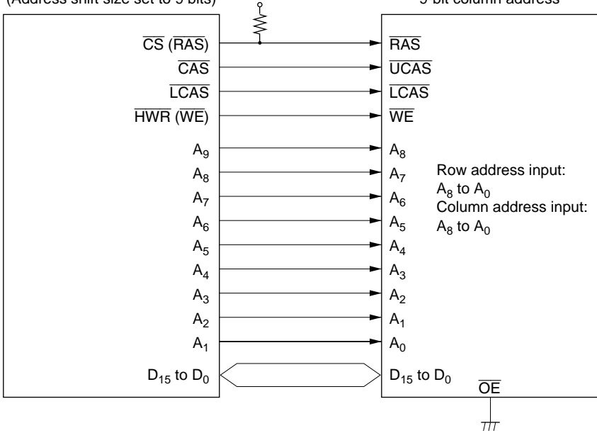
Figure 4.9 Example of 2-CAS DRAM Connection
