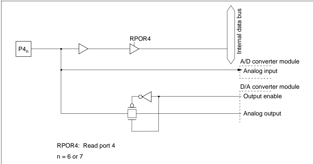
Figure 5.30 (b) Port 4 Block Diagram (Pins P4_6 and P4_7 )
