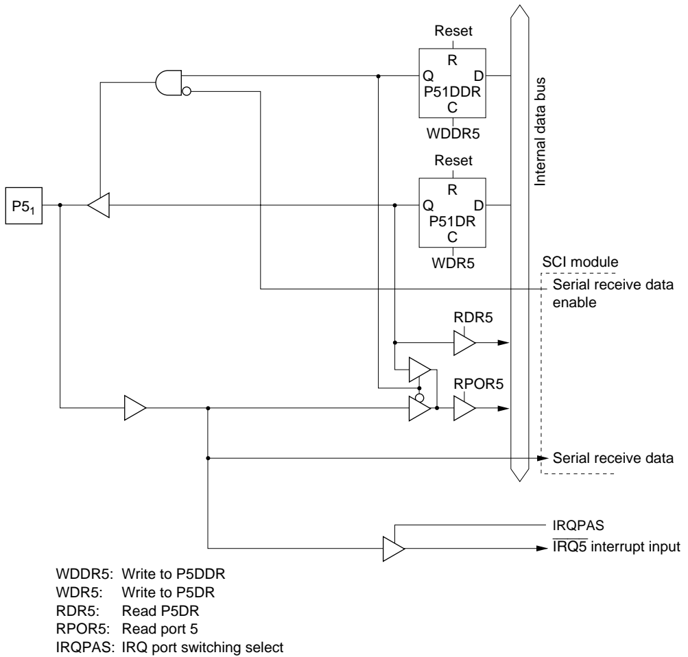
Figure 5.31 (b) Port 5 Block Diagram (Pin P5 1 )
