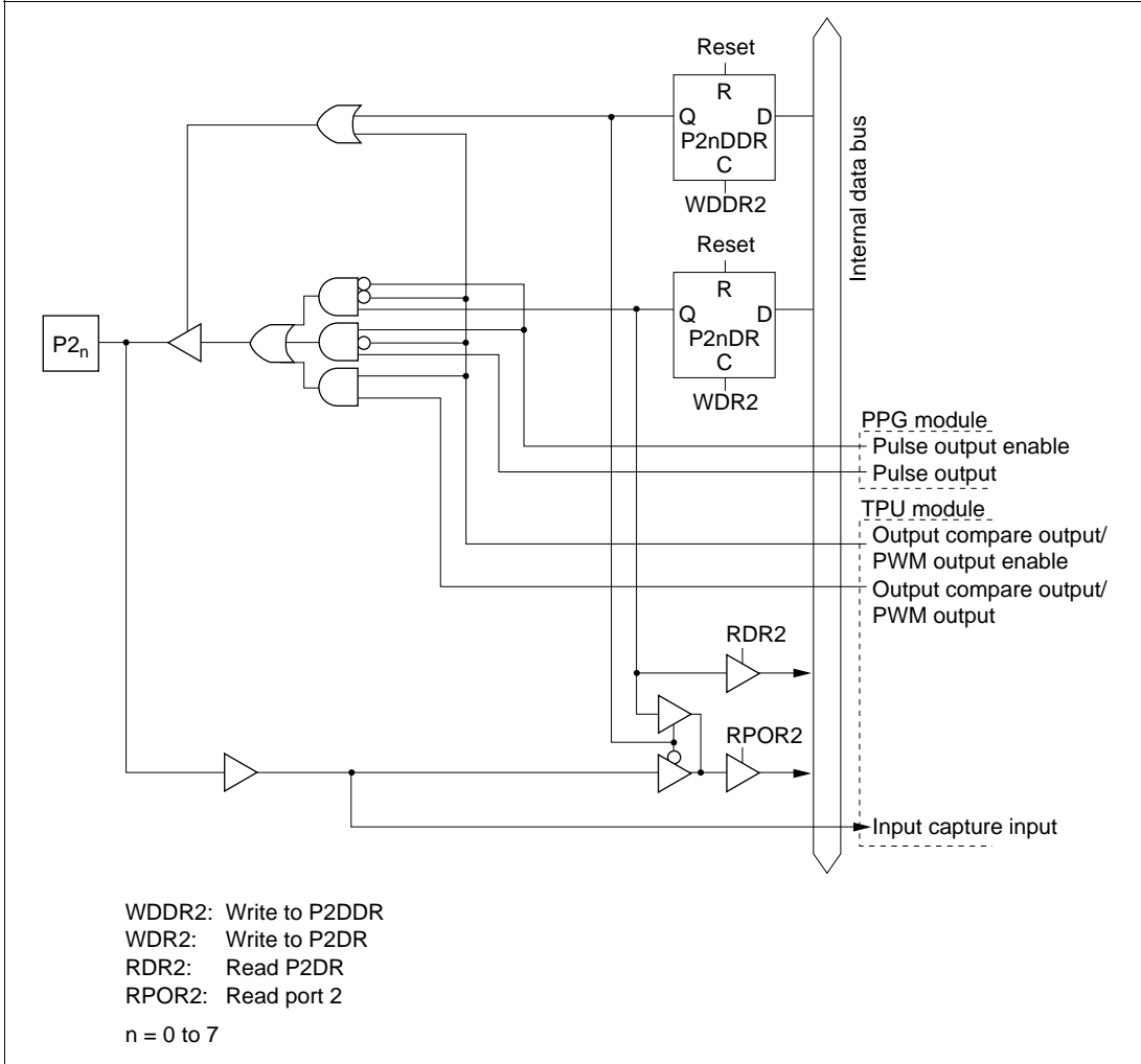
Figure 5.28 Port 2 Block Diagram (Pins P2_n )
