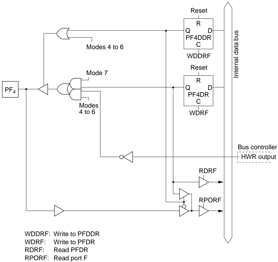
Figure 5.41 (e) Port F Block Diagram (Pin PF 4 )
