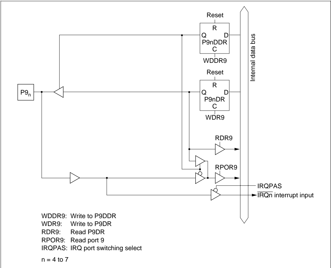
Figure 5.35 (a) Port 9 Block Diagram (Pins P9_4 to P9_7 )
