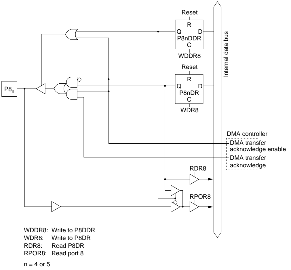
Figure 5.34 (c) Port 8 Block Diagram (Pins P8_4 and P8_5 )
