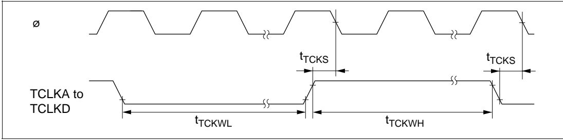
Figure 7.23 TPU Clock Input Timing
