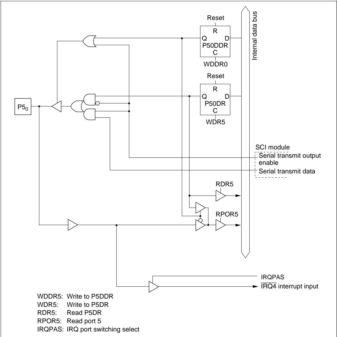
Figure 5.31 (a) Port 5 Block Diagram (Pin P5 0 )
