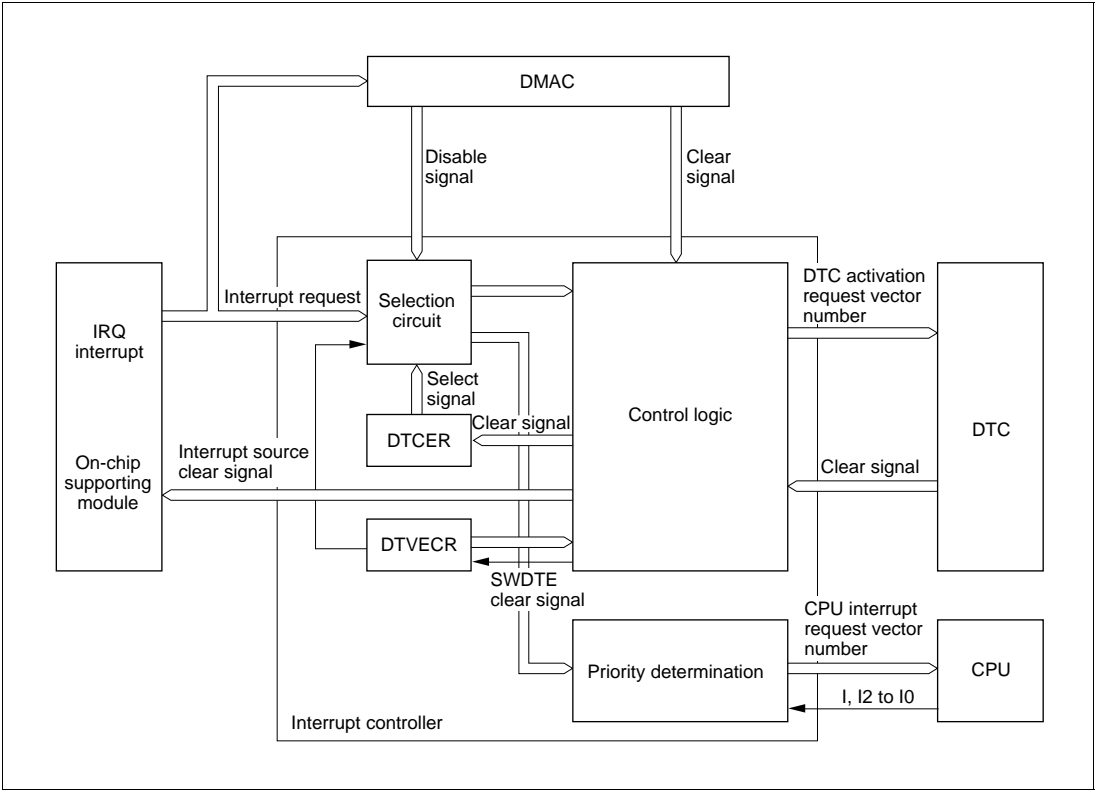
Figure 3.3 Interrupt Control for DTC and DMAC
