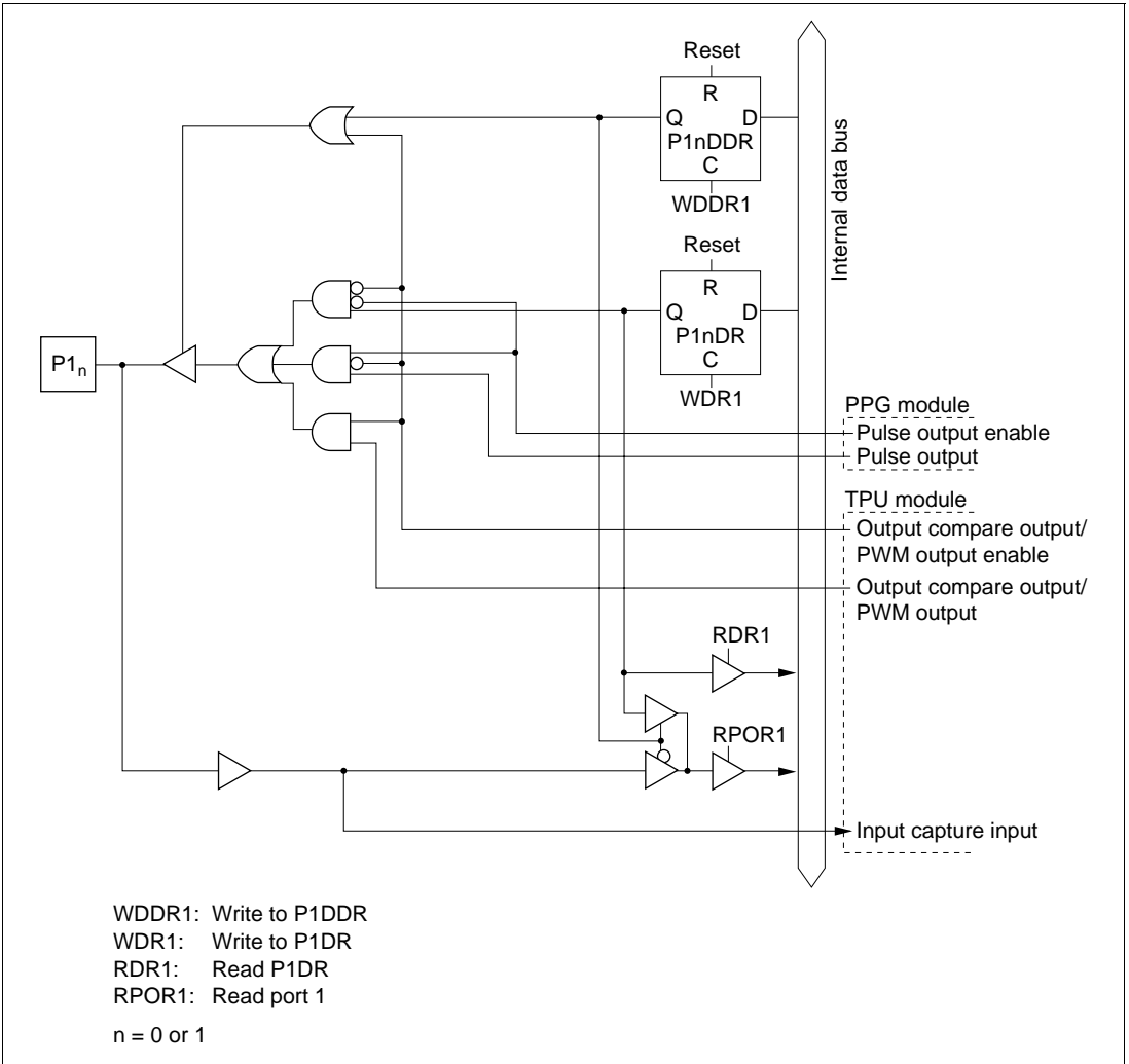
Figure 5.27 (a) Port 1 Block Diagram (Pins P1 0 and P1 1 )
