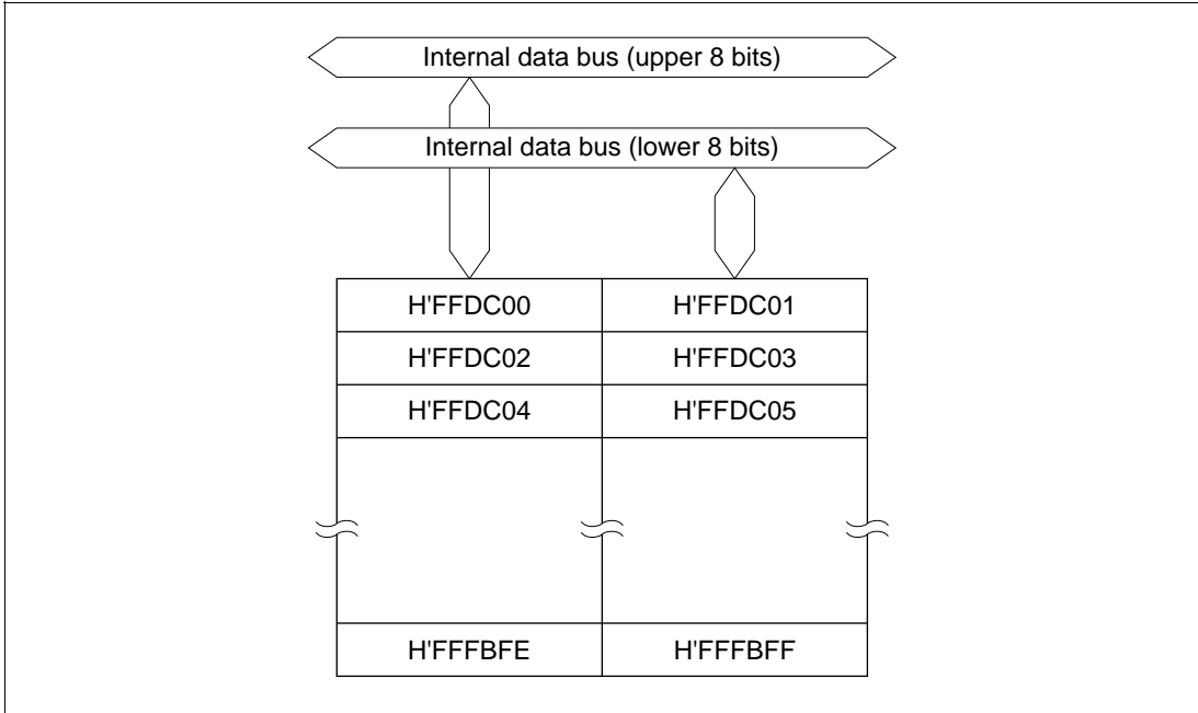
Figure 6.13 Block Diagram of RAM (8 kbytes)
