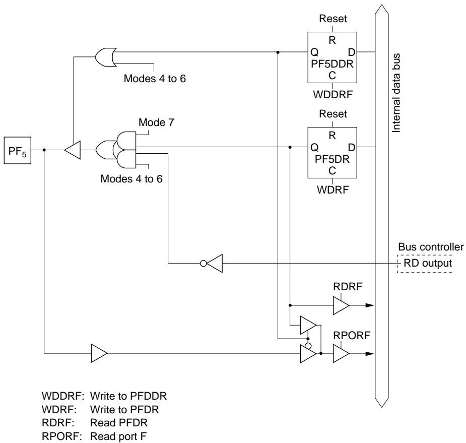
Figure 5.41 (f) Port F Block Diagram (Pin PF 5 )
