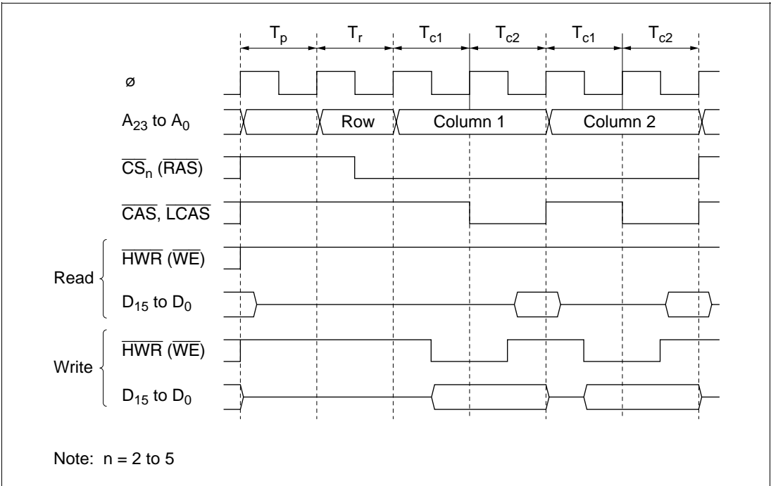
Figure 4.10 Operation Timing in Fast Page Mode
