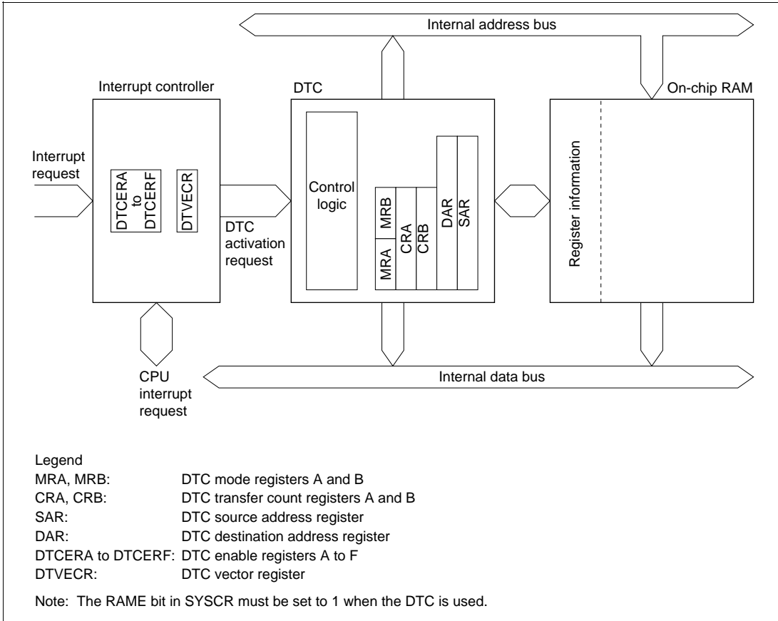
Figure 6.3 Block Diagram of DTC
