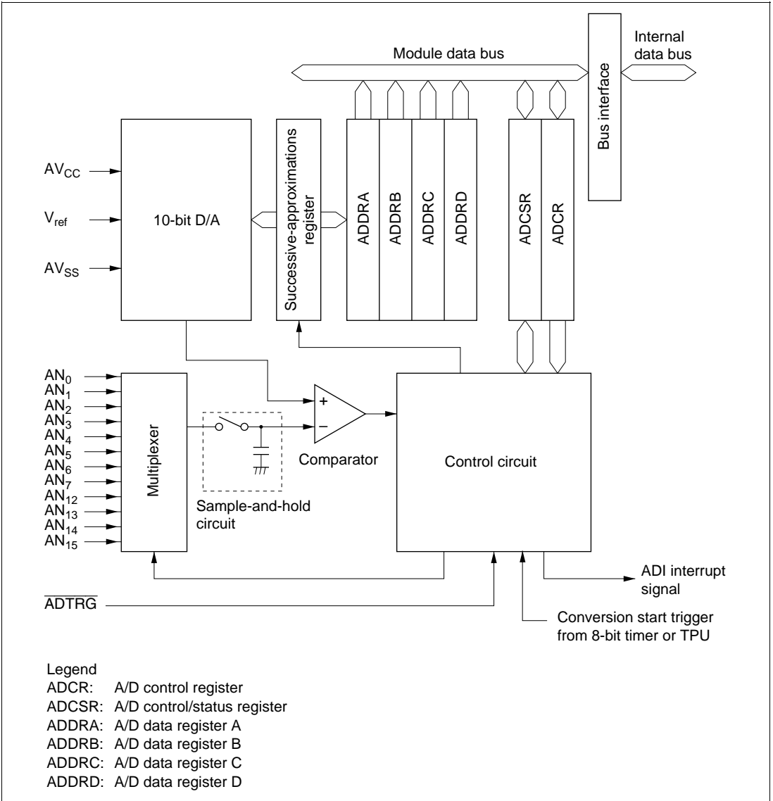
Figure 6.10 Block Diagram of A/D Converter
