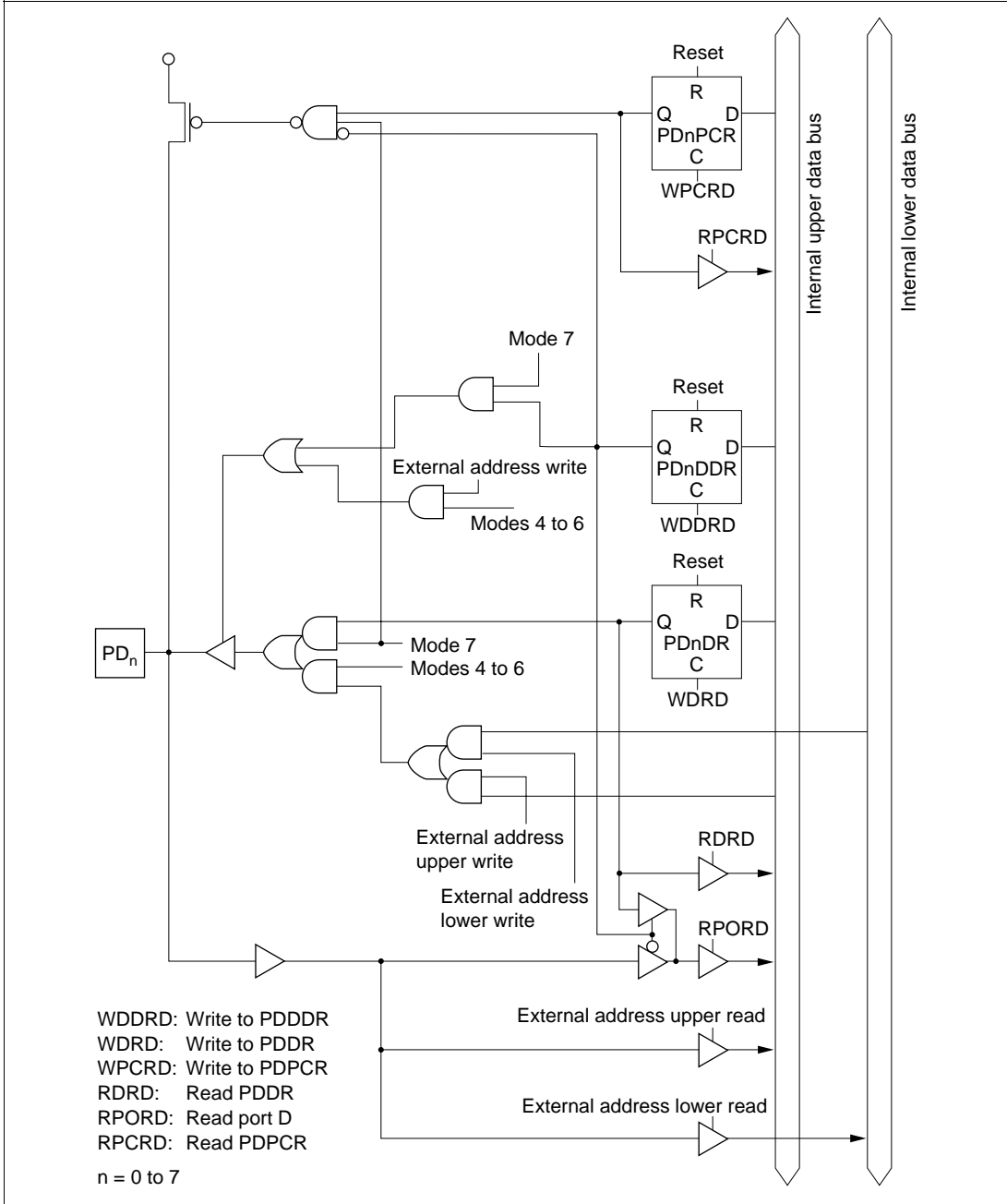
Figure 5.39 Port D Block Diagram (Pins PD n )
