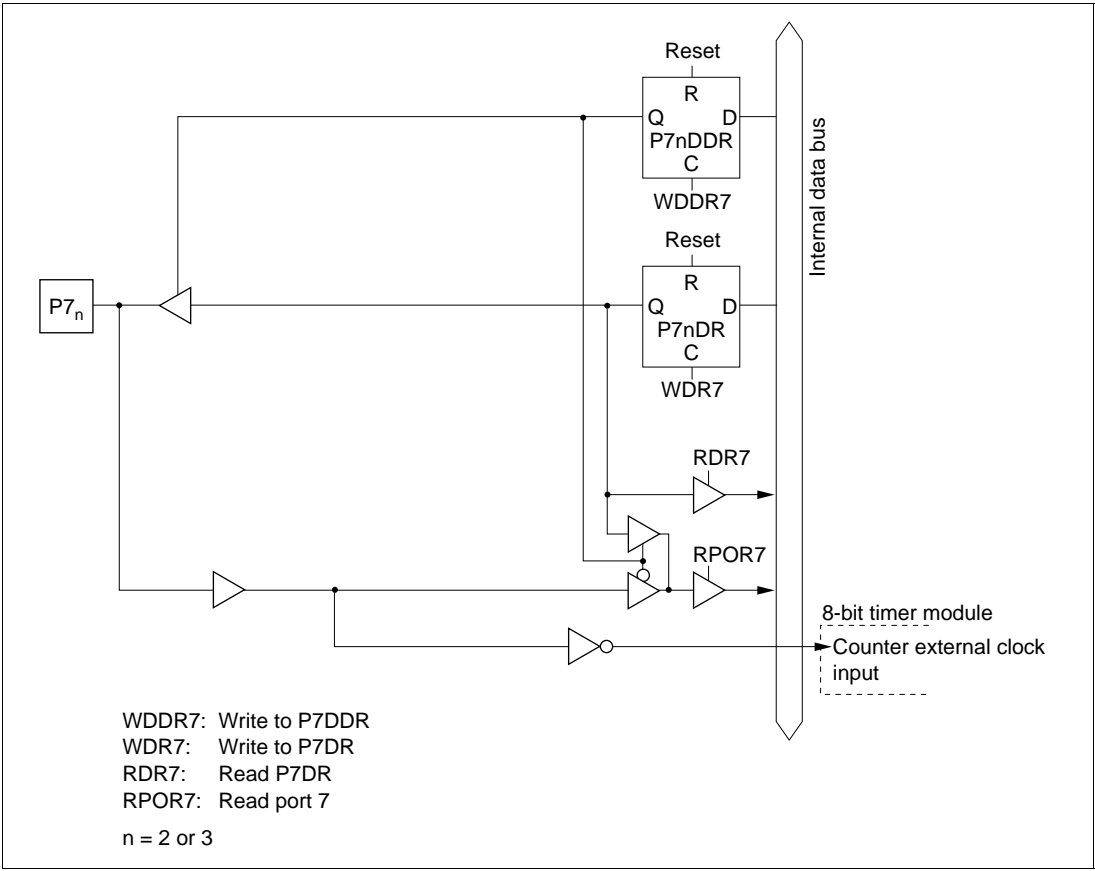
Figure 5.33 (b) Port 7 Block Diagram (Pins P7 2 and P7 3 )
