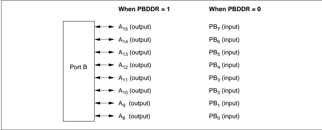
Figure 5.13 Port B Pin Functions (Mode 6)
