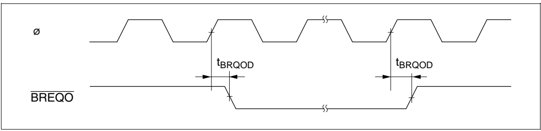
Figure 7.15 External Bus Request Output Timing
