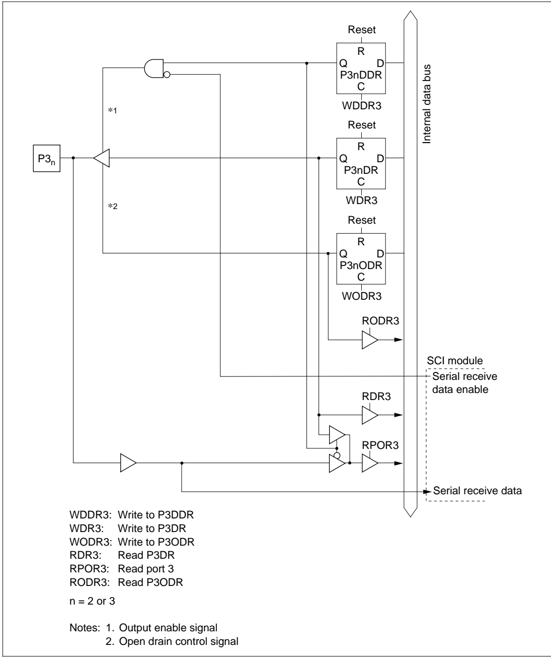
Figure 5.29 (b) Port 3 Block Diagram (Pins P3 2 and P3 3 )
