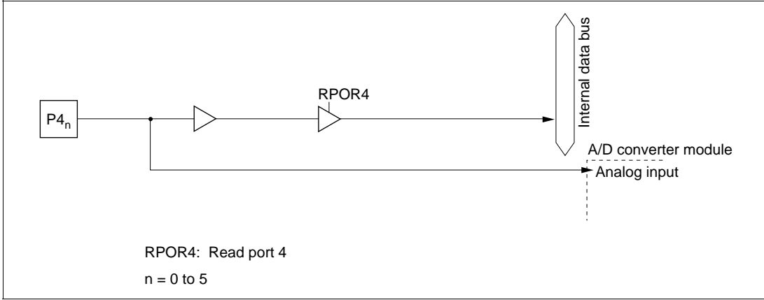
Figure 5.30 (a) Port 4 Block Diagram (Pins P4_0 to P4_5 )
