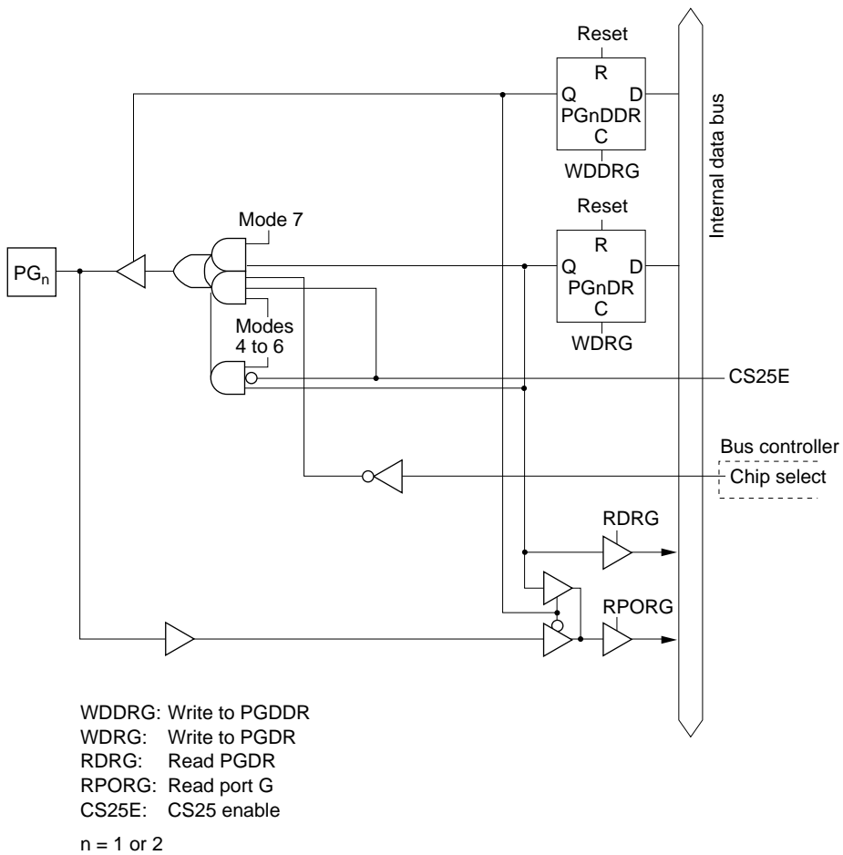
Figure 5.42 (b) Port G Block Diagram (Pins PG 1 and PG 2 )
