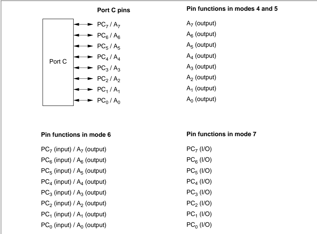
Figure 5.15 Port C Pin Functions
