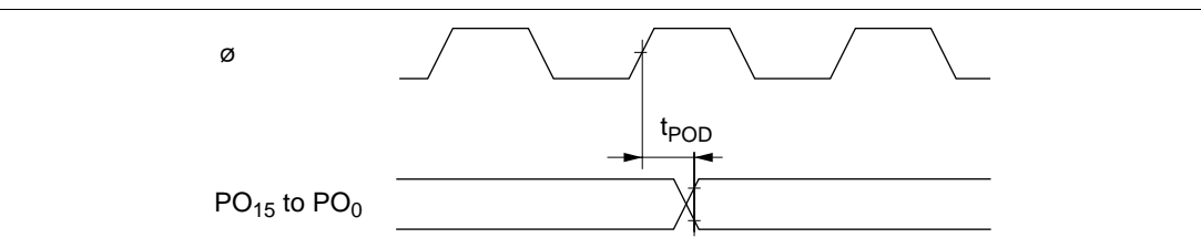
Figure 7.21 PPG Output Timing
