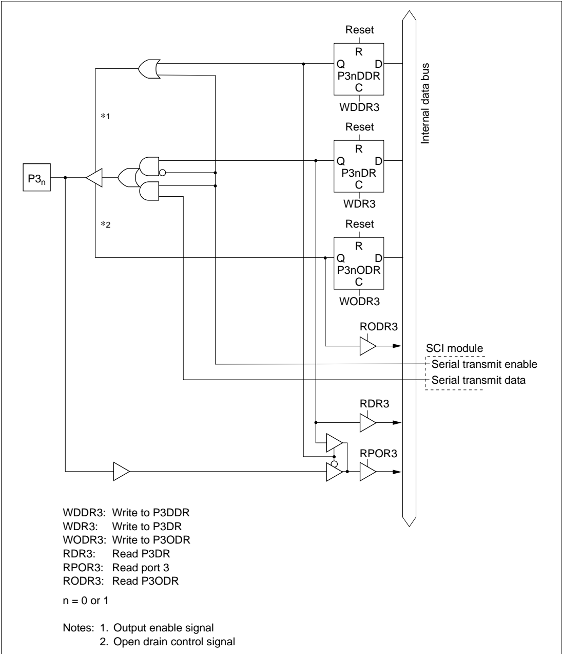
Figure 5.29 (a) Port 3 Block Diagram (Pins P3_0 and P3_1 )
