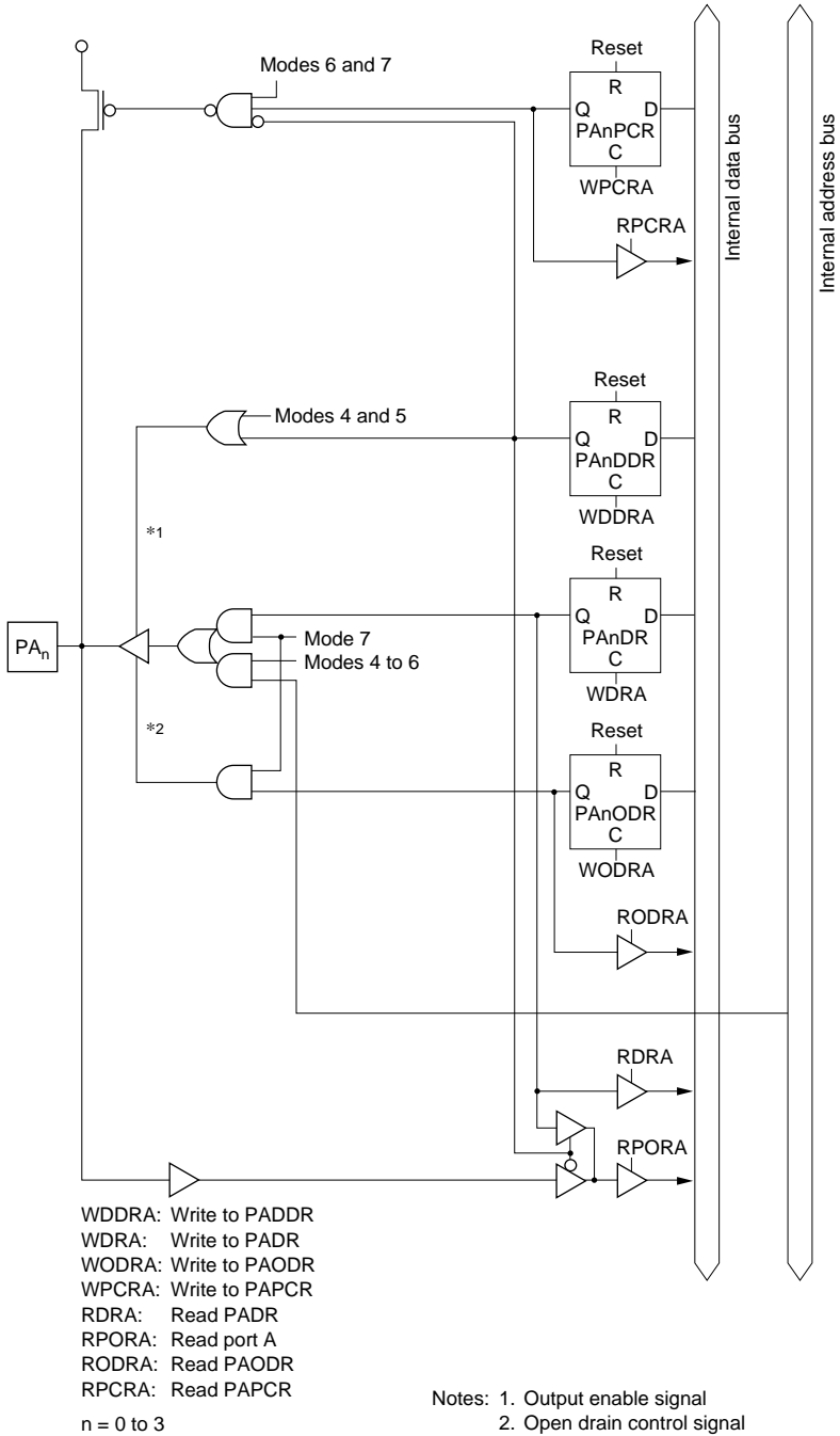
Figure 5.36 (a) Port A Block Diagram (Pins PA_0 , PA_1 , PA_2 , and PA_3 )
