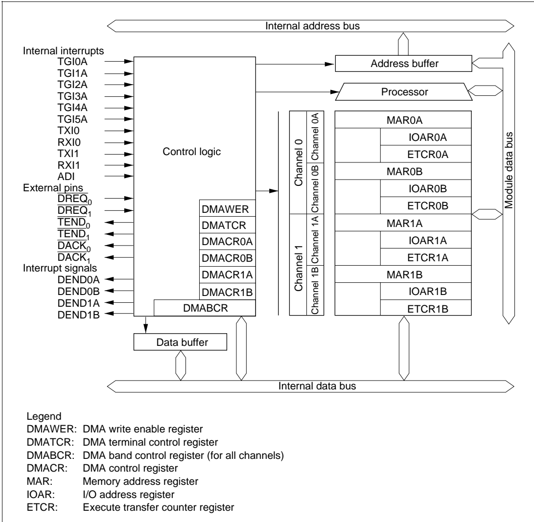
Figure 6.2 Block Diagram of DMAC
