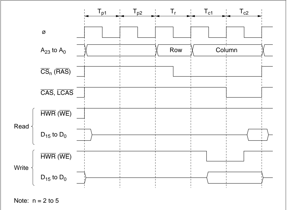
Figure 4.6 Timing with Two-State Precharge Cycle
