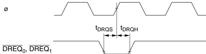
Figure 7.19 DMAC \overline{DREQ} Input Timing
