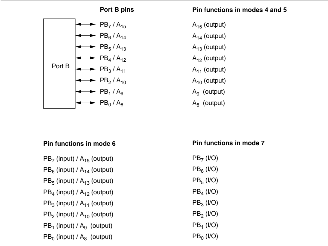
Figure 5.11 Port B Pin Functions
