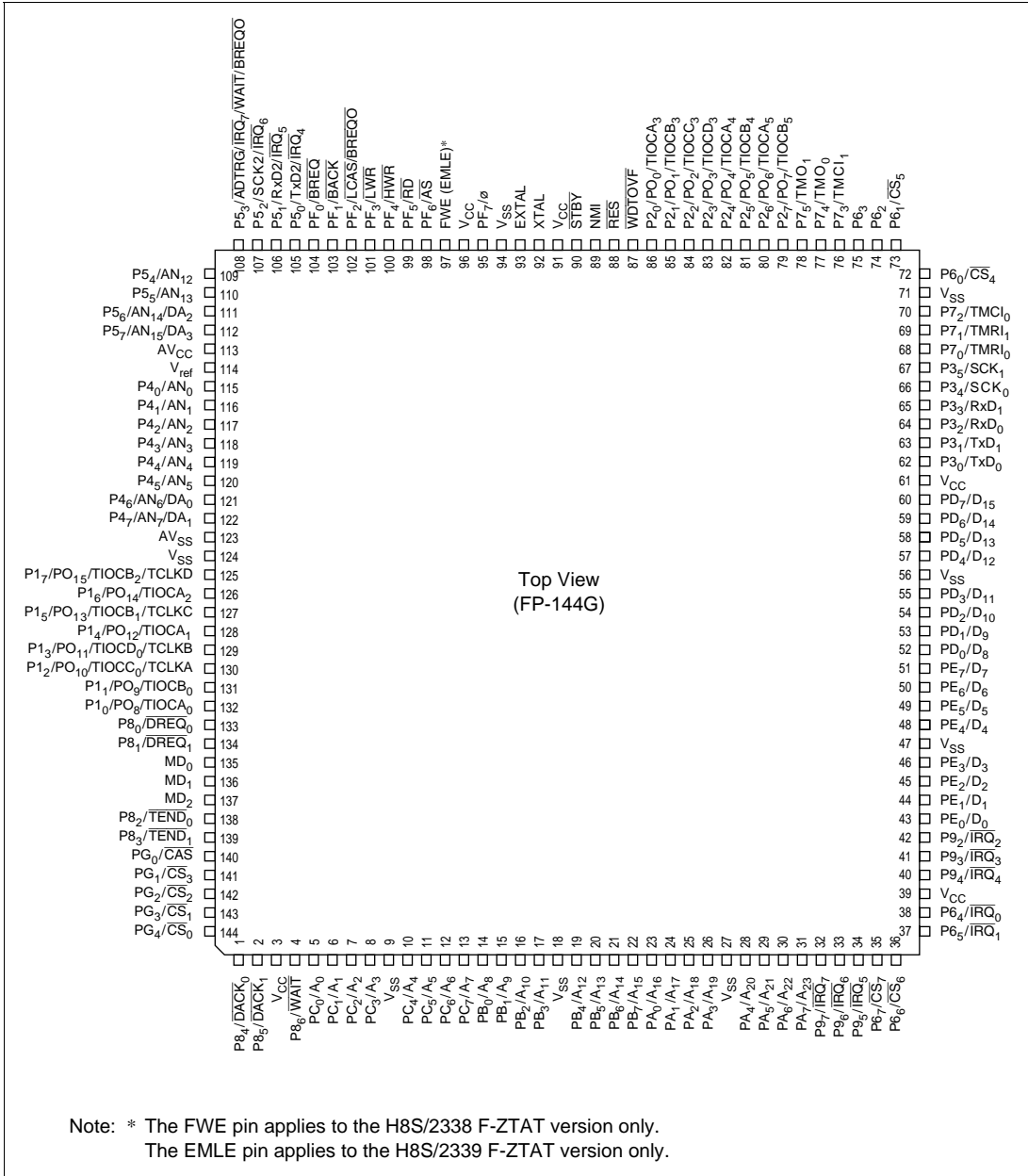
Figure 1.2 Pin Arrangement (TFP-144G: Top View)
