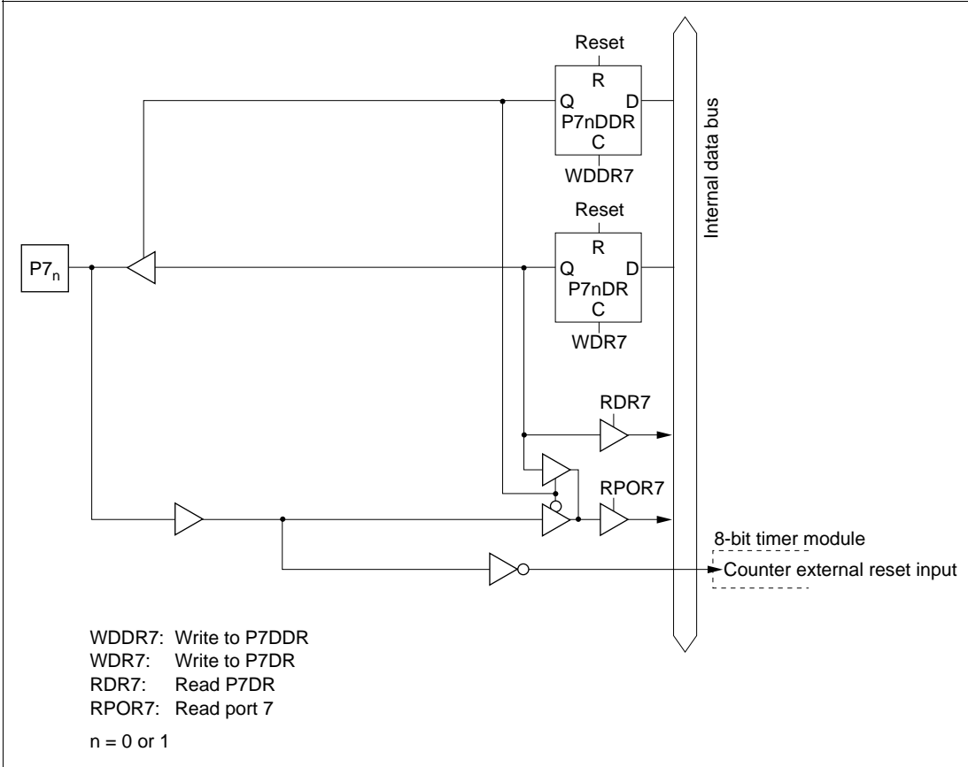
Figure 5.33 (a) Port 7 Block Diagram (Pins P7 0 and P7 1 )
