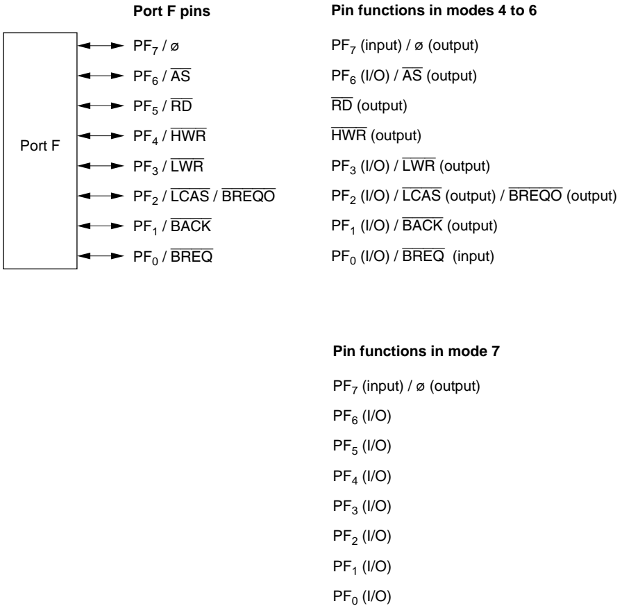
Figure 5.25 Port F Pin Functions
