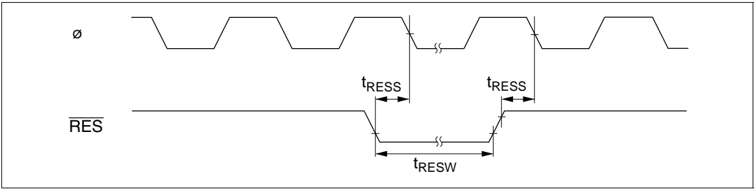
Figure 7.4 Reset Input Timing
