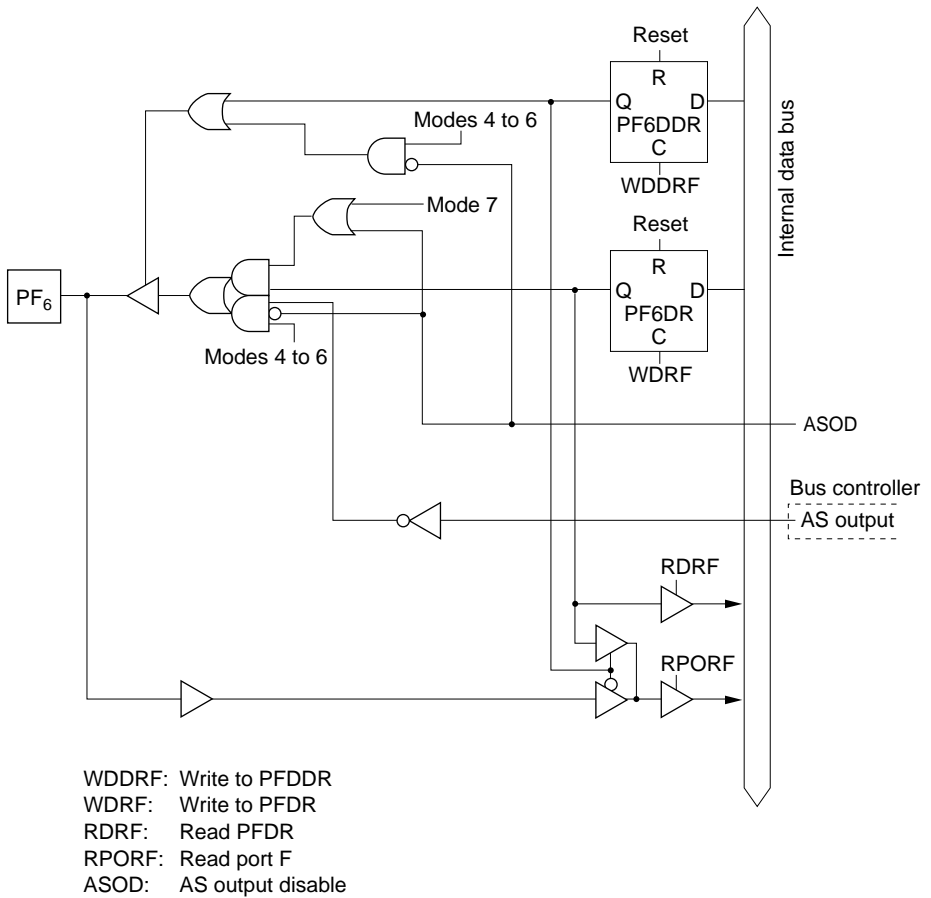
Figure 5.41 (g) Port F Block Diagram (Pin PF 6 )
