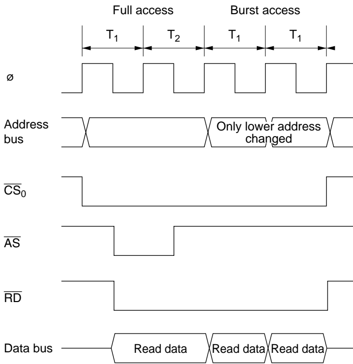
Figure 4.20 (b) Example of Burst ROM Access Timing (When AST0 = BRSTS1 = 0 )
