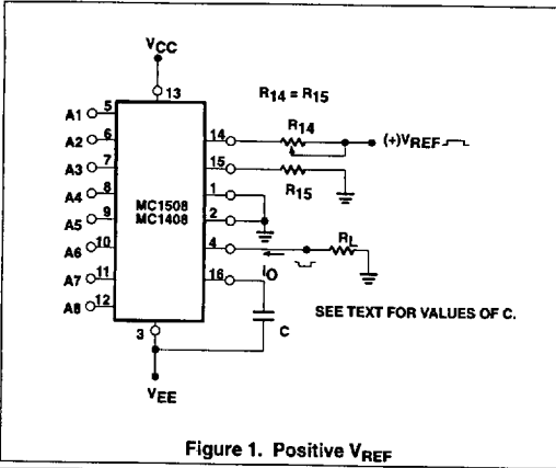
Figure 1. Positive V_{REF}
