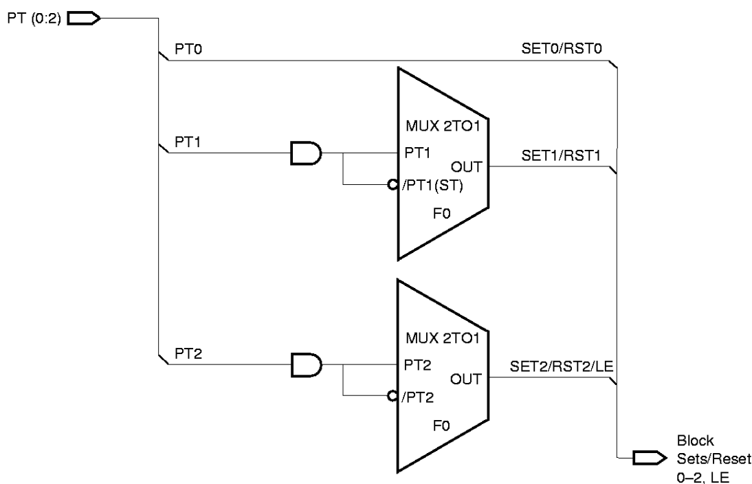
Figure 5. Set/Reset Generator
