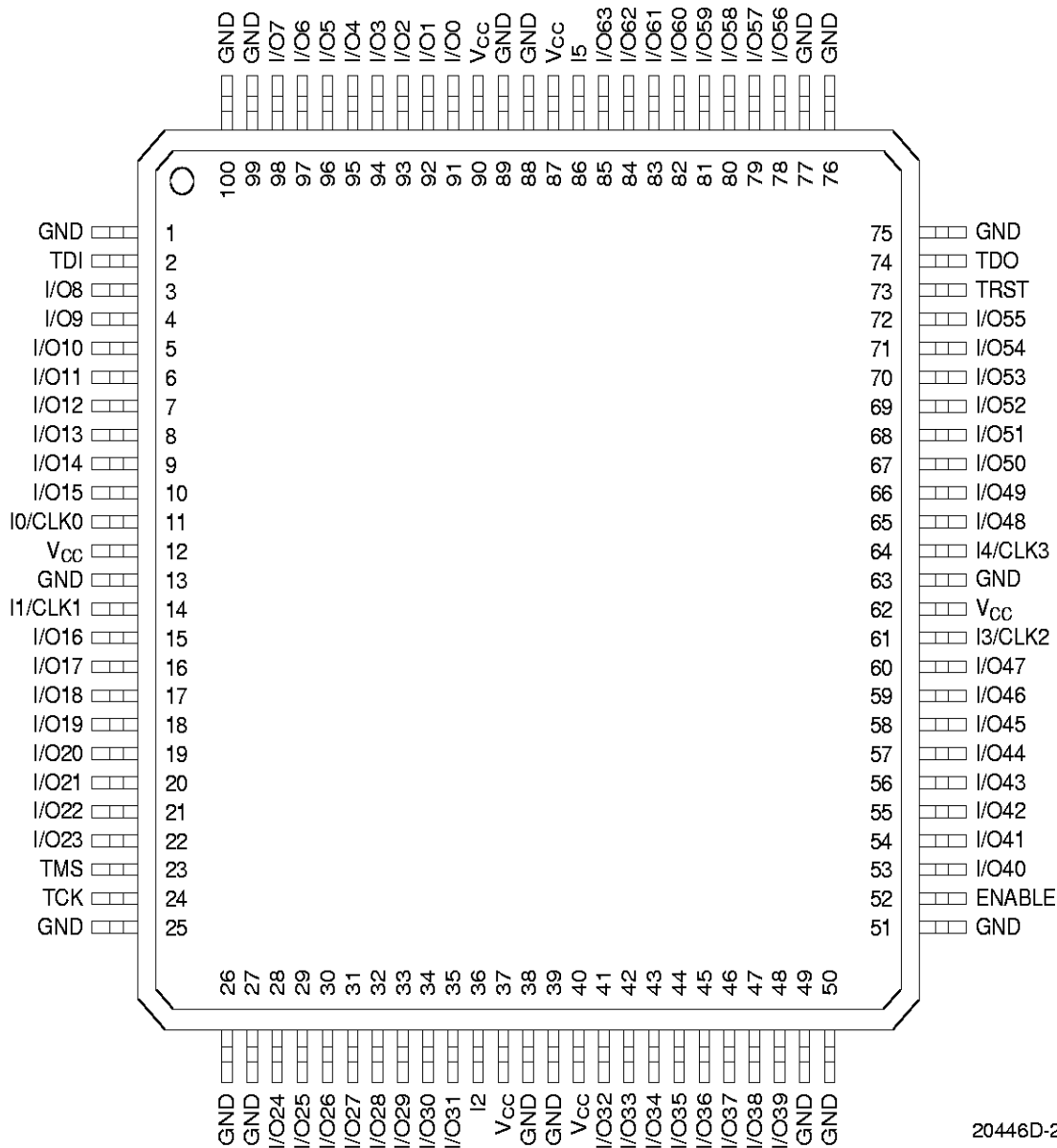
100-Pin TQFP
