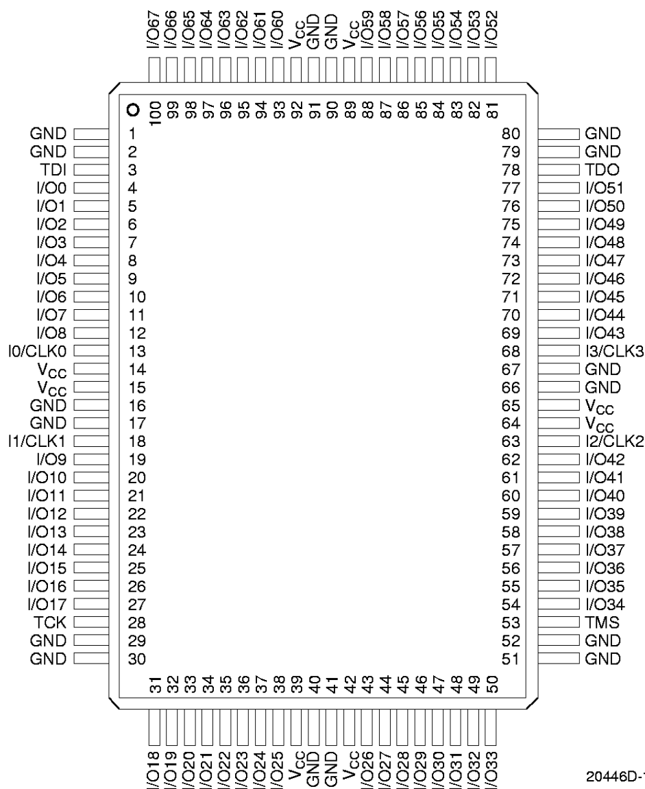
100-Pin PQFP
