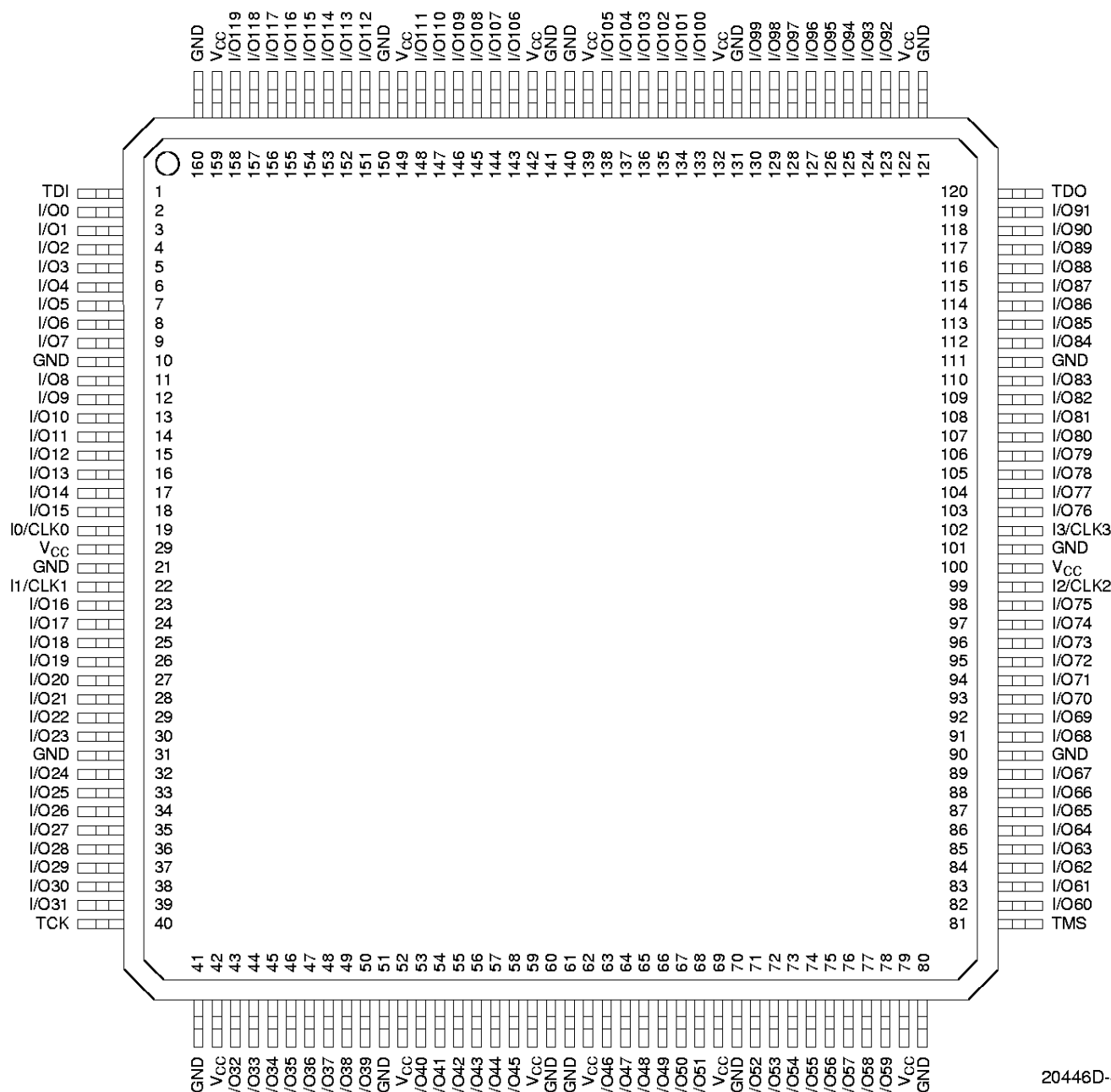
160-Pin PQFP
