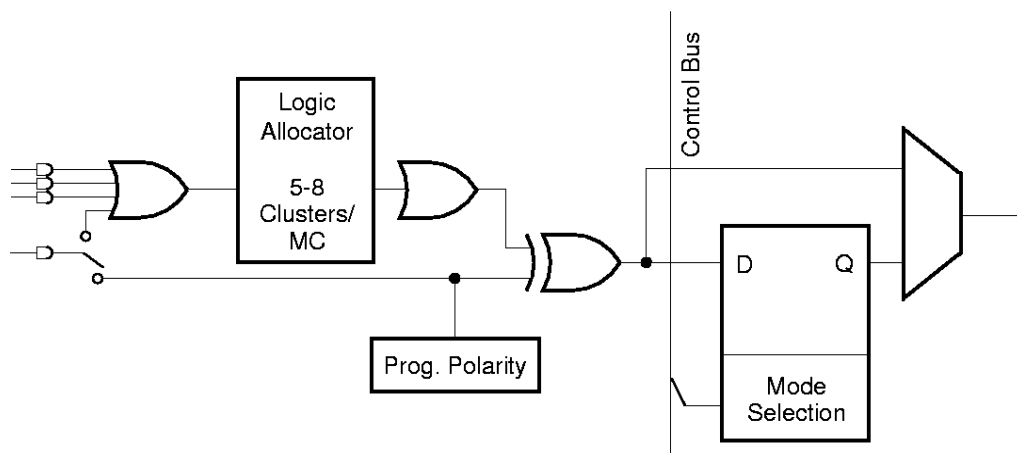
Figure 3. Macrocell Diagram
