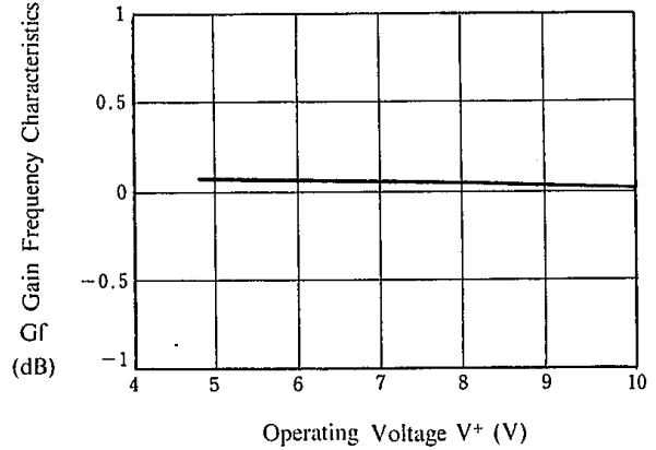
Gain Frequency Characteristics vs. Operating Voltage (Bias Type Input)
