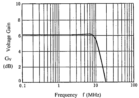
Voltage Gain vs. Frequency (Bias Type Input)
