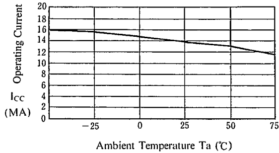
Operating Current vs. T_a ( V^+ = 5\text{ V} )
