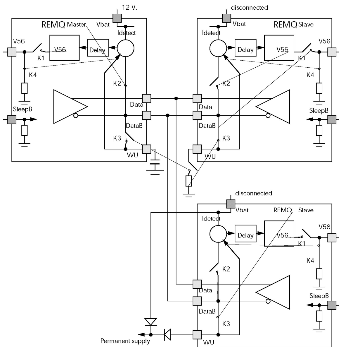
Fig. 6: System Configuration in Sleep Mode
