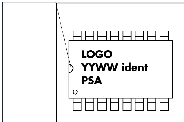
Fig. 11: Topside Marking
