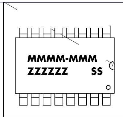
Fig. 12: Backside Marking
