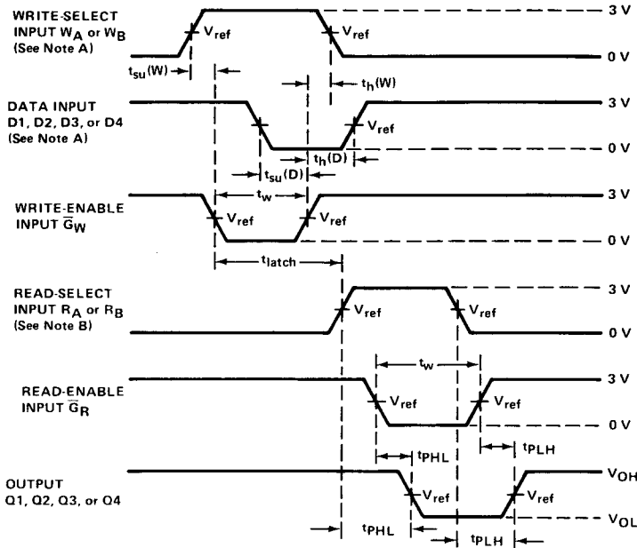
VOLTAGE WAVEFORMS
