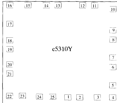
Figure 6. Pad layout of the e5310 chip
