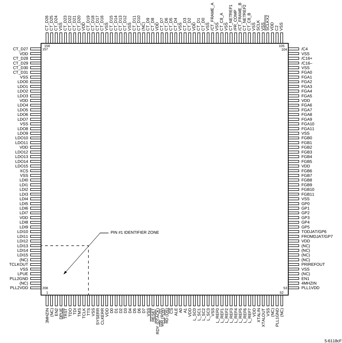
Figure 1. 208 SQFP—Top View
