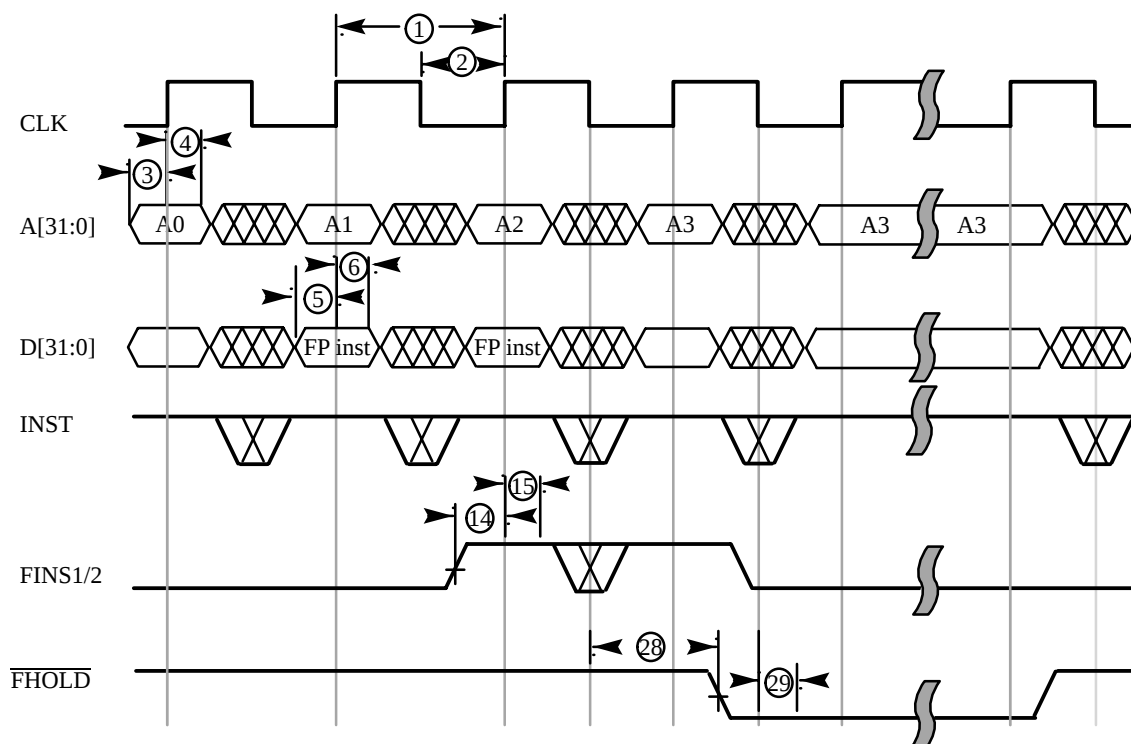
Figure 25. Floating-Point \overline{\text{FHOLD}} Assertion
