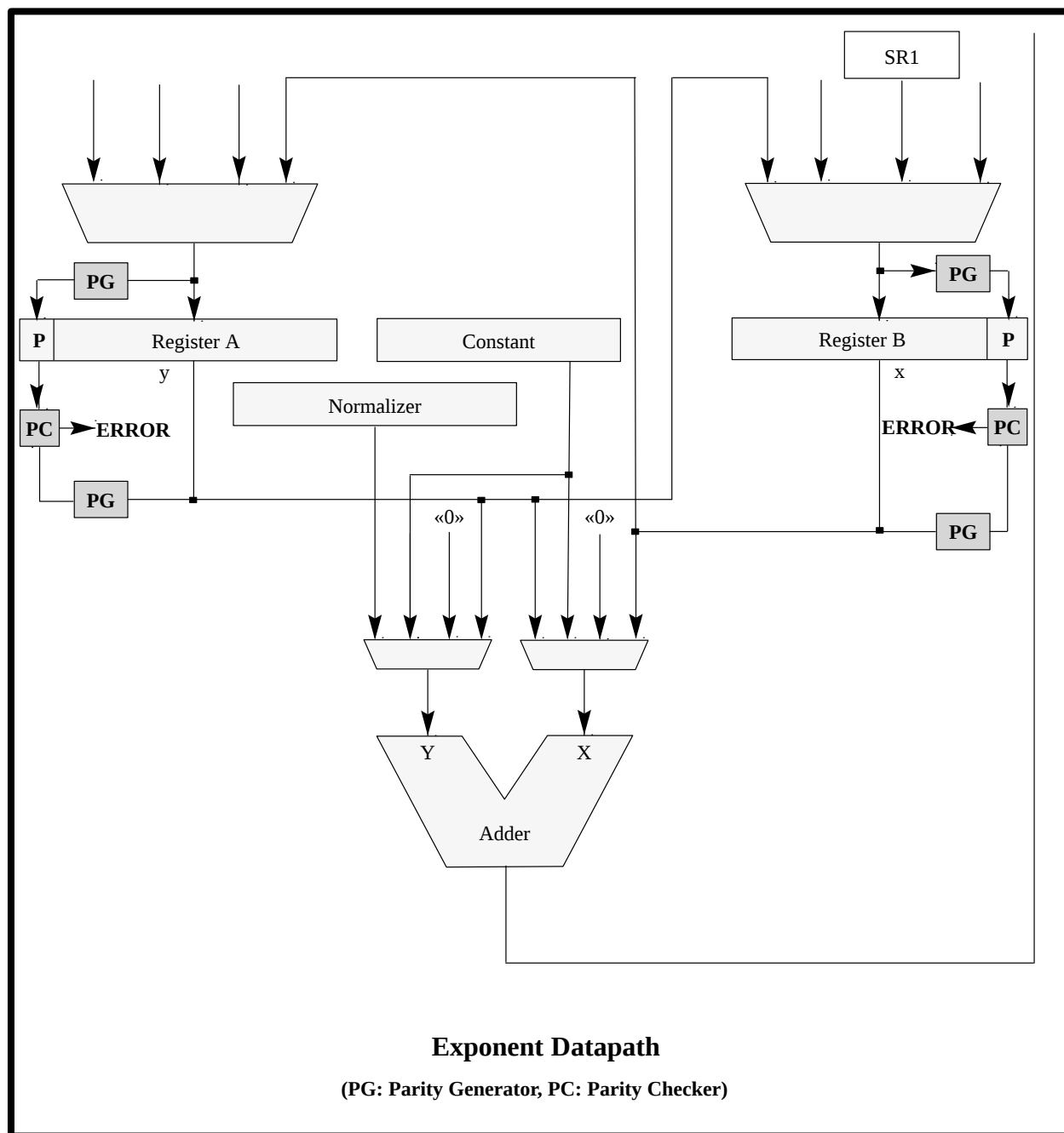
Figure 20. Parity Checking on Exponent Datapath
