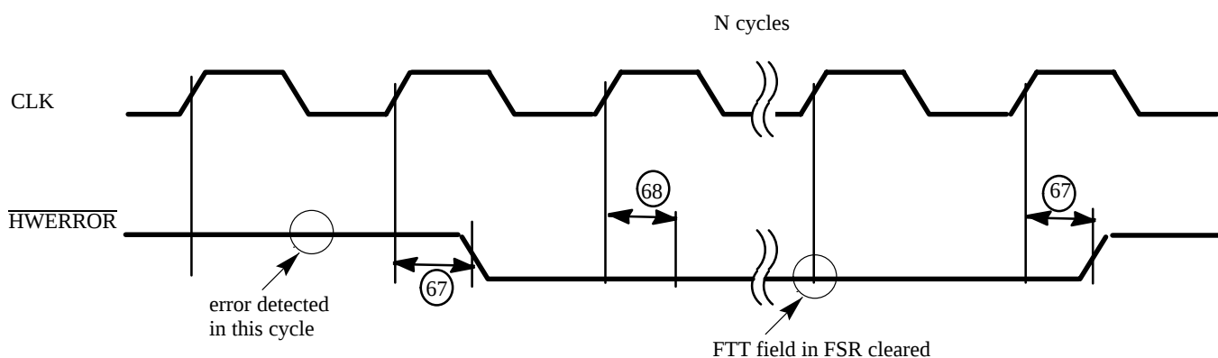
Figure 35. HWERROR Timing
