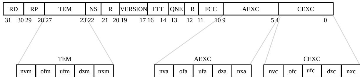
Figure 14. Floating-Point Status Register
