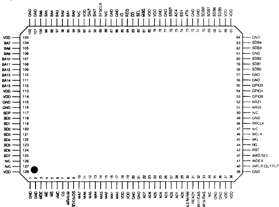
128-Lead QFP, TQFP
