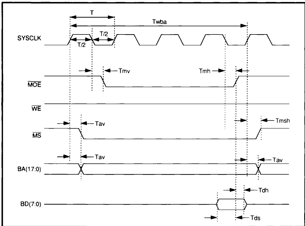
FIGURE 8: SRAM Read Timing
