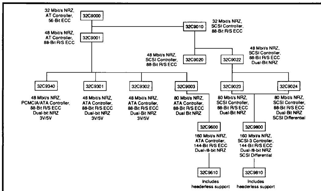
FIGURE 1: Silicon Systems' Single Chip Controller Hierarchy
