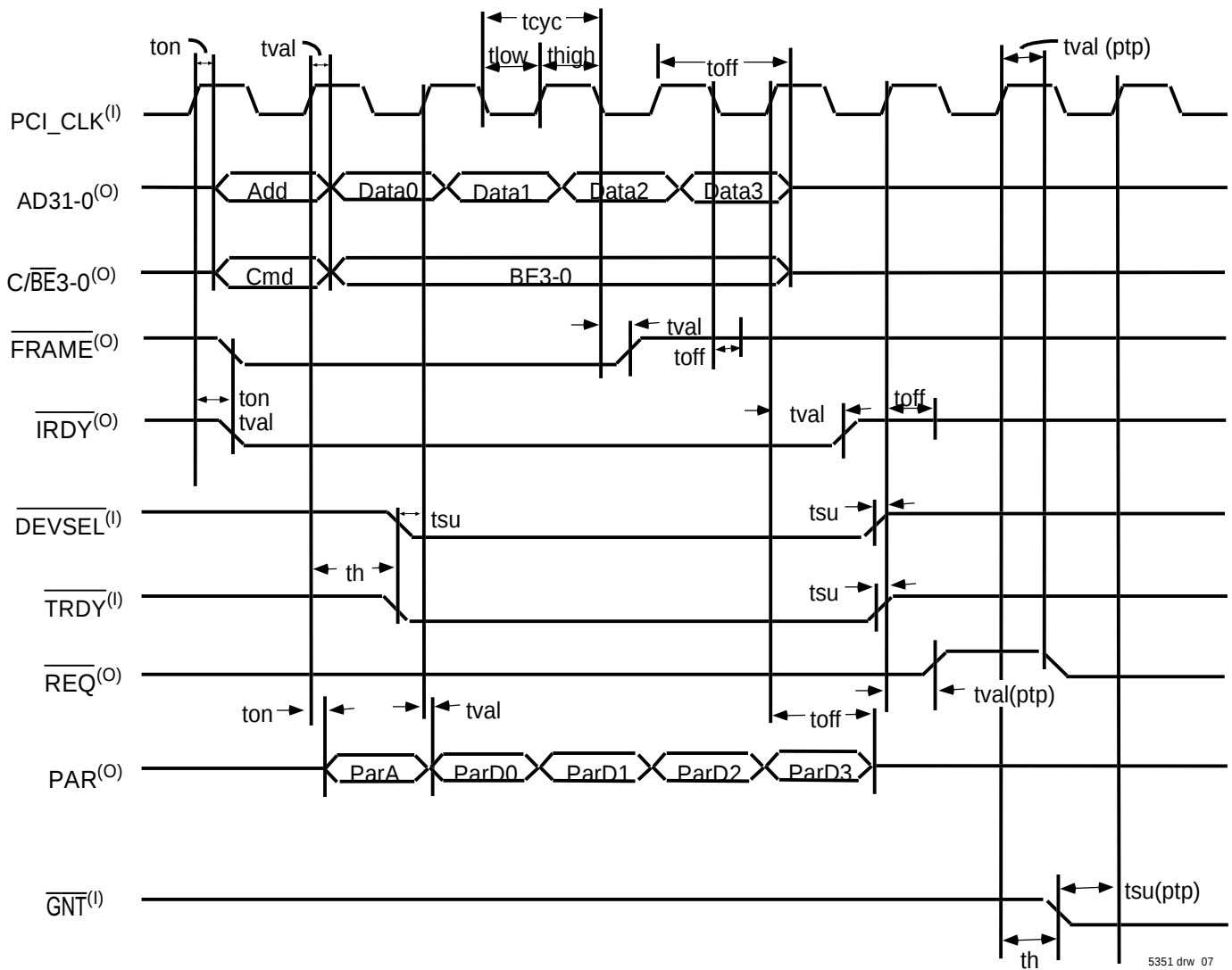
Figure 1. The IDT77V222 as a PCI master (illustrates a 4-word write by the IDT77V222 to host memory)
