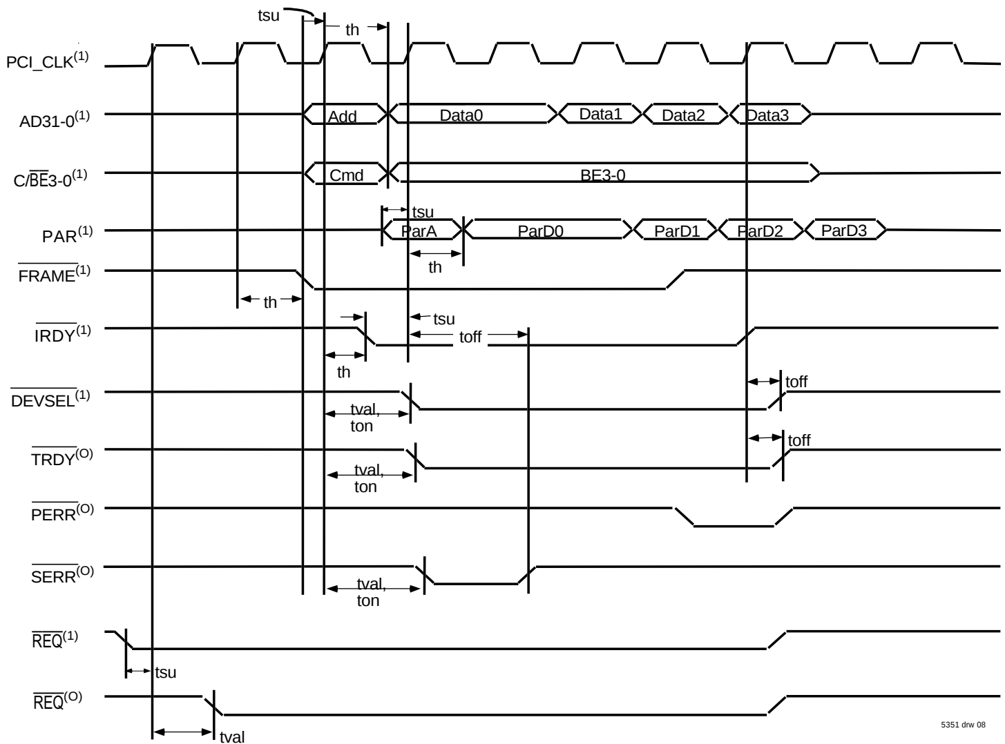
Figure 2. The IDT77V222 as a PCI target (illustrates a 4-word write operation by the host device driver to the IDT77V222 )
