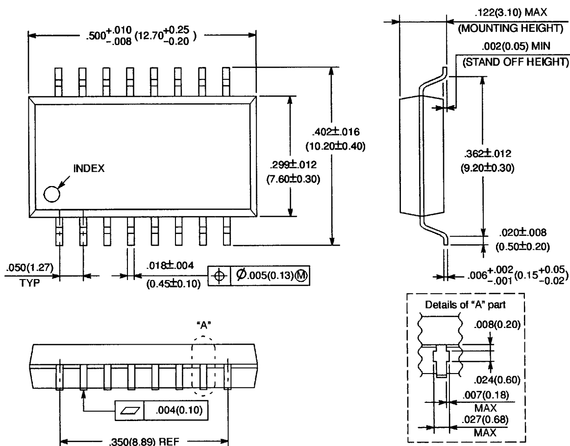
16-LEAD PLASTIC FLAT PACKAGE (CASE No.: FPT-16P-M03)
