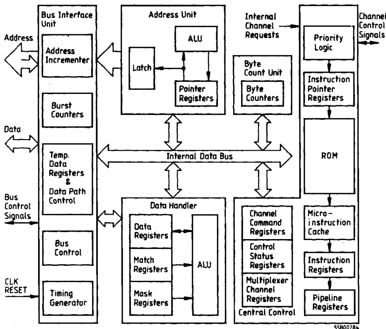
Block Diagram of the SAB 82258A
