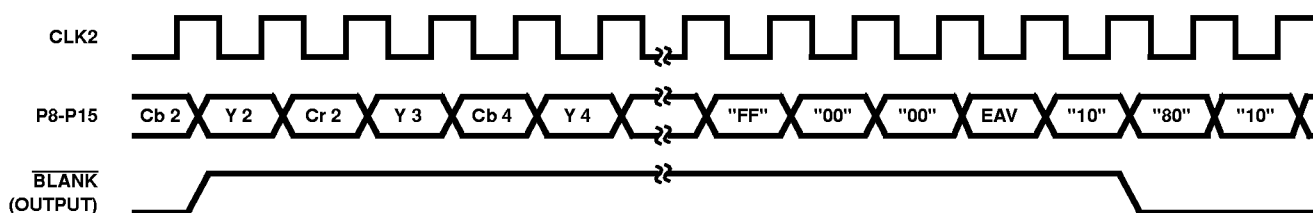
FIGURE 3. PIXEL INPUT TIMING - BT.656
